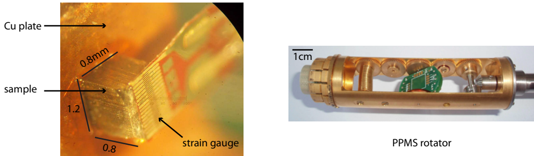
Figure 2.13: Picture of a strain gauge stucken on a sample of URhSi. The setup is mounted on a PPMS rotator.
