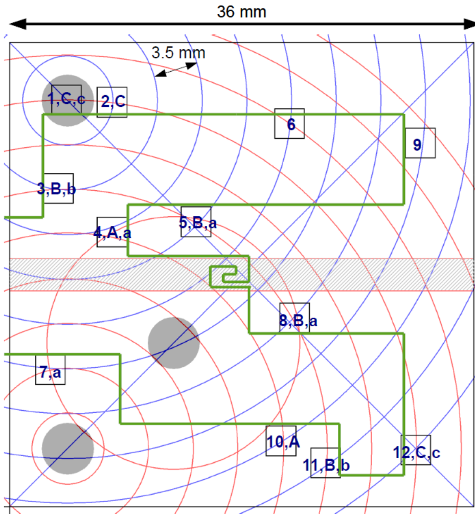
Figure 8.25: Schematic representation of the pixels positions on the new SPK-2 arrays. The grey circles represent the different possible impact points. In green, a sketch of the approximate route of the feedline. The SPK-2 mask contains two copies of the same array, one with the ground-plane present on the whole surface of the frontside, the second with a bare silicon frontside and the ground-plane only around the central conductor of the feedline.
