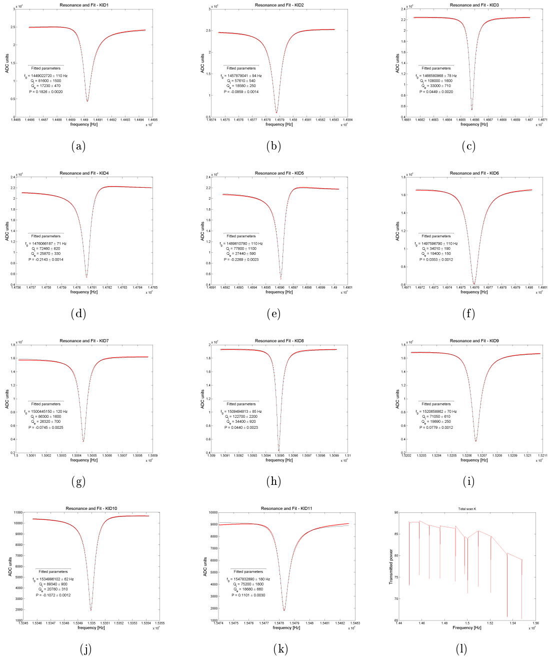
Figure 8.14: All the active resonances (data and fits) of the SPK-D array fabricated on HR-Si, with the additional backside titanium layer.
