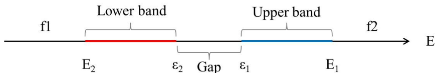
Figure II.3 – Schematic illustration of the different energy regions in which the retarded Green's function takes different expressions. The exact values of the band edges depending on the TB parameters of the FI are detailed in Appendix B.
