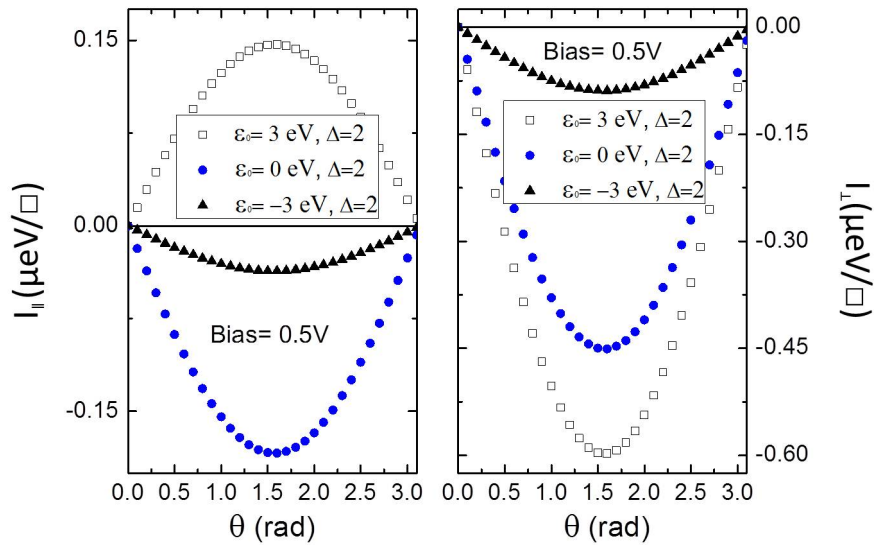
Figure III.5 – (Left) Angular dependence of the in-plane spin current density component for three different 3-D AF/B/AF MTJ with a bias of 0.5V and a barrier height U_B of 9 eV. (Right) Idem for the out-of-plane component.
