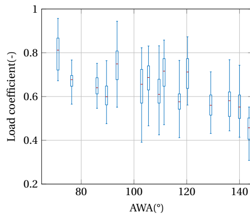
(a) Head load coefficient
