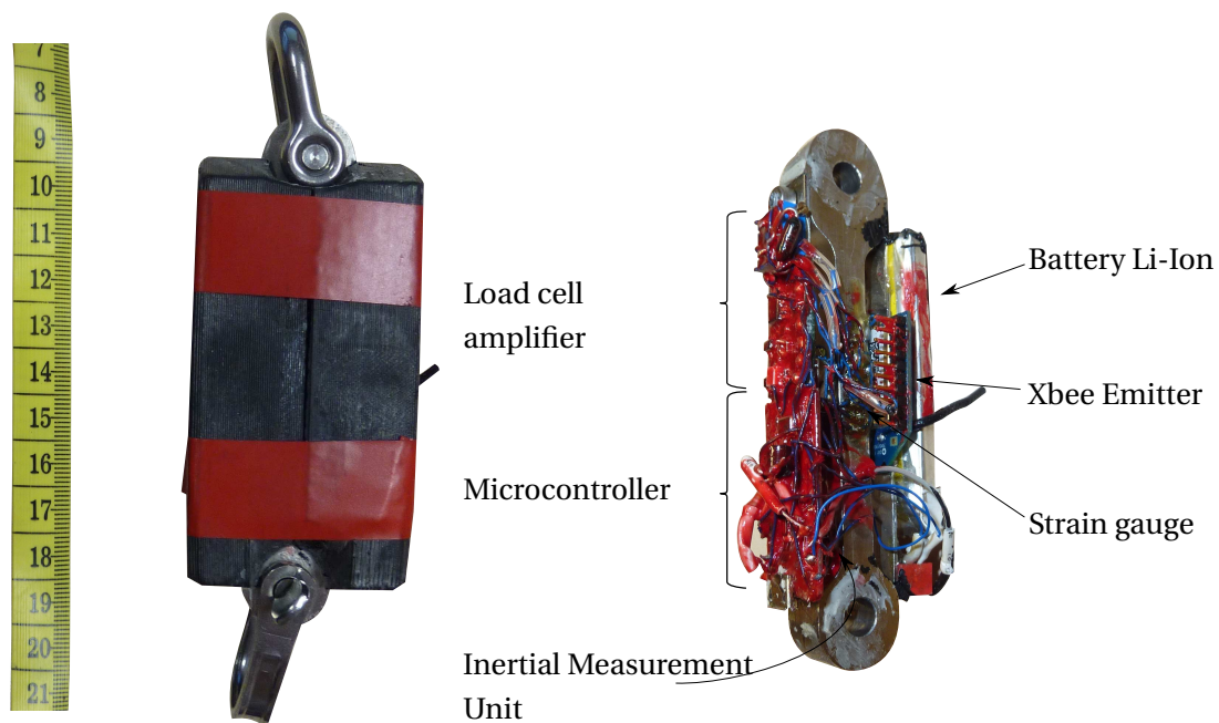
Figure 2.16 – Directional Load Cell (DLC) with its case and shackles (left), inside view (right).
