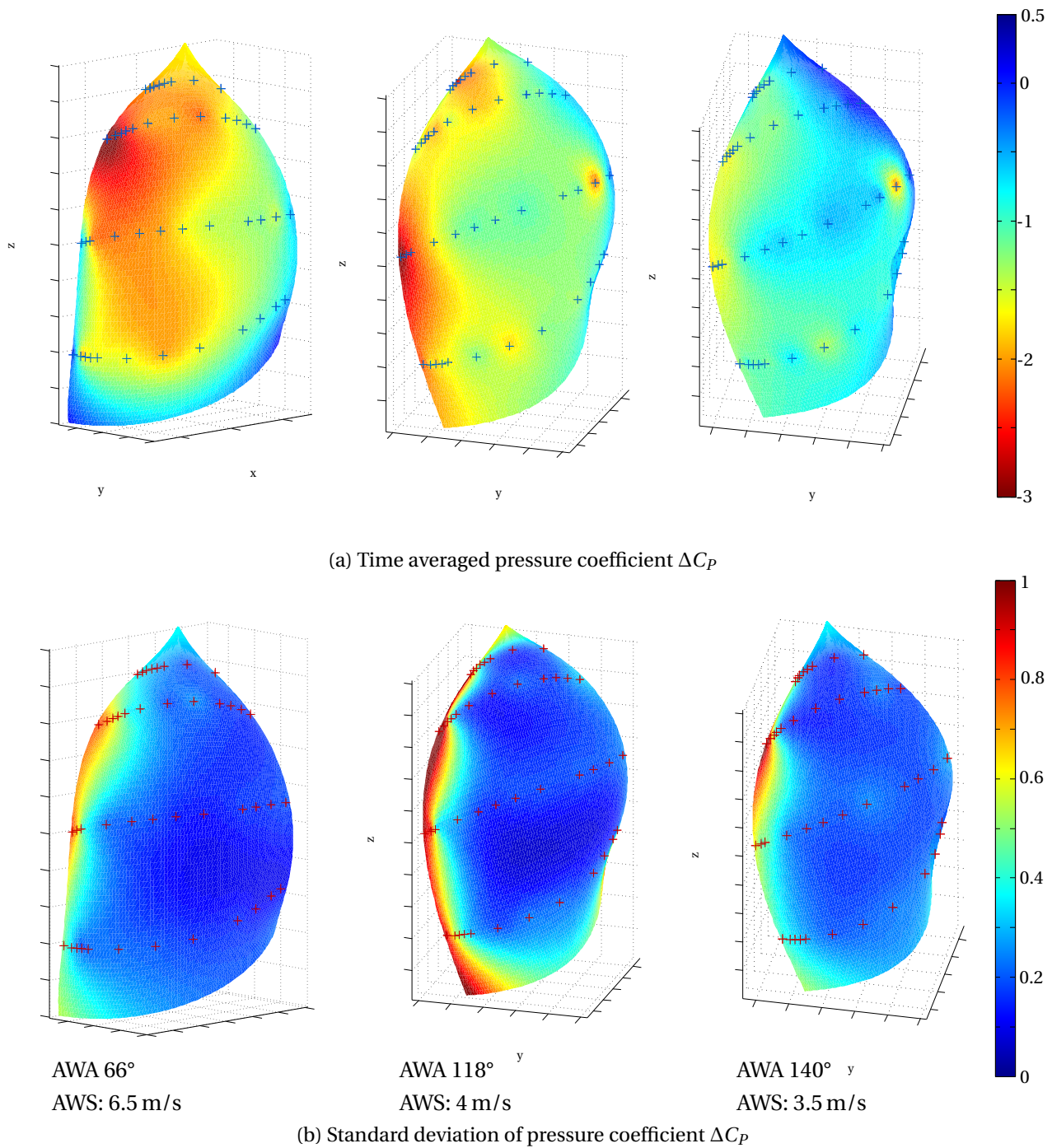
Figure 3.28 – Pressure distributions interpolated and extrapolated on referenced flying shapes for 3 typical AWA (66°, 118°, 140°). Time averaged pressure coefficient \Delta C_p (a) and the fluctuations represented by the standard deviations (b). The crosses (in blue in (a) and in red in (b)) indicate the positions of the pressure taps.
