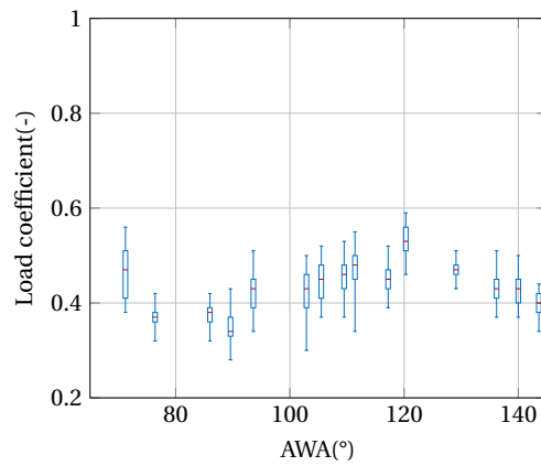
(c) Clew load coefficient
