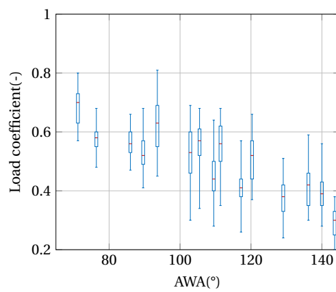
(b) Tack load coefficient
