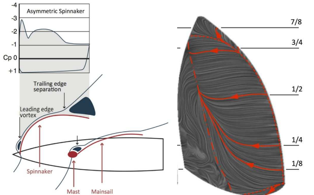
(a) Typical flow and pressure distributions in down-wind conditions.
