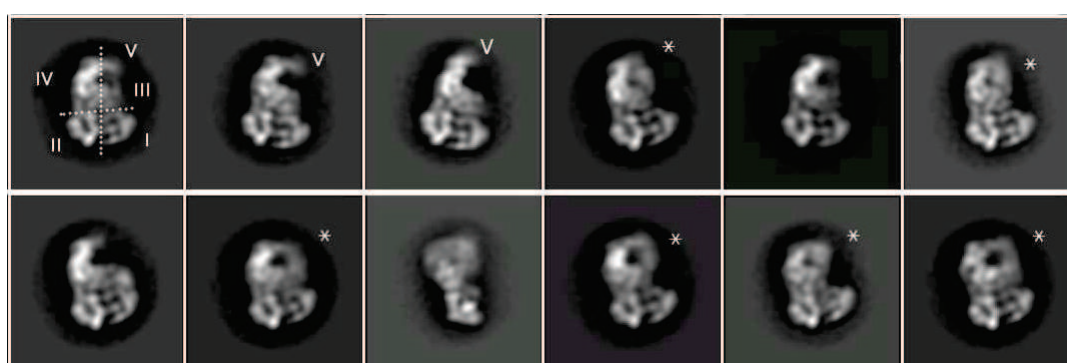
Fig. 61. Some representative 2D class averages of the SAGA complex.
