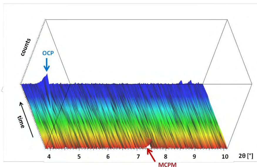
Figure A.b.2: Evolution during time (0-14d) of phases at the surface of DCPD samples after immersion in PBS. Range 2\theta = 4^\circ\text{-}10^\circ
