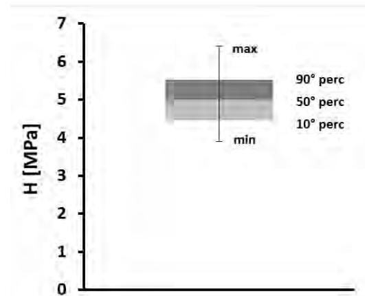
Figure 5: Distribution of hardness values obtained at the surface for all \beta -TCP samples at t_0
