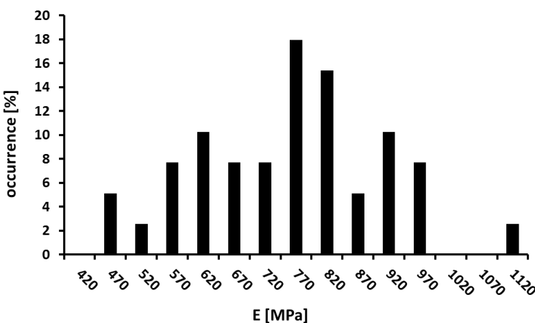
Figure 6: Distribution of values of Young's Modulus obtained at the surface for all \beta -TCP samples at t_0
