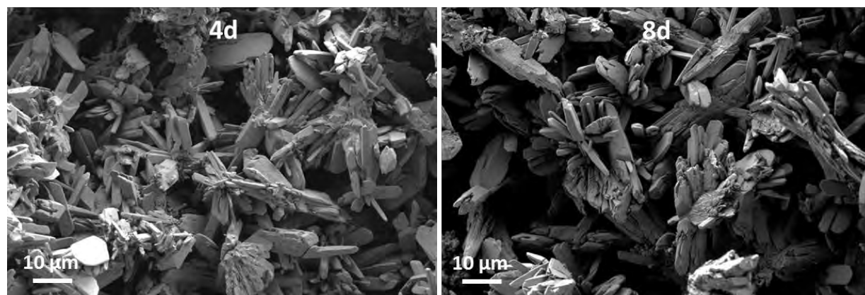
Figure A.b.12: SEM micrographs of the core of DCPD samples after immersion in PBSd for 4 and 8 days
