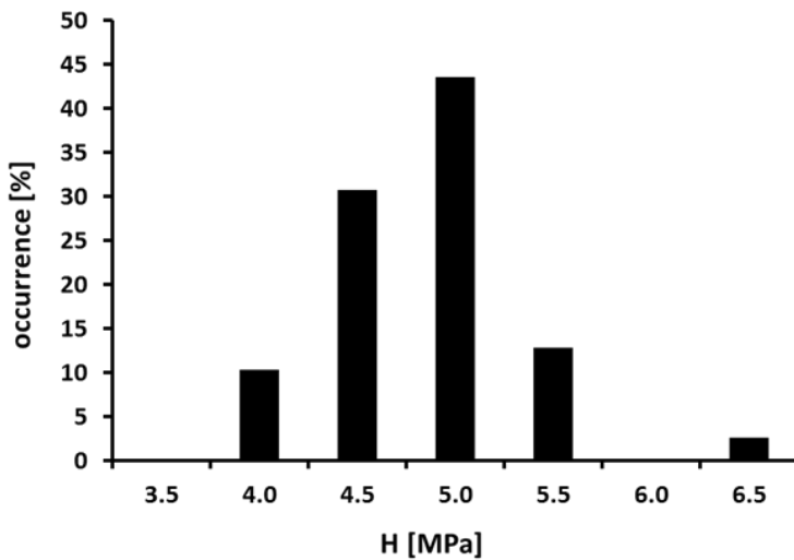
Figure 5: Distribution of hardness values obtained at the surface for all \beta -TCP samples at t_0
