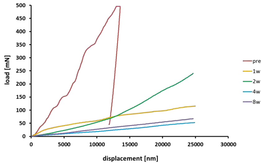
Figure 36: Representative load-displacement curves obtained at the surface of \beta -TCP samples after immersion in TRISd
