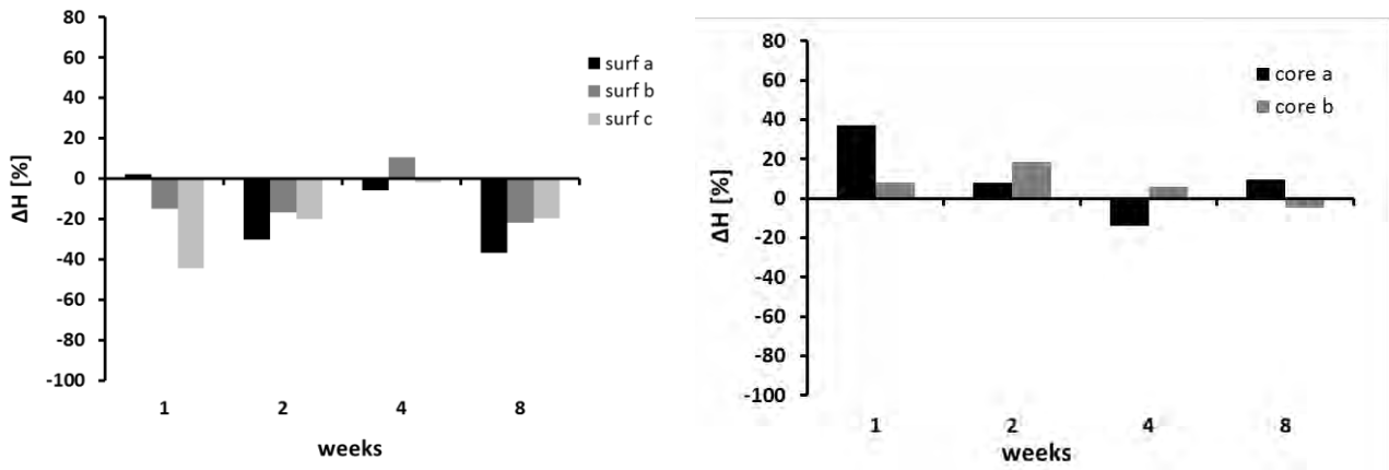
Figure A.c.5: Variation of hardness of \beta -TCP samples at the surface (left) and in the core (right) after different times of immersion in PBSd. Average values at t_0 : H_{surface}=5.0MPa , E_{surface}=788MPa , H_{core}=3.8MPa , E_{core}=986MPa
