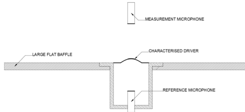
Figure 9: Schematic setup of space function measurement in an anechoic room.
