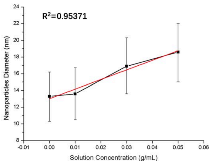
Fig. 3-6 Relation between solution concentration and NPs diameter
