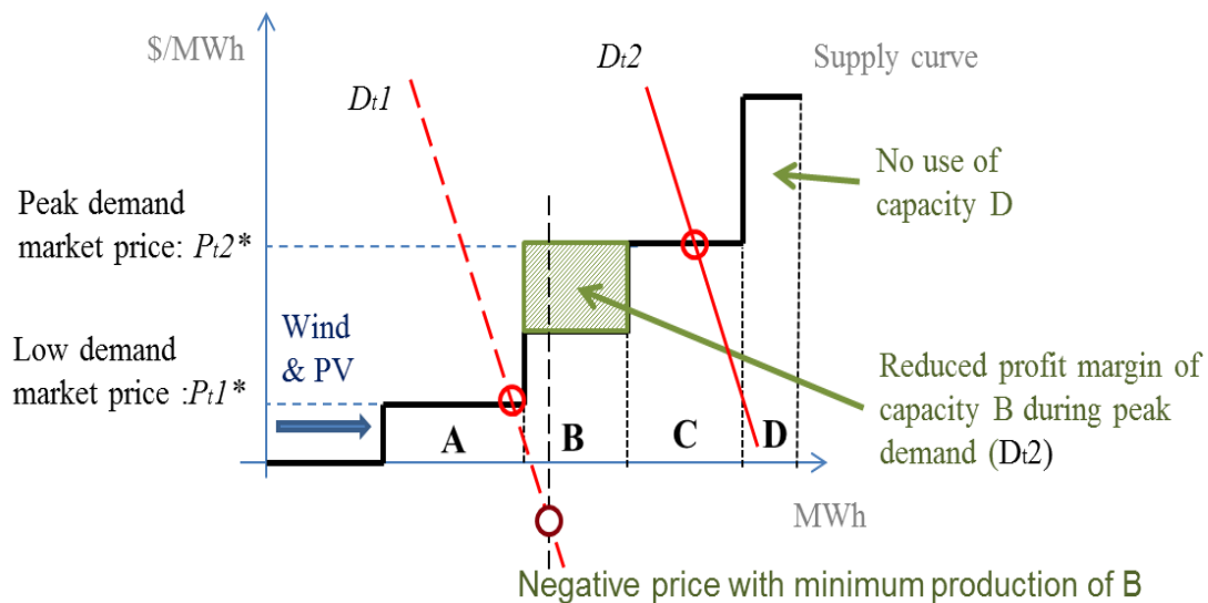
Figure 34: Merit order shifts with the integration of intermittent power (e.g. PV)
