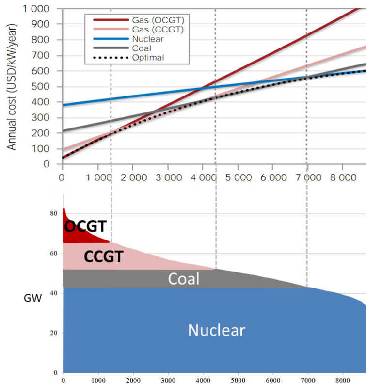
Figure 30: Example of optimal mix based on load duration curve (OECD/NEA, 2012)
