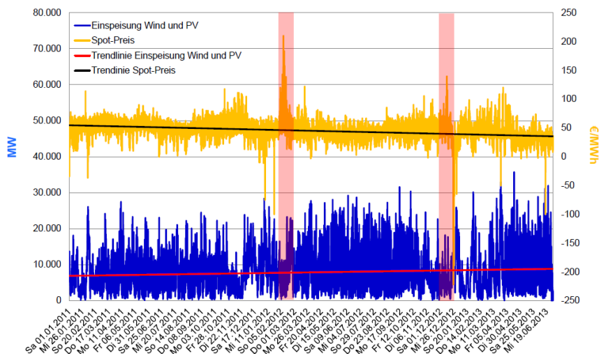
Figure 62: The decrease in average electricity price with the rise of the PV and wind productions (Tennet, Op. cit.)
