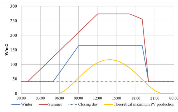
Figure 73: Consumption profile and maximum production curve of PV electricity
