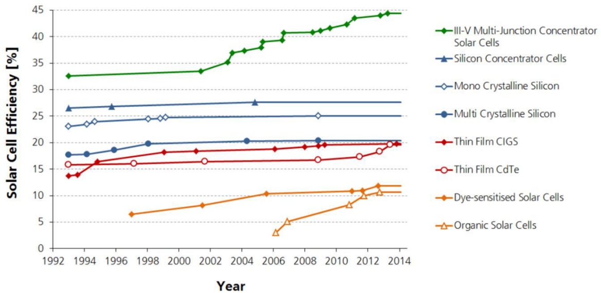
Figure 10: Overview of solar PV technology efficiency gain (R&D)
