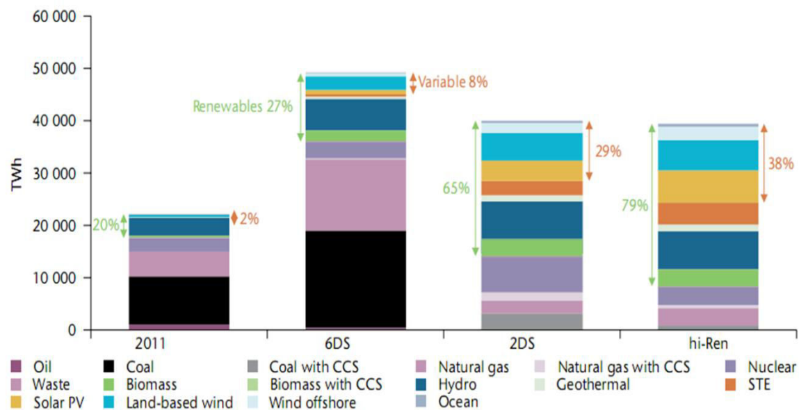
Figure 36 : IEA's global electricity mix in 2050 (IEA, 2014) 47
