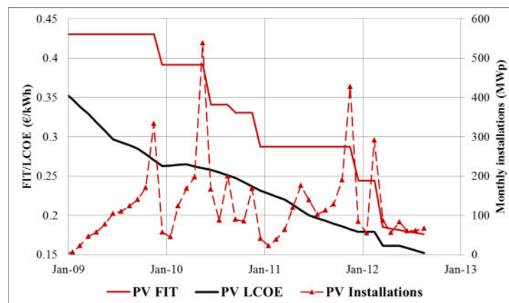
Figure 57: PV installation peaks under the FIT system in Germany for PV systems of 10 kWp – 30 kWp.
