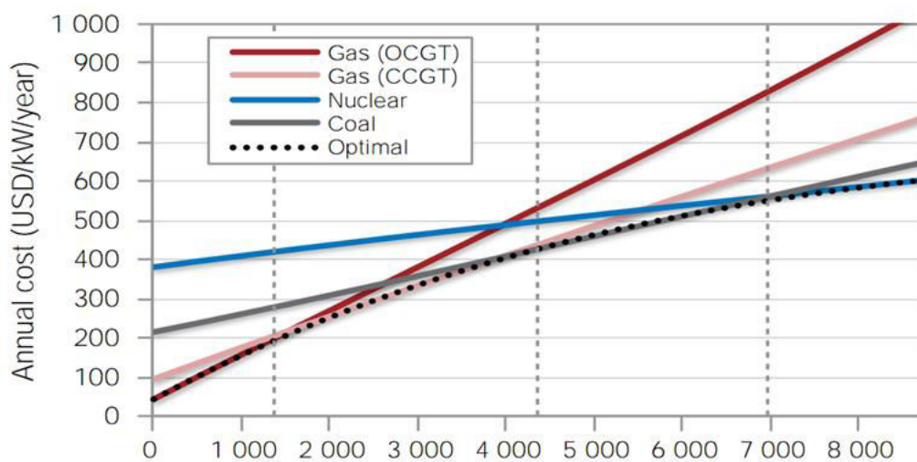
Figure 28: Example of mix optimization with gas, coal and nuclear capacities (OECD/NEA, 2012, pp. 133, Ch. 4, Box 4.4)
