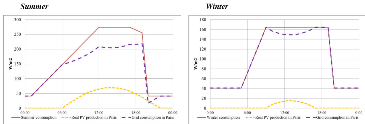
Figure 74: Demand from the grid with and without self-consumption
