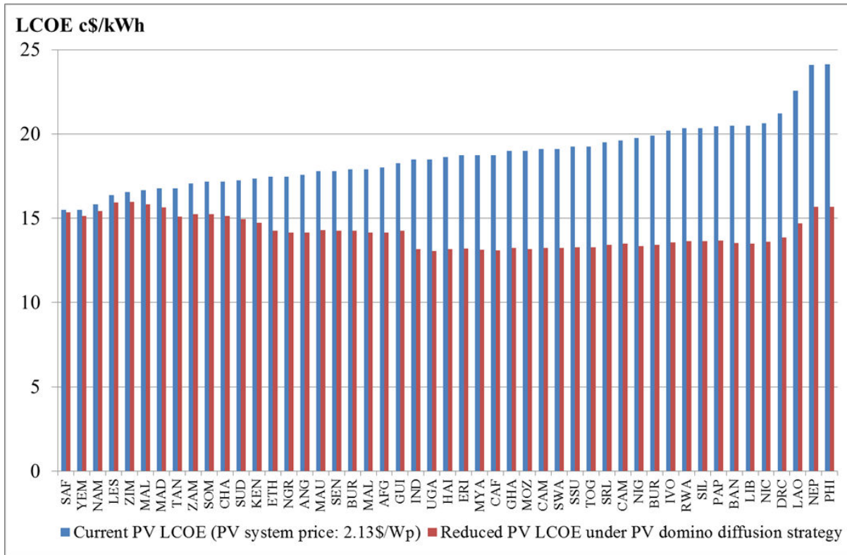
Figure 90: Reduced PV LCOE with the PV domino diffusion strategy model (in red) vs. current PV LCOE with a PV system price of 2.13$/Wp (in blue) (author’s proposal with 12% discount rate)
