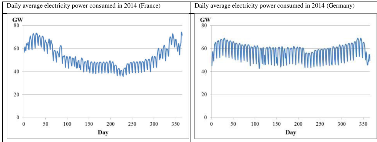
Figure 31: Consumption profiles in France and Germany 41
