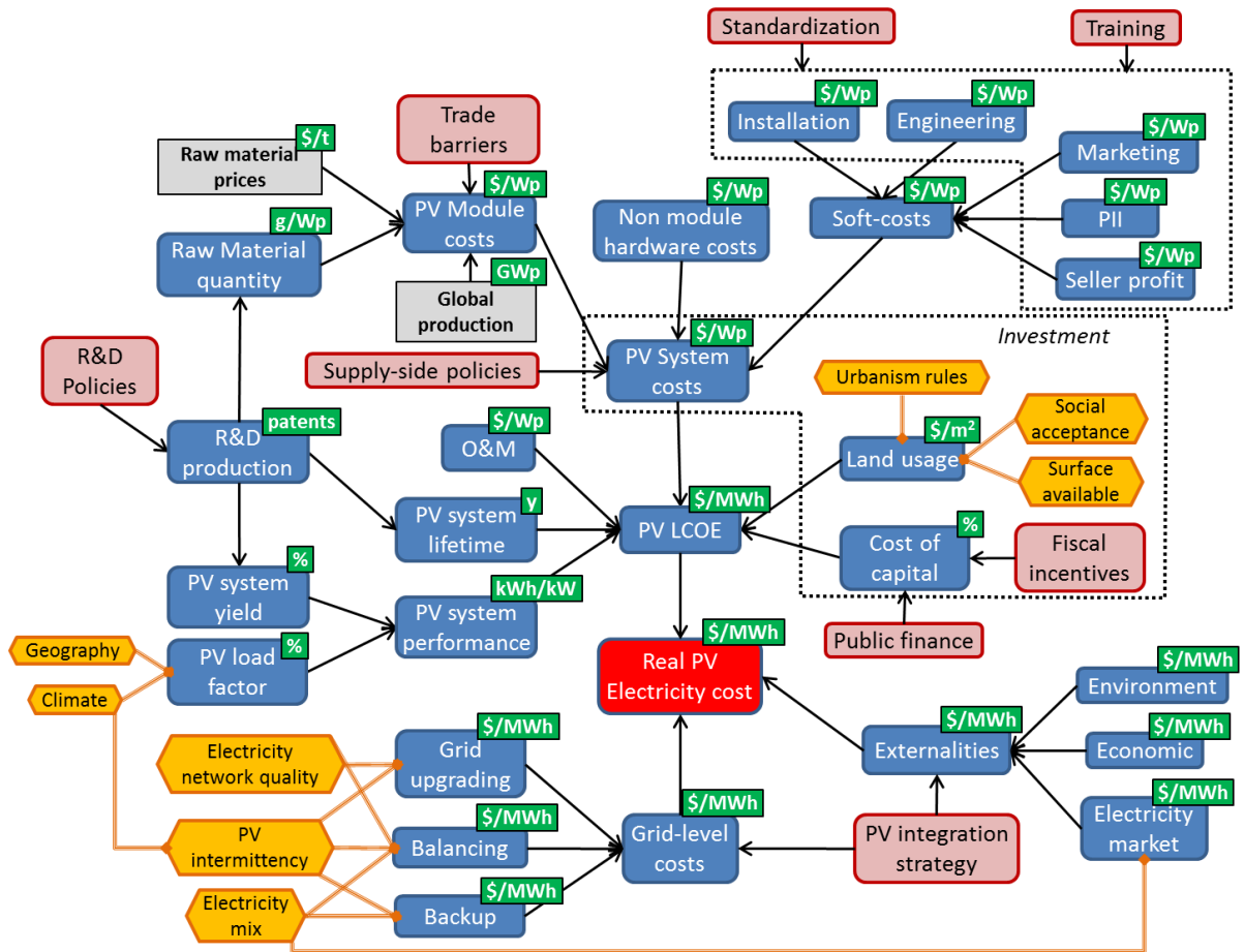
Figure 50: PV integration: reduction of real PV electricity costs ($/kW) (author's proposal)
