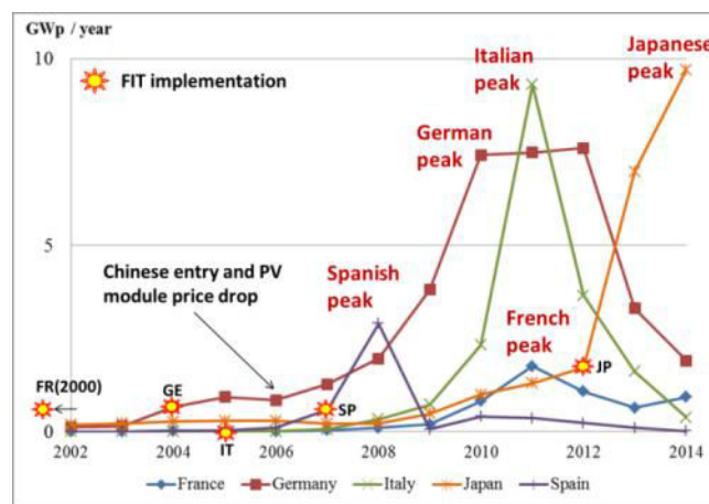
Figure 55: Annual installation peaks under the FIT system (IEA PVPS, 2002 to 2014; Campoccia, et al., 2014)
