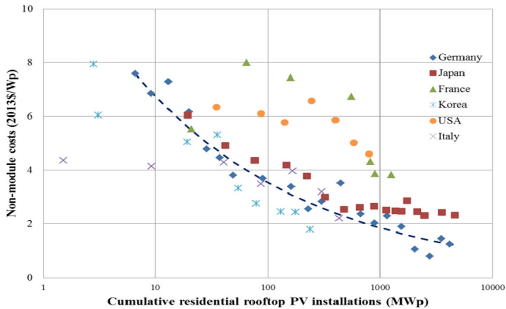
Figure 17: Learning curve for non-module costs of PV rooftop systems in different countries 28 .
