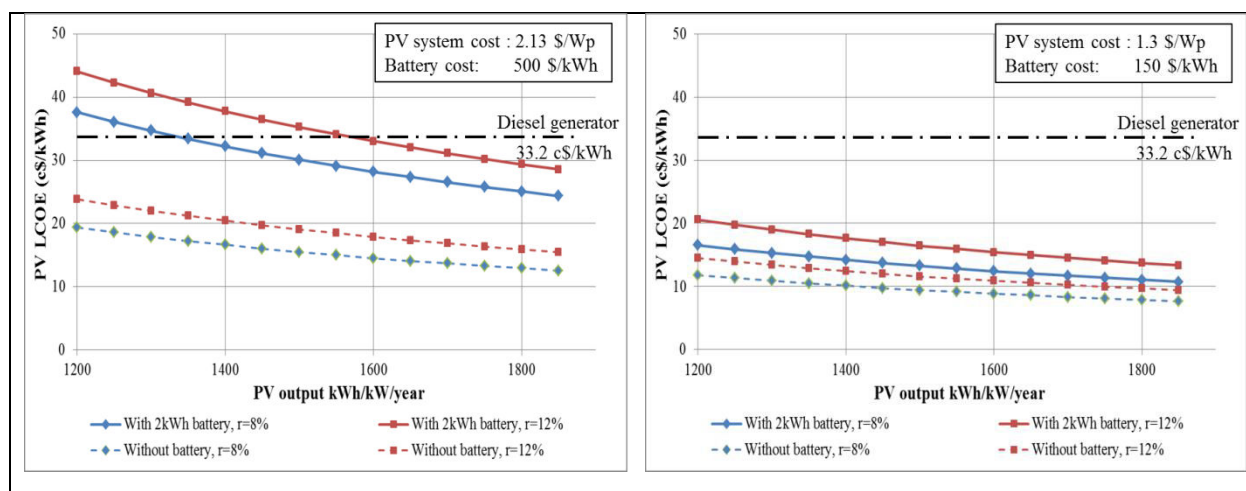
Figure 88: PV LCOE with 0.6 kWp PV system + 2kWh batteries based on discount rates of 8% and 12%: current PV LCOE (left) and reduced PV LCOE (right)
