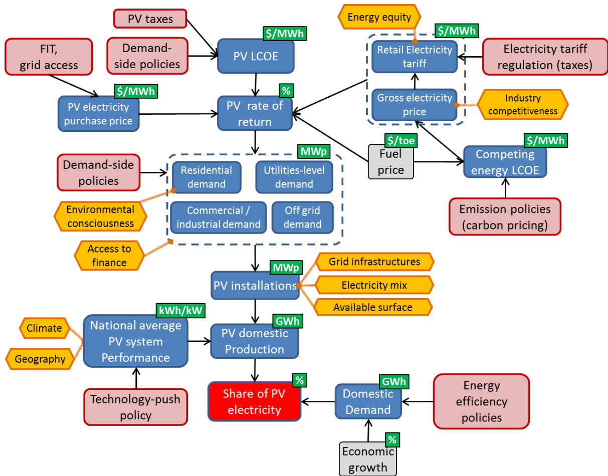
Figure 48: PV demand: the share of PV electricity in electricity mix (author’s proposal)
