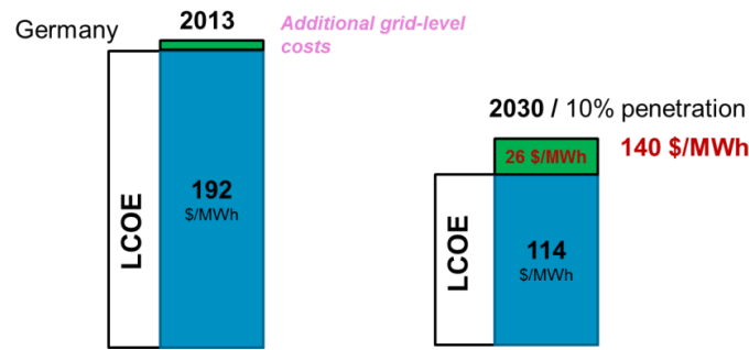
Figure 54 Estimated residential PV costs in Germany in 2030 with grid-level costs included
