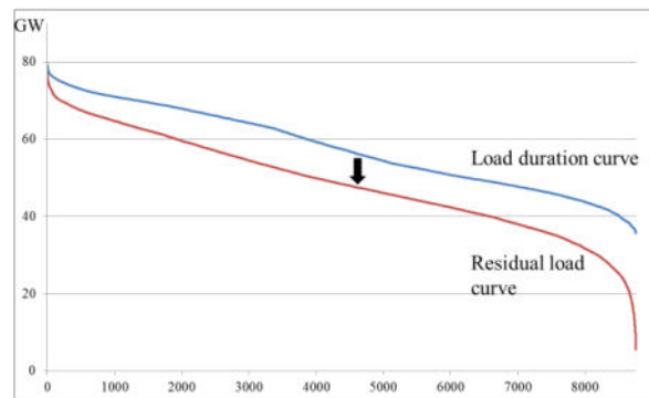
Figure 60: German load duration curve in 2014 and residual load 123
