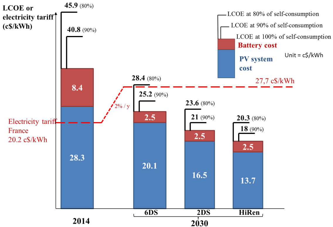
Figure 76 : Economic feasibility of residential PV self-consumption model combined with batteries in 2030
