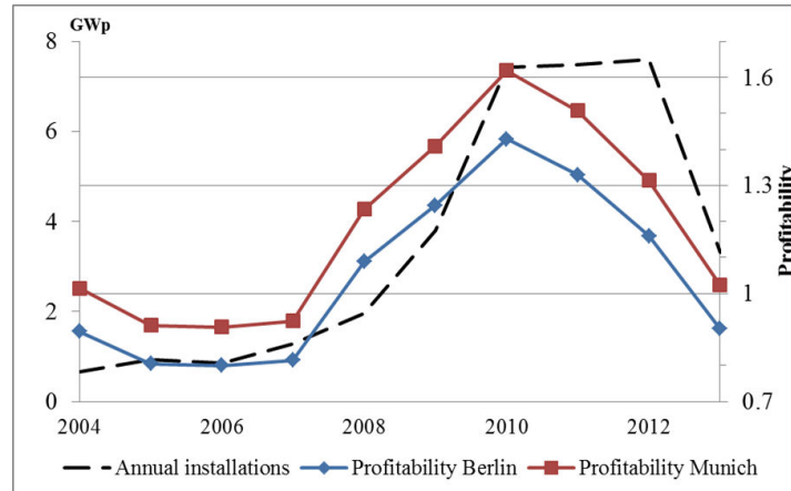
Figure 51: PV profitability of a rooftop PV system in Germany & annual PV installations 99
