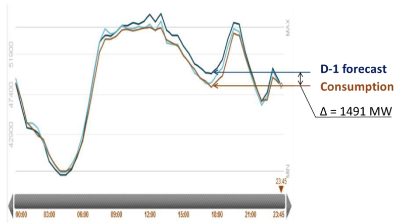
Figure 32: Day-ahead forecast and consumption for October 17 2014 in France (RTE).
