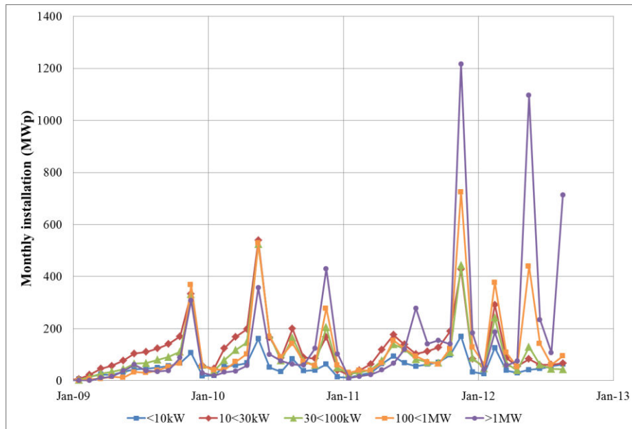
Figure 58: PV installation peaks in Germany according to the size of PV systems
