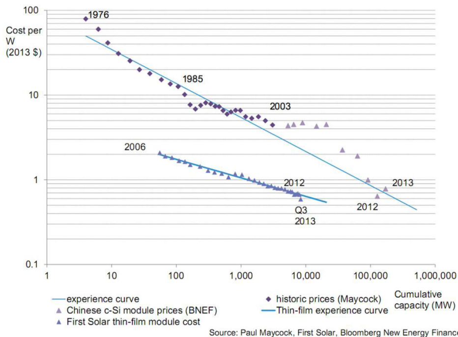
Figure 11: Learning curve (or experience curve) 25 for c-Si technologies and thin film technologies (Bloomberg New Energy Finance, 2014b)
