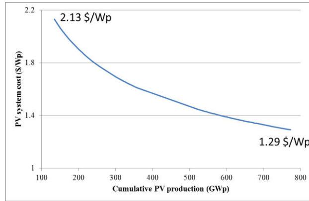
Figure 87: Estimated PV system cost (with a learning rate of 18%)
