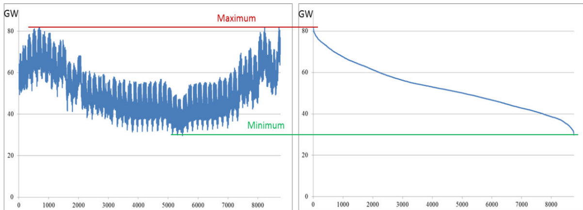
Figure 29: Hourly consumption profile in France in 2014 and load duration curve 37
