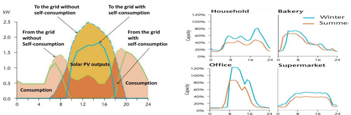
Figure 68: PV self-consumption without storage (residential PV system) (IEA, 2014; IEA, 2014b) (left)
