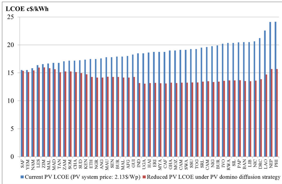
Figure 90: Reduced PV LCOE with the PV domino diffusion strategy model (in red) vs. current PV LCOE with a PV system price of 2.13$/Wp (in blue) (author’s proposal with 12% discount rate)
