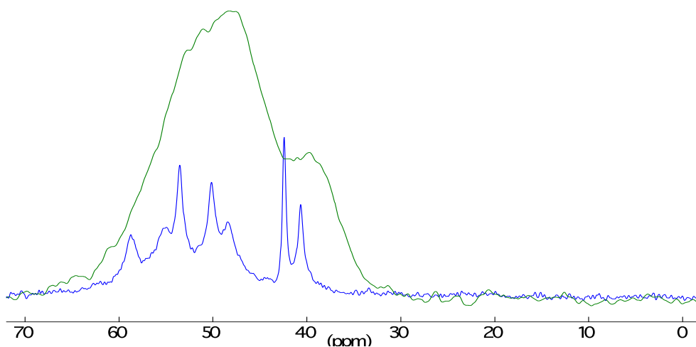
Figure III-6 Blue line: ^{13}\text{C} HPDec spectra of PEI (Recycle time: 3s@30°; NS: 280; rotation: 300 Hz); green line: ^{13}\text{C} - \{^1\text{H}\} CP-MAS NMR of \text{SiO}_2 @PEI (Recycle time: 1s; contact time: 1ms; NS: 4096; rot: 5 kHz)
