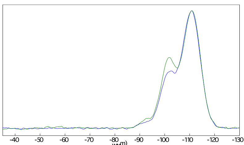
Figure III-2. 29 Si MAS NMR spectra of (blue line) SiO 2 -SO 3 and (green line) SiO 2 -Cl. Experiments were carried out using a single-pulse technique and high power 1 H decoupling (HPDEC) at a 5 kHz spinning rate with 30° pulses and a recycling delay of 60 s with 720 and 840 scans, respectively
