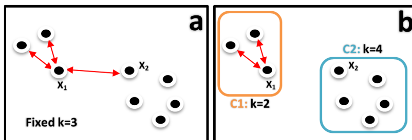
Figure 3.4: (a) Fixed k -nearest neighborhood. (b) Adaptive k -nearest neighborhood
