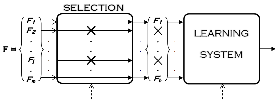
Figure 2.2: General framework of feature selection
