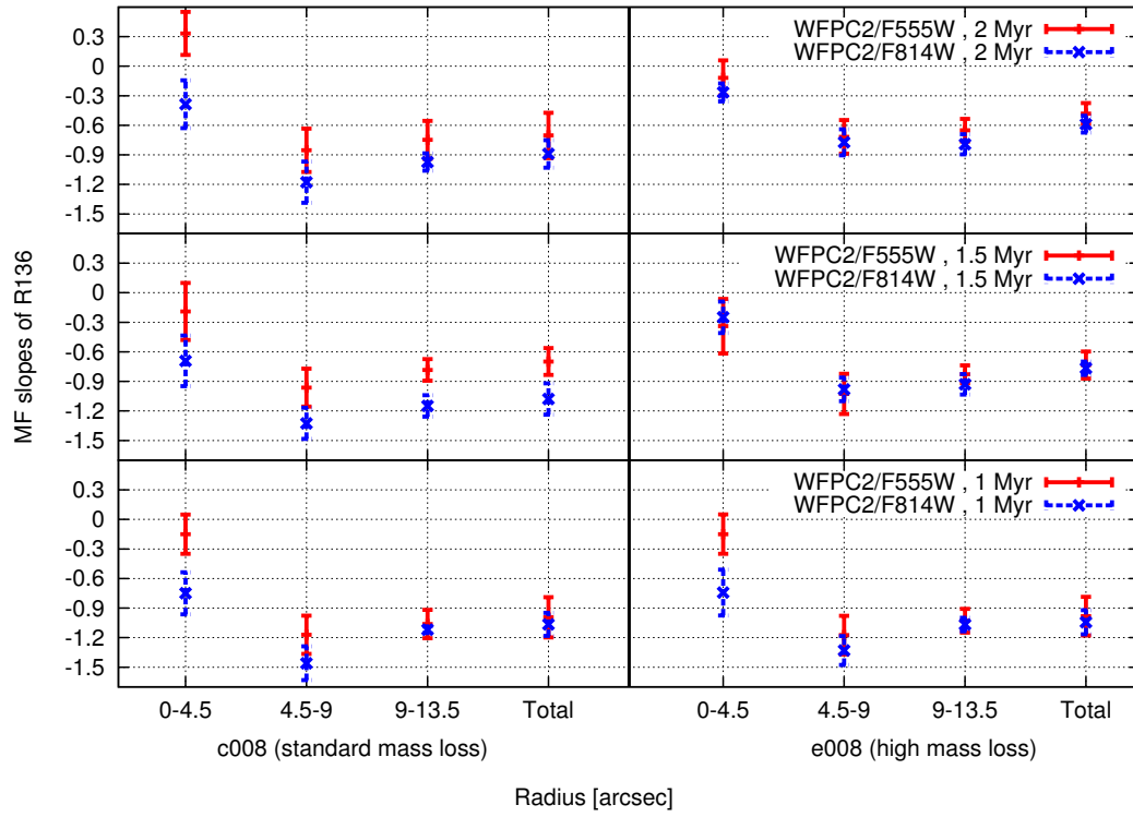
Figure 2.12 Mass function slopes of R136 derived in F555W (red) and F814W (blue) for the whole cluster and in three different regions using three different isochrones: 2, 1.5 and 1 Myr from top to bottom. Left plot is for the standard mass loss (c-models from Geneva stellar evolution models) and right plot for enhanced mass loss (e-models from Geneva stellar evolution models)
