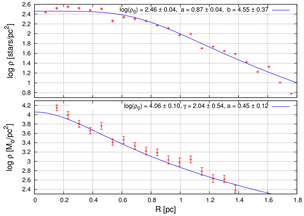
Figure 5.20 Projected density profile of R136 in IRDIS FoV centered on R136a1. Up: number density [stars/pc 2 ]. Number of stars is taken from the catalog of common stars between IRDIS, J and Ks data. Bottom: mass density [M ⊙ /pc 2 ]. The stellar masses are estimated at the age of 2 Myr with extinction values of A_J = 1.3 \pm 0.5 and A_K = 0.4 \pm 0.5 in J and Ks band. Eq. 5.1 and Eq. 5.2 are used to fit the blue solid line to the data in upper and bottom plots, respectively.
