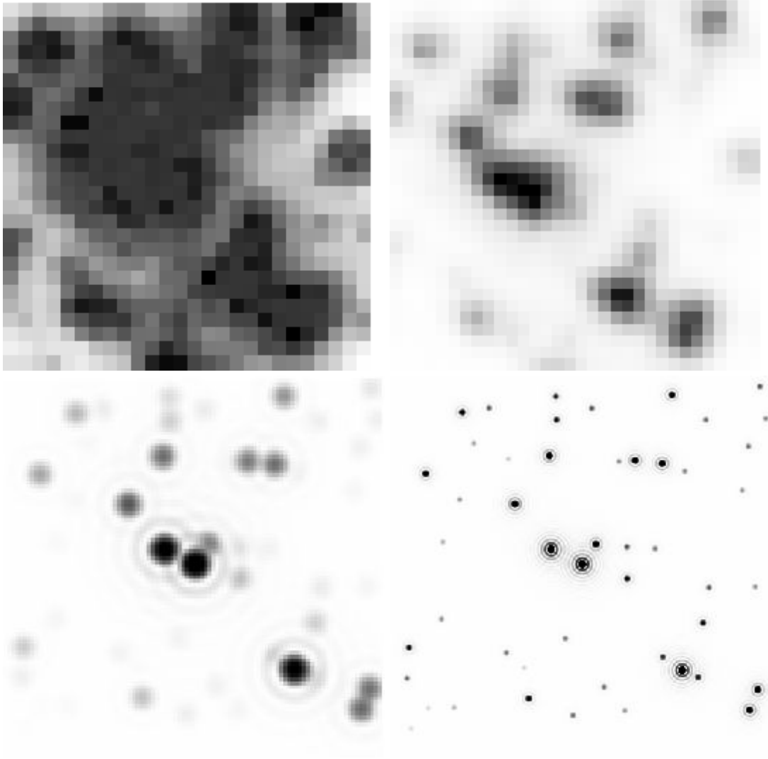
Figure 5.26 FoV: 1.225'' \times 1.225'' of the core of R136 taken by HST in V-band at the top (Left:WFPC2 and Right: WFC3). At Bottom is the reconstructed images of IRDIS/Ks (left) and E-ELT/MICADO/Ks (right), with the same FoV as top images.
