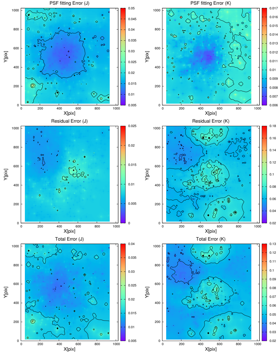
Fig. 5. Map of the photometric, residual and total error-bars. Top: map of the PSF fitting errors (outcome of the Satfinder photometry) along the IRDIS FoV. Middle: map of the residual errors, outcome of the background analysis after removing the stellar sources signals from the image. Bottom: map of the total error, combination of the PSF-fitting errors and the residuals background errors. Left images are in the J band. Right images are in the Ks band
