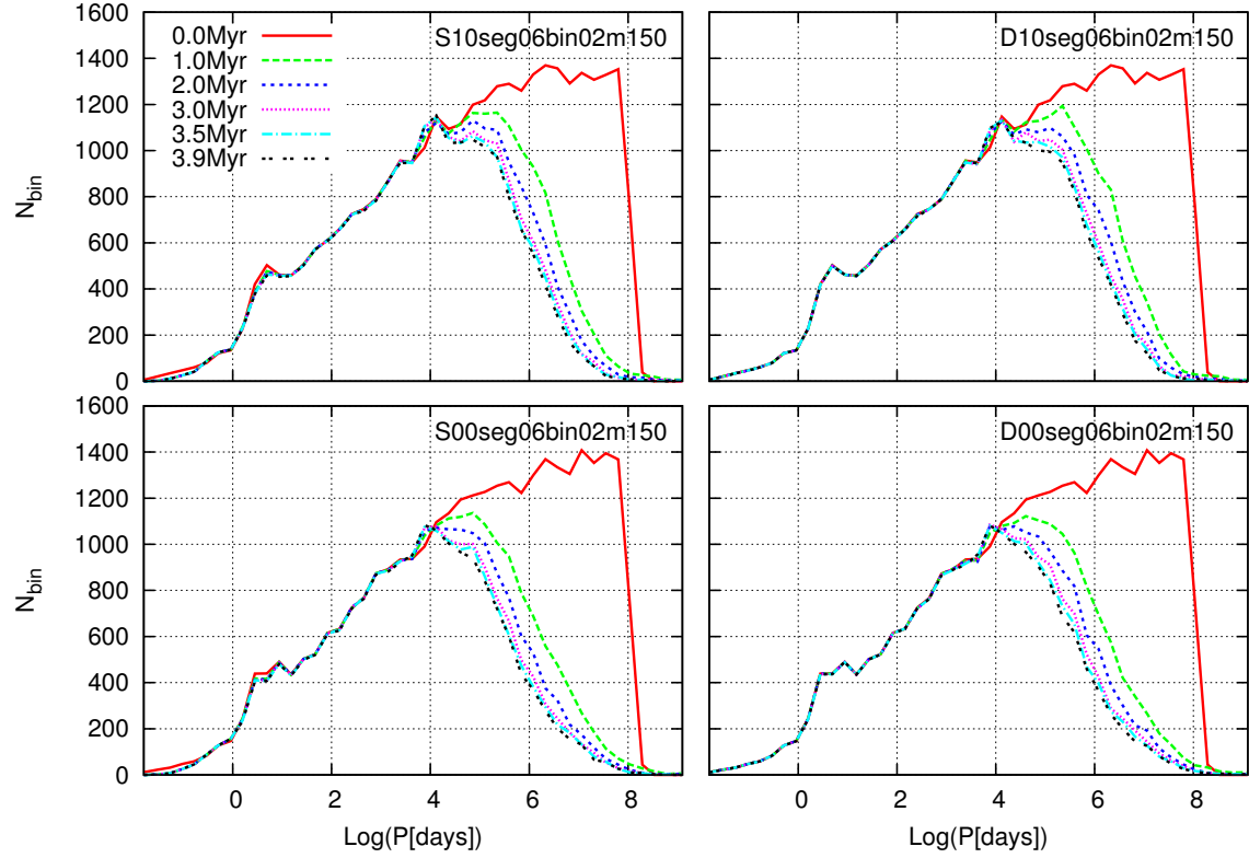
Figure 3.9 Histogram of the Log(period [days]) of bound binary systems in 6 time-steps (0.0, 1.0, 2.0, 3.0, 3.5 and 3.9 Myr) for 4 clusters with mass range of 0.2M_{\odot} - 150M_{\odot} and 60% Initial binaries.
