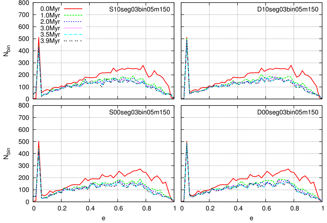
Figure 3.10 Histogram of the eccentricity of bound binary systems in 6 time-steps (0.0, 1.0, 2.0, 3.0, 3.5 and 3.9 Myr) for 4 clusters with mass range of 0.5M_{\odot} - 150M_{\odot} and 30% Initial binaries.
