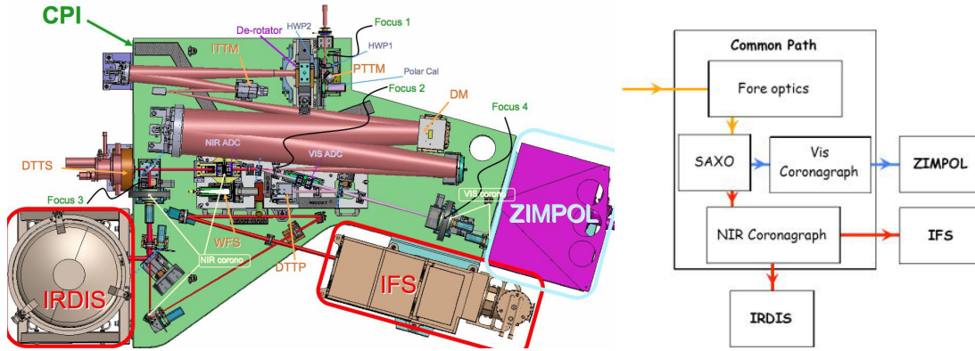
Figure 1.9 SPHERE instruments (courtesy of ESO).
