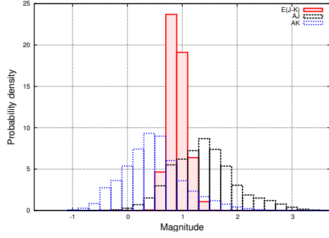
Fig. 9. Generalized histogram of the extinction of 54 spectroscopically known stars from Crowther et al. 2016. (shown in Figure 7). We used PARSEC models to estimate the extinction for each of these stars according to its age-range.
