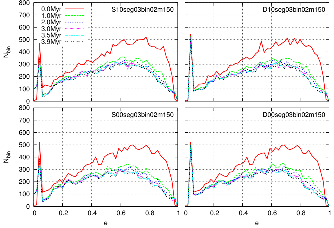
Figure 3.12 Histogram of the eccentricity of bound binary systems in 6 time-steps (0.0, 1.0, 2.0, 3.0, 3.5 and 3.9 Myr) for 4 clusters with mass range of 0.2M_{\odot} - 150M_{\odot} and 30% Initial binaries.
