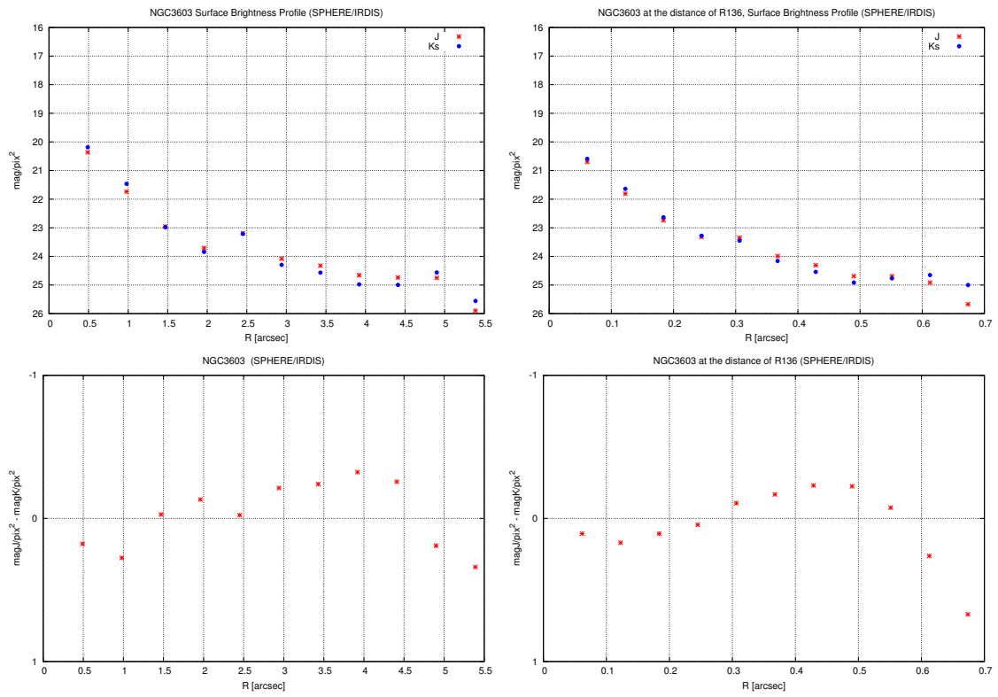
Figure 5.24 Top: SBP of NGC3603 in SPHERE/IRDIS J and K band data. Bottom: the difference of Kmag/pixel-Jmag/pixel. Left: NGC3603 real images. Right: NGC3603 in the distance of R136.
