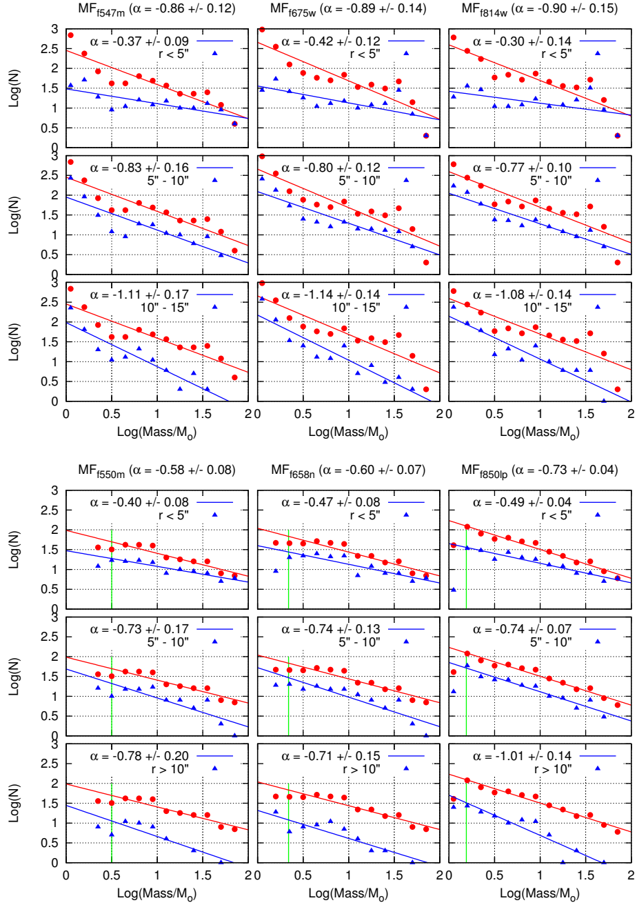
Figure 2.10 Mass function of NGC 3603 derived for the whole cluster (red dots) and in three different regions (from top to bottom). Top: Data from three WFC2 filters (F547M, F675W, F814W). Bottom: Data from three ACS/HRC filters (F550M, F658N, F850LP)
