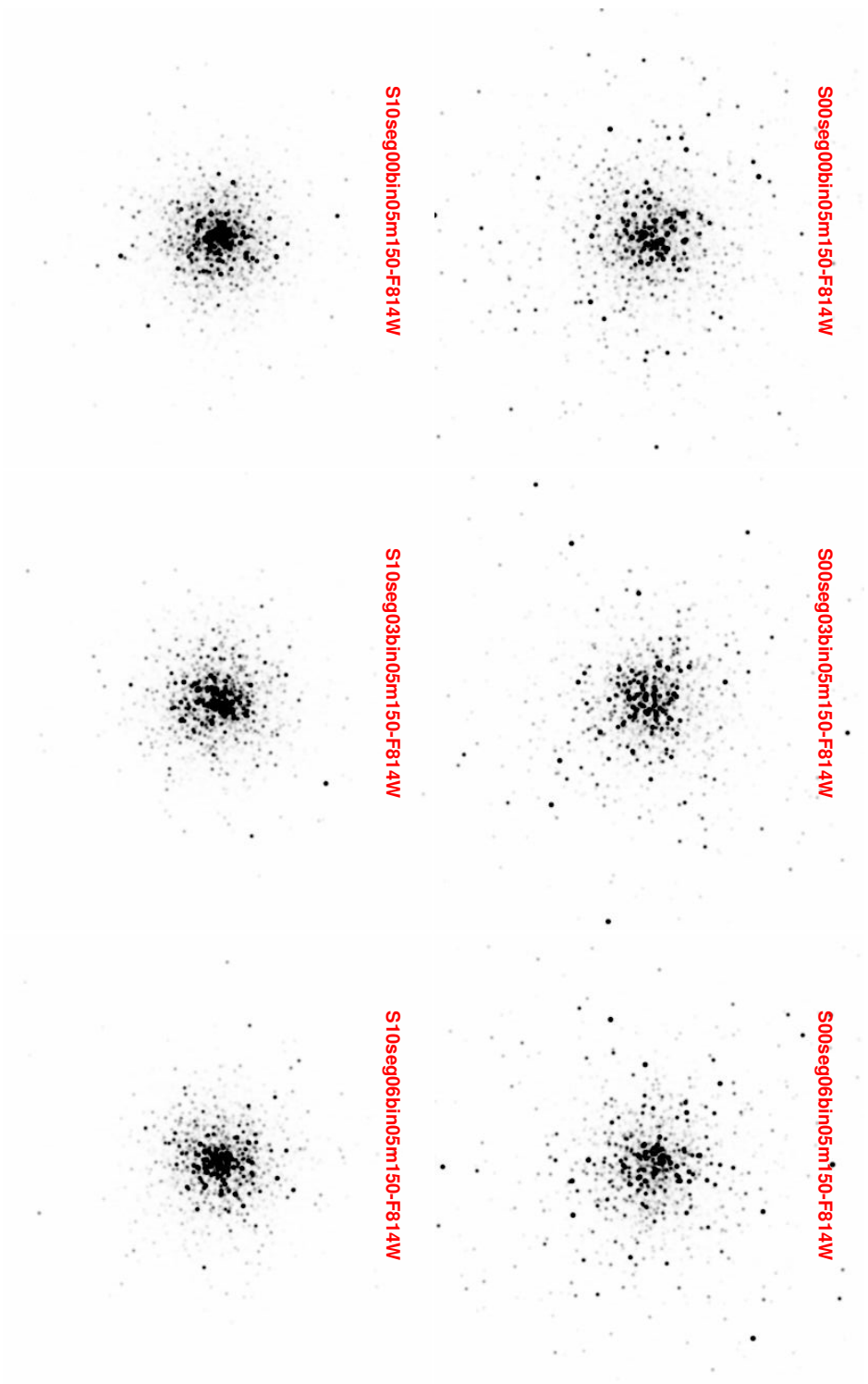
Figure 3.17 Same as Figure 3.15 but in XY plane.
