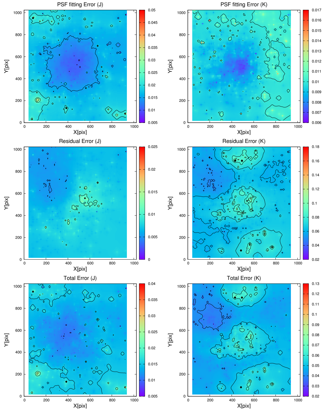
Figure 5.9 Top: map of the PSF fitting errors (outcome pf the Satrfinder photometry) along the IRDIS FoV. Middle: map of the residual errors, outcome of the background analysis after removing the stellar sources signals from the image. Bottom: map of the total error, combination of the PSF-fitting errors and the residuals background errors. Left: J; Right: K
