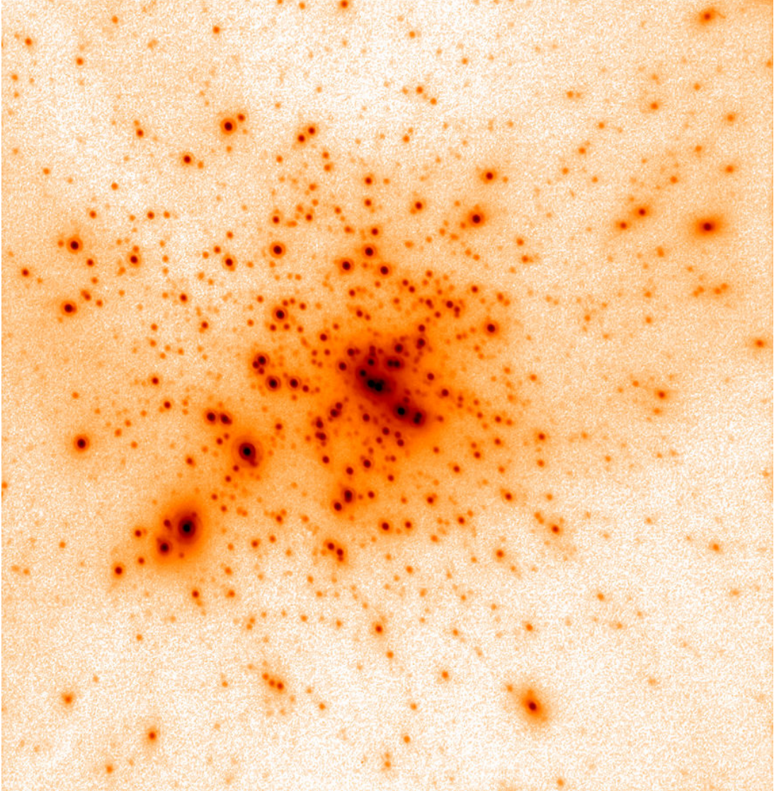
Figure 5.1 SPHERE/IRDIS images of the core of R136 in K-band.
