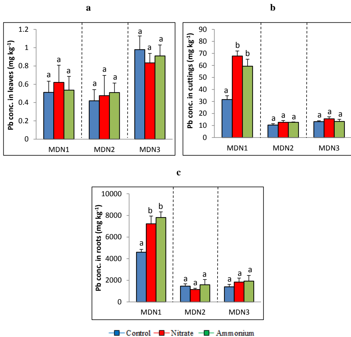
Figure 4.2.8: Effects of nitrogen nutrition on Pb concentrations in leaves (a), cuttings (b) and roots (c) of Populus euramericana Dorkamp grown in a contaminated technosol during 35 days (n = 5), bars refer to standard error, letters indicate differences between treatment for a given soil.
