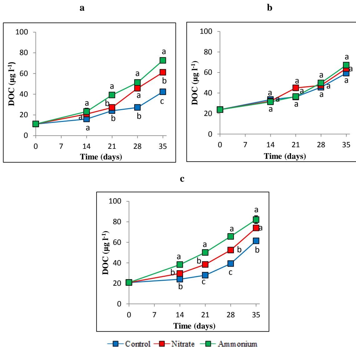
Figure 4.2.2: Effects of nitrogen nutrition on rhizospheric DOC concentrations of Populus euramericana Dorskamp grown in a contaminated technosol, MDN1 (a), MDN2 (b) and MDN3 (c), during 35 days (n = 5), bars refer to standard error. For each day measurement, letters indicate differences between control and treated soils.
