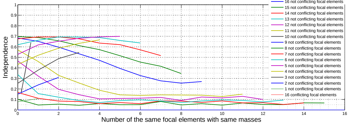
Figure 4.10: The independence when the number of focal elements is 16 and |\Omega| = 5
