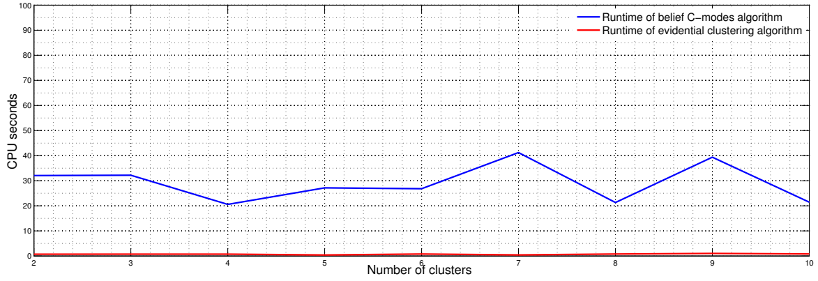
Figure 3.5: Comparison of run-times of belief C -modes and evidential clustering when N = 200 , |\Omega| = 5 and C \in [2, 10]
