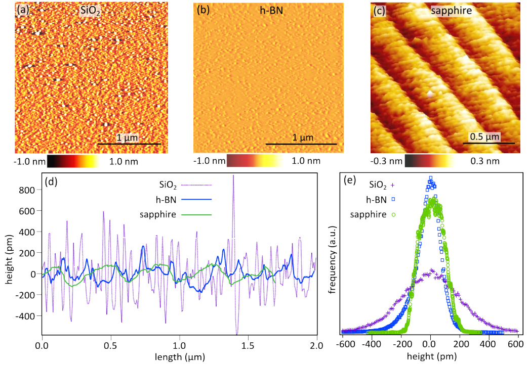
Figure 2.9: Roughness comparison of different substrates a), (b) and (c): height mapping of the surfaces of the silica, h-BN and sapphire respectively d) Height profile through arbitrary lines in the corresponding mappings in a, b and c e) Histogram of the height distribution over the whole windows of a, b and c: histogram areas have been normalized.
