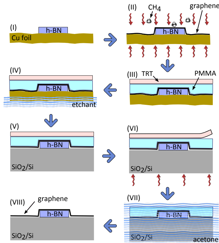
Figure 3.6: Growth and transferring process of the samples h -BN is first mechanically exfoliated on the copper foil (I). Then through a typical CVD process, graphene is grown on the foil covering h -BN flakes (II). After cooling, Poly(methyl methacrylate) (PMMA) is spun on the sample and thermal release tape (TRT) is used to support them (III). At the next step Cu foil is etched away by using a right solution of ammonium persulfate (IV). After washing the sample with distilled water, it is dried out using a nitrogen gun and is transferred on a surface activated wafer (V). Finally by applying heat (VI) and treatment with acetone (VII), TRT and PMMA are removed one after the other.
