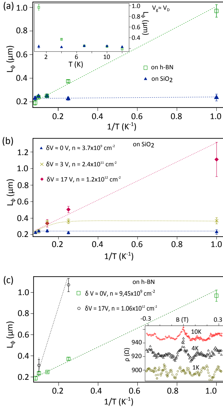
Figure 2.15: Coherence length as a function of the temperature for the devices a) Comparison of the behaviors of the coherence lengths for gr/h — BN and gr/ \text{SiO}_2 at the gate voltage close to the Dirac point versus inverse temperature: While cooling the sample, the L_\phi for gr/h — BN increases monotonically, it saturates rapidly for the gr/ \text{SiO}_2 . Inset is the same data plotted as a function of the temperature. b) Temperature dependency of the L_\phi for the gr/ \text{SiO}_2 at different densities: Electron and hole puddles limit the coherence length of the carriers at low densities. c) Temperature dependency of the L_\phi for the gr/h — BN at different carrier densities: no clear saturation as what is seen for the case of gr/ \text{SiO}_2 is detectable for the gr/h — BN. In high doping regime, L_\phi reaches the length of the sample very rapidly at 4 K; further cooling of the sample (inset figure) leads to elimination of the weak localization. Dashed lines in all the cases are guides for the eyes. Also \delta V = |V_g - V_D| where V_D : Dirac point voltage.
