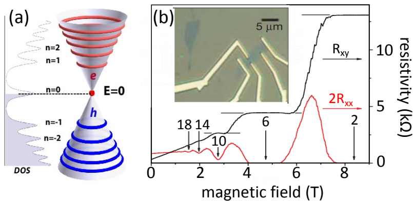
Figure 1.10: Quantum Hall effect in graphene under high magnetic field
