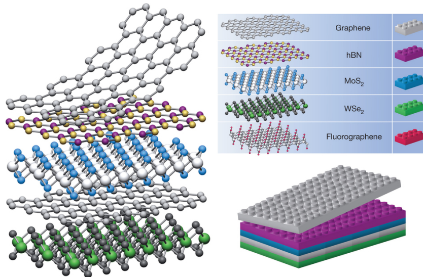
Figure 2.1: Building complex heterostructures based on mono- and few layer 2D materials (reprinted from [62]) Planner isolated thin crystals can be viewed as Lego blocks (right panel) which make the construction of layered structures out of mixed materials possible.
