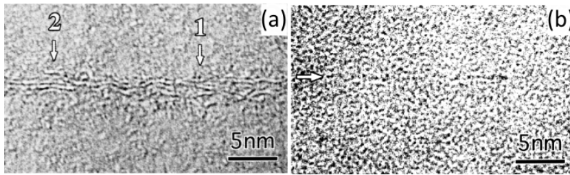
Figure 1.3: Selected of the results reported in Horiuchi's paper [27] a) and b) High-resolution TEM images they obtained from graphite samples after chemical exfoliation: They believe that at the site marked by arrows in (a) graphene layers separate into branches. Also the hardly visible dark line along the arrow in (b) corresponds to a single graphene layer.
