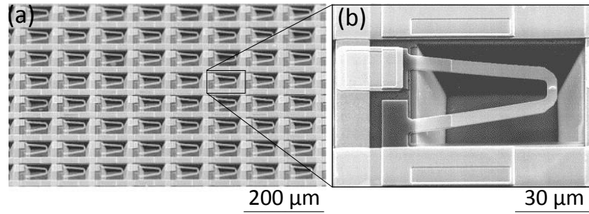
Figure 4.1: SEM images of one of the first NEMS devices a) A compact array of the cantilevers made for thermal data storage b) Focused image on one of the cantilevers
