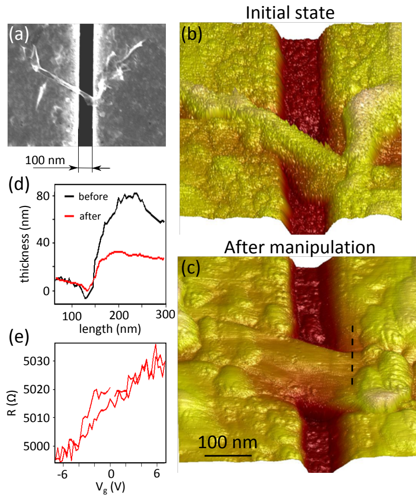
Figure 6.9: AFM manipulation to reduce the thickness of a suspended graphene flake a) SEM image of a suspended graphene realized by directly exfoliating graphene on predefined array of superconducting electrodes b) Corresponding AFM mapping of this sample at initial state c) AFM mapping of the same sample after several steps of manipulation with AFM tip d) Thickness profile of this flake before and after AFM manipulation measured along the dashed line marked in c e) Corresponding field effect measurement after AFM manipulation
