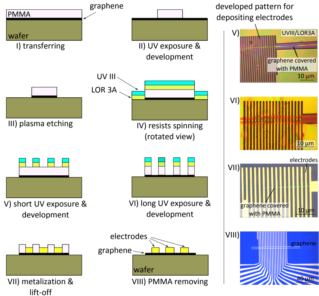
Figure 4.11: Process flow of the recipe developed for preserving the quality of the graphene Different fabrication steps are demonstrated schematically in the left side and described in the text. Right: Optical micrographs taken at the steps V through VIII
