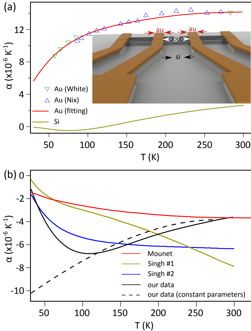
Figure 4.18: Temperature dependency of the coefficient of thermal expansion (CTE, \alpha ) of graphene a) CTE of gold and silicon used in the calculation of the data in (b): While Au (White) and Au (Nix) refer to the data reported in [180] and [181] respectively, the CTE for silicon are reprinted from [182]. Red line is the polynomial fit for both sets of the gold data which we use to calculate the CTE of graphene. b) Extracted CTE of graphene and comparison with the previous theoretical (Mounet2005) [57] and experimental (Singh2010 #1 and #2) [58] works. While the temperature dependency of the CTE of silicon and gold are not considered in the calculation for the dashed black line, the solid black curve is obtained by including these effects.
