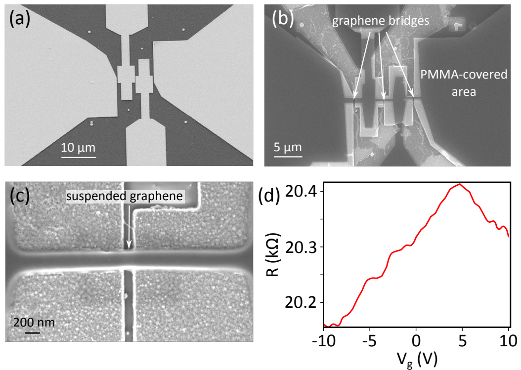
Figure 6.3: Second generation of our graphene on superconducting-lectrode devices a) Superconducting Al/Pd electrodes are deposited at the first step. b) CVD graphene covered with PMMA layer is transferred on the electrodes and is patterned. c) By removing the PMMA layer, the sample is ready for the measurements. d) Two-probe resistance versus gate voltage measurements of this sample shows the graphene ribbon is of low transport quality.
