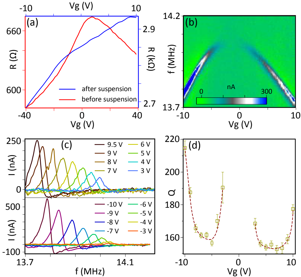
Figure 4.15: Room temperature electrical and mechanical measurements of sample 2 a) Two probe gate dependence of the resistance before and after under etching the sample
