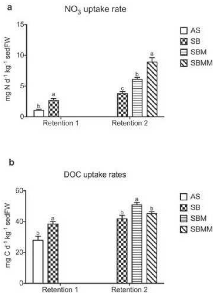
Figure 4-3 \text{NO}_3^- uptake rates (a) and DOC uptake rates (b) at the end of the experiment (mean \pm SE). Sample numbers are n = 4 for AS, n = 16 for SB in Retention 1, and n = 4 for SB, n = 6 for SBM, and n = 6 for SBMM in Retention 2. Different characters (“a”, “b”) resulting from statistic tests mark the treatments with significantly differences.
