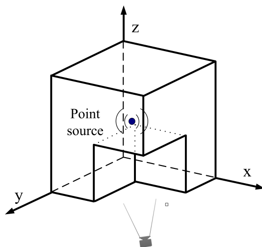
Fig. 5.6 The building model with re-entrant corner.
