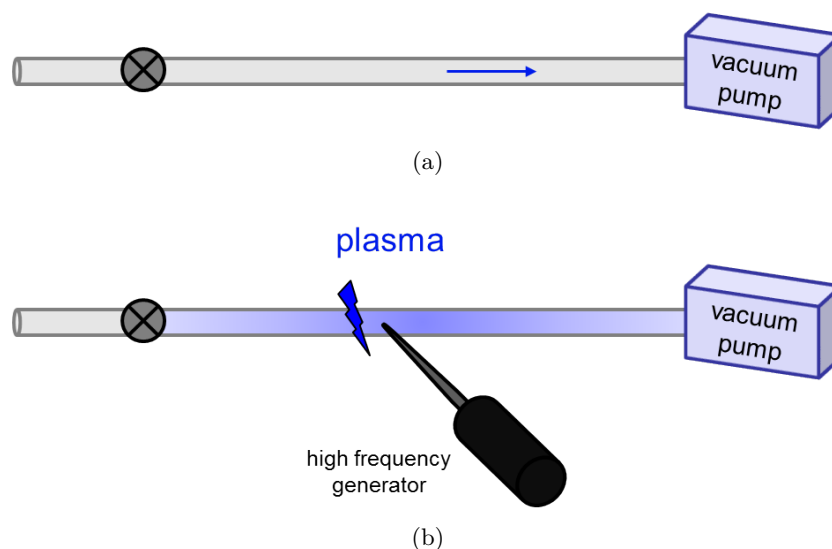
FIGURE 2.9: Schematic representation of the plasma treatment: (a) first step vacuum, (b) second step plasma ignition. The plasma propagates along the tube L_{tube} = 1.5 m.
