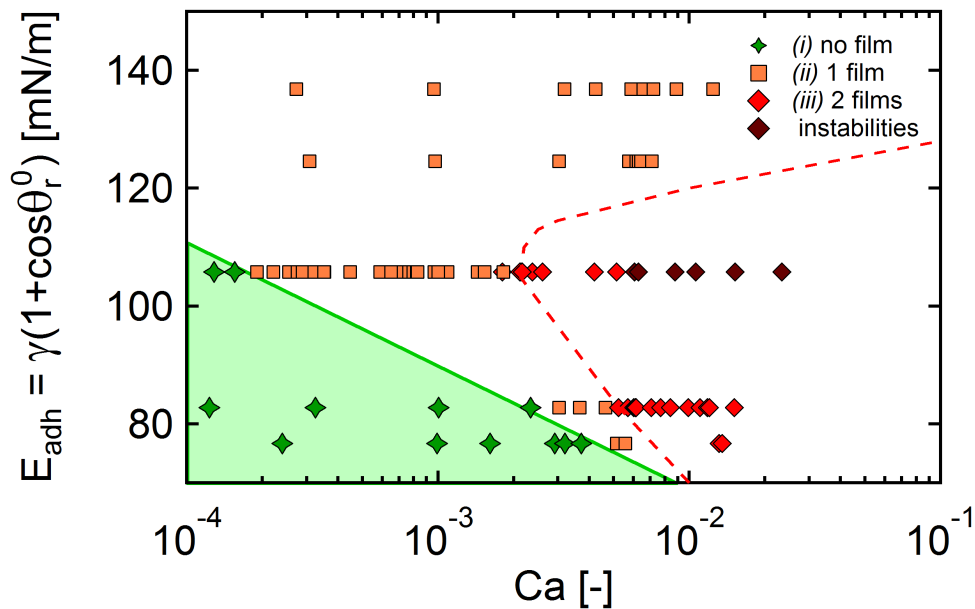
FIGURE 7.4: Phase diagram for pure water: adhesion energy E_{adh} = \gamma(1 + \cos\theta_r^0) versus capillary number Ca . The green and the red curves correspond to the qualitative limit between regime (i) and (ii), and regime (ii) and (iii) respectively.
