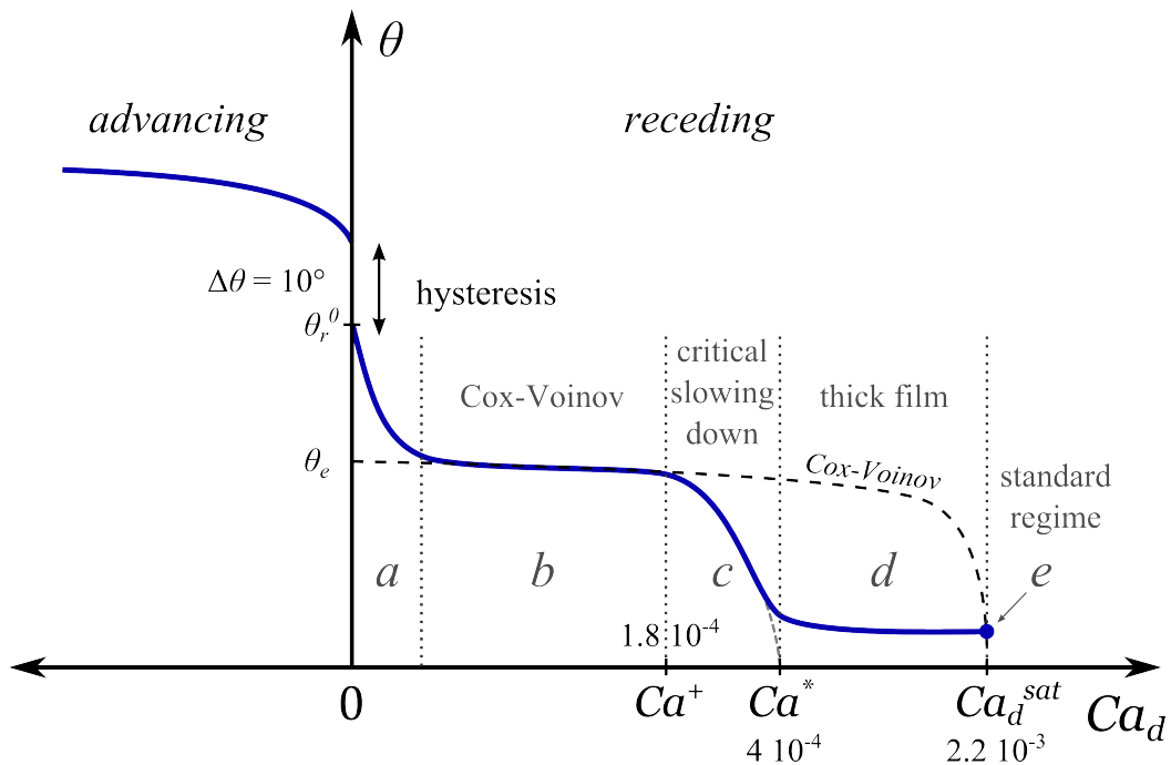
FIGURE 7.2: Schematic of the evolution of the dynamic contact angle \theta as a function of the capillary number based on the triple line velocity Ca_d . Advancing contact lines correspond to negative velocities. Values are given for PVC tubes.
