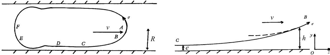
FIGURE A.1: Bretherton problem: air bubble displaced in a capillary [14].
