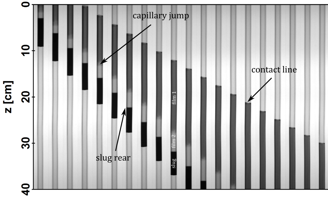
FIGURE 5.2: Image sequence for a typical experiment in regime (iii), i.e for Ca > Ca^* , where two films are formed. Experimental parameters are: 20%wt glycerol solution ( \eta = 1.66 \text{ mPa}\cdot\text{s} ), v = 15.8 \text{ cm}\cdot\text{s}^{-1} , Ca = 4 \cdot 10^{-3} , \Delta t = 0.2 \text{ s} .
