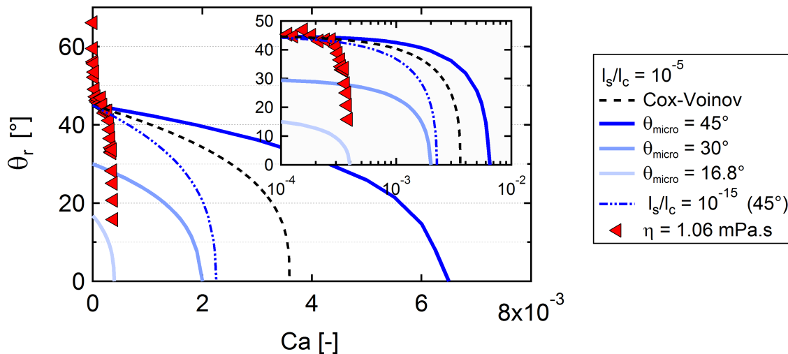
FIGURE 3.6: Experimental contact angle for 5%wt glycerol solution ( \eta = 1.06 mPa.s red triangles), Cox-Voinov model (dashed lines) and model assuming a constant microscopic contact angle \theta_{micro} (solid lines). Logarithmic scale in inset.
