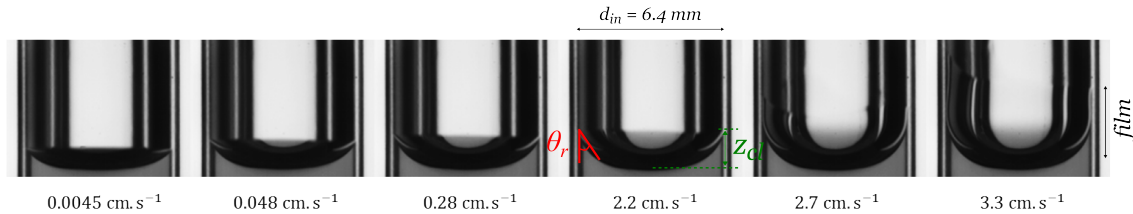
FIGURE 3.2: Images of a receding meniscus for various meniscus velocity v as indicated below each image. The tube diameter is 6.4 mm. The liquid used is 5wt% glycerol solution, \eta = 1.06 mPa.s. The meniscus elevation z_{cl} and receding contact angle \theta_r are measured for each value of v . z_{cl} increases and \theta_r decreases with increasing v . Above a threshold velocity v^* , a liquid film is entrained as observed on the last image.
