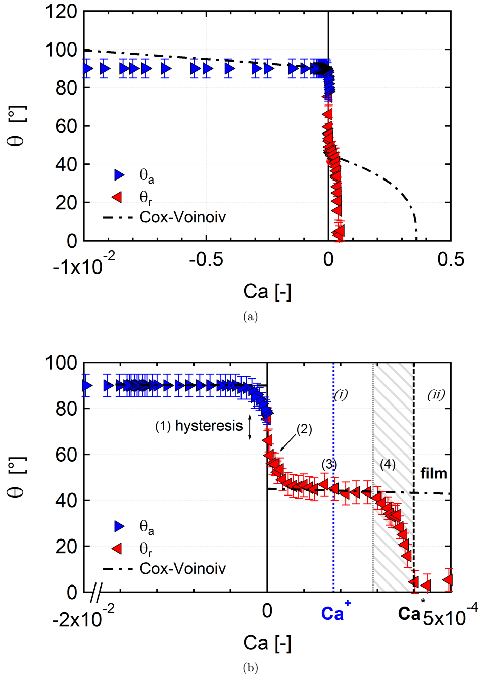
FIGURE 3.3: Advancing \theta_a and receding \theta_r contact angles as a function of the capillary number Ca for a 5%wt glycerol solution ( \eta = 1.06 mPa.s). (a) Full Ca scale (b) zoom in. By convention, receding contact lines have a positive velocity. The dotted-dashed curve represents the Cox-Voinov prediction for \theta_e = 45^\circ for receding and \theta_e = 90^\circ for advancing triple line (Equation (1.13)). The black dashed vertical line indicates our measurement of the dynamic wetting transition ( Ca^* ). The blue vertical dotted line indicates Ca^+ as defined in Section 3.5.
