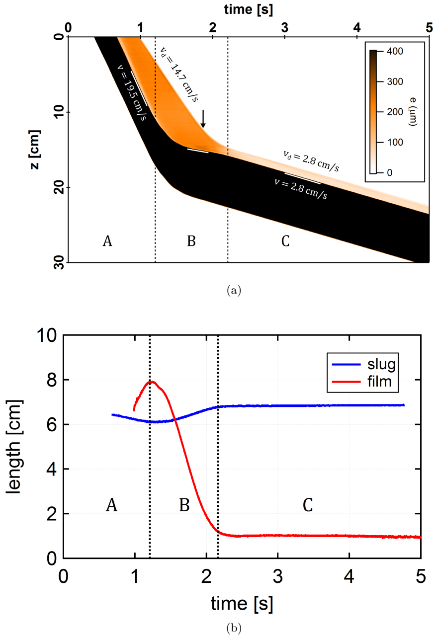
FIGURE 4.18: (a) Spatio-temporal diagram of film thickness for an experiment with water ( \eta = 0.94 \text{ mPa}\cdot\text{s} ), where we have suddenly decreased the velocity of the slug during the flow. The velocity goes from 19.5 \text{ cm}\cdot\text{s}^{-1} to 2.8 \text{ cm}\cdot\text{s}^{-1} . (b) Corresponding slug and film length evolution with time.
