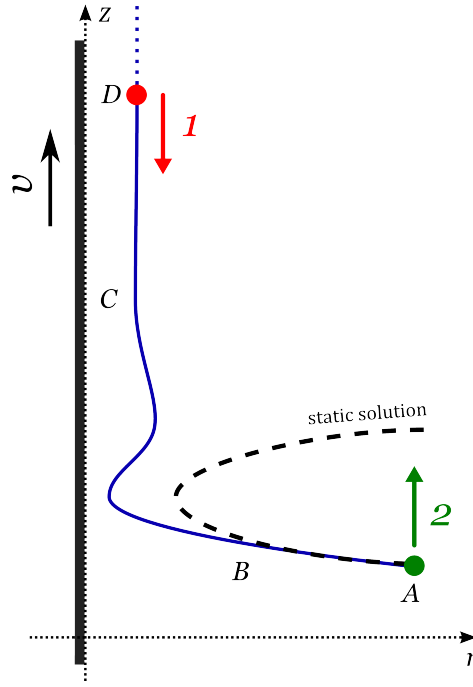
FIGURE 4.11: Schematic explaining the integration scenarios. The liquid film profile and the static meniscus are represented in blue and in dashed black respectively. The zone A - B corresponds to the matching between the static meniscus and the film solution; zone B - C is a transition zone; zone C - D is the flat film part. Numerical integration can be achieved starting from the flat film in D using the direction 1 (red), or starting from the static meniscus in A using the direction 2 (green).
