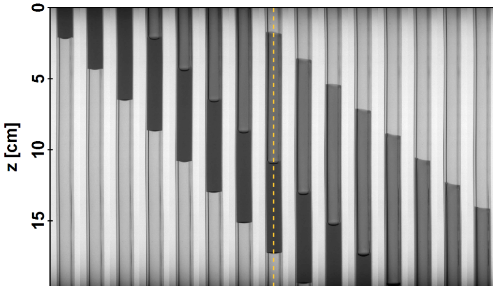
FIGURE 2.2: Image sequence of a typical experiment where a liquid film is deposited at the rear of the liquid slug (light grey). The slug appears in dark grey, V = 2 mL of dyed water. The inner diameter of the polymer tube (PVC) is d_{in} = 6.4 mm. The images are separated by a time step of \Delta t = 0.8 s.
