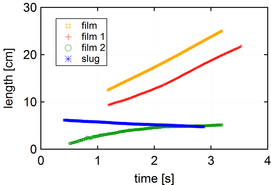
FIGURE 5.3: Slug (blue) and total film length (orange) as a function of time, measured from the image sequence shown in Figure 5.2. The film is segmented in two parts, the first film in the upper part (red) and the second film in the lower part (green). Experimental parameters are: 20%wt glycerol solution ( \eta = 1.66 \text{ mPa}\cdot\text{s} ), v = 15.8 \text{ cm}\cdot\text{s}^{-1} ( Ca = 4 \cdot 10^{-3} ). The slug decreases in length while the film grows.
