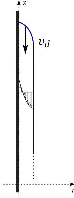
FIGURE 4.14: Schematic representation of a flat film solution with a triple line moving down a cylindrical tube up at the velocity -v_d in the reference frame of the triple line. The flow is upward close to the wall and downward close to the free surface.
