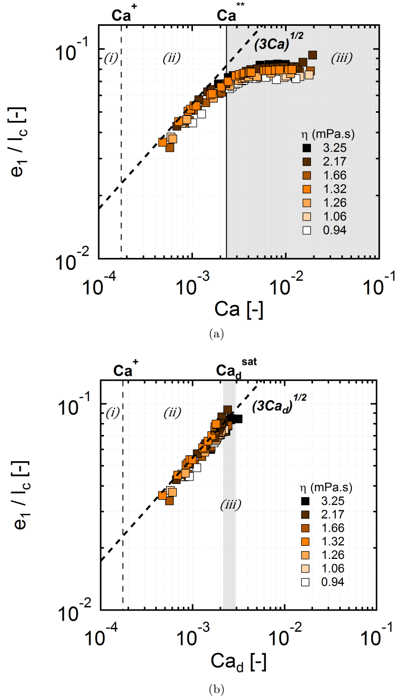
FIGURE 4.9: Average film thickness e_1 normalized by the capillary length l_c as a function of (a) the capillary number of the slug Ca , (b) the capillary number of the dewetting film Ca_d . The dashed black line is the predictive model with no adjustable parameter considering a gravitational drainage at constant film thickness.
