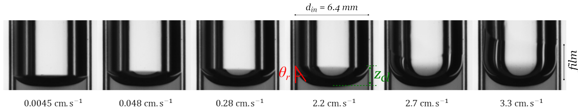
FIGURE 3.2: Images of a receding meniscus for various meniscus velocity v as indicated below each image. The tube diameter is 6.4 mm. The liquid used is 5wt% glycerol solution, \eta = 1.06 mPa.s. The meniscus elevation z_{cl} and receding contact angle \theta_r are measured for each value of v . z_{cl} increases and \theta_r decreases with increasing v . Above a threshold velocity v^* , a liquid film is entrained as observed on the last image.
