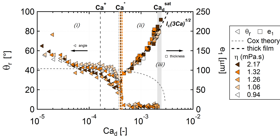
FIGURE 4.17: Receding contact angle \theta_r (left axis - triangles) and thick film thickness e_1 (right axis - squares) as a function of the capillary number of the dewetting film for various mixtures.
