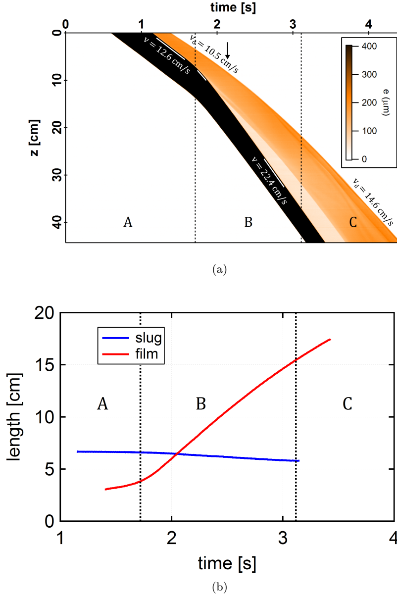
FIGURE 5.14: (a) Spatio-temporal diagram of film thickness for an experiment with water ( \eta = 0.94 \text{ mPa.s} ), where we have increased sharply the velocity of the slug during the flow. The velocity goes from 12.6 \text{ cm.s}^{-1} to 22.4 \text{ cm.s}^{-1} . (b) Corresponding slug and film length evolution with time.
