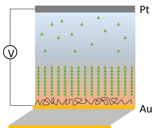
Figure 3.11 Schematic representation of the eSI-ATRP: polymer brushes are obtained by ATRP on a conducting substrate on which a polymeric macro-initiator is adsorbed. The reaction is meant possible by the catalyst gradient electrochemically generated from the surface (morphogen). Triangles represent the monomers and the Cu(I) gradient is represented by the orange gradient.
