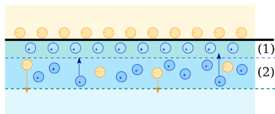
Figure 2.8: Schematic representation of the electronic double layer model: 1) Stern layer of desolvated ions behaving like a resistance and 2) Gouy-Chapman layer of heterogeneous ion composition behaving like a capacitor.
