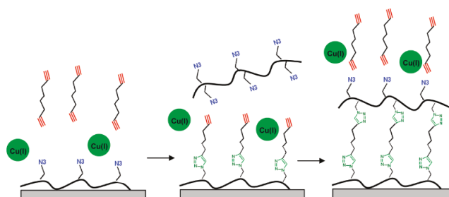
Figure 1.4 Schematic representation of the step-by-step buildup of a polymer film based on the formation of triazole by the Huisgen—Sharpleess click reaction between polymer chains bearing azide groups and a spacer bearing alkyne groups. The copper(I) catalyst of the reaction is generated by the chemical reduction of copper(II) by sodium ascorbate (El Haitami et al. 2010).
