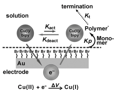
Figure 3.29 Schematic representation of polymer brushes buildup by eSI-ATRP. A gold working electrode covered with a SAM containing an ATRP initiator is brought into contact with an aqueous solution containing monomers, copper (II) chloride with the bipyridine ligand. A fixed potential is applied at the interface reducing the copper (II) complex into copper (I) thus forming the ATRP catalyst. The classical ATRP process then takes place leading to the formation of brushes (Li et al. 2012).
