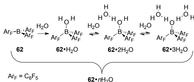
Scheme 2.20. Dynamic equilibrium between hydrated forms of B(C_6F_5)_3 .
