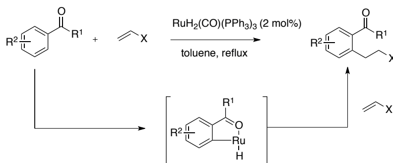
Scheme 4.2. Ru-catalyzed C-H activation with aromatic ketones and olefins.
