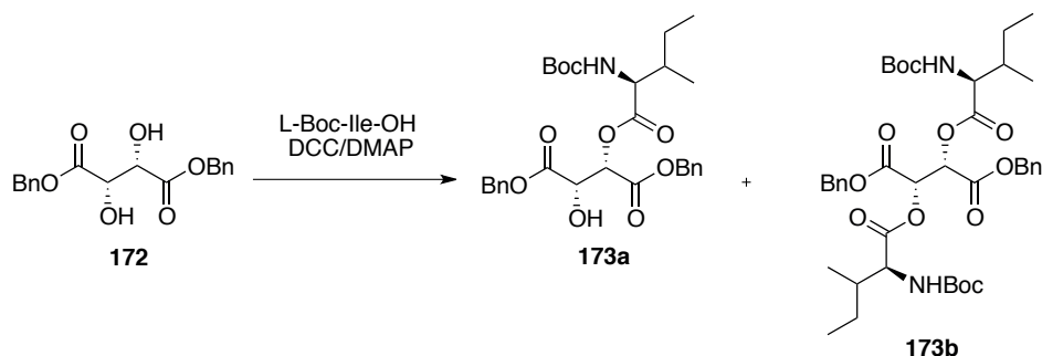
Scheme 5.7. Initial synthetic route to access tartaric acid ligand derivatives.
