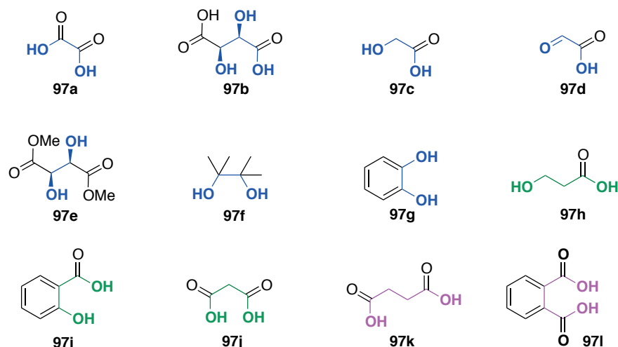
Scheme 3.6. Diverse O -ligands library. In blue, ligands forming a 5-membered ring with boronic acids; in green, ligands forming a 6-membered ring with the boronic acids; in pink, ligands forming a 7-membered ring with boronic acids.
