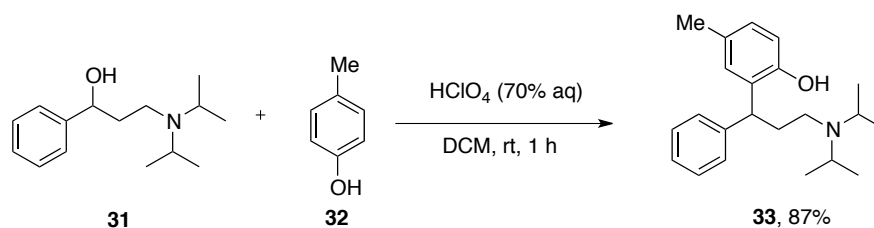
Scheme 2.3. Synthesis of rac -tolderodine involving a Friedel-Crafts reaction of a phenyl propane aminoalcohol with p -cresol.
