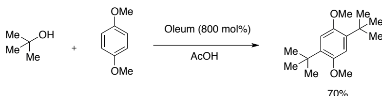
Scheme 2.23. Friedel-Crafts reaction with t BuOH in the presence of fuming sulfuric acid.
