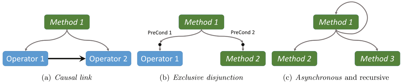
FIGURE 4.1: A method decomposition can be only operators (a), only methods (c), or a mix between them (b), and it can also be recursive (c). In (a) Operator 2 cannot be applied unless Operator 1 is applied successfully. In (b) to decompose Method 1 , either we apply Operator 1 if PreCond 1 holds (pre-condition for this decomposition) or we apply Method 2 if PreCond 2 holds, but not both at the same time even if the two pre-conditions holds at the same time. In (c) the decomposition is asynchronous: all the methods in the decomposition are applied, but are not ordered.
