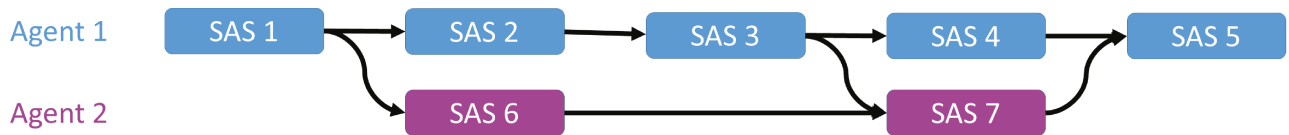
FIGURE 4.2: An example plan generated by HATP: it contains two streams, for agent 1 and agent 2, connected through causal links
