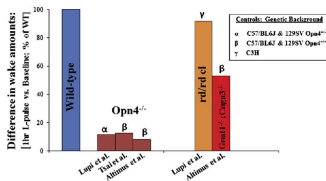
Fig. 1. Differences between studies in wake amounts during a 1-h light pulse administered at the same ZT (early part of the dark phase). Effect of a 1-h light pulse administered at ZT14, ZT15, or ZT16 on wake suppression in different transgenic mouse models (maintained under 12-h: 12-h light–dark cycle; 12 hL:12 hD). The data were extrapolated from different studies 28–30 and expressed as a deviation from their respective controls (symbols, α, β, γ, indicate the genetic background used in each of the studies) that are normalized to 100%. No s.e.m. is given nor statistics done due to the availability of the data extrapolated. Opn4 +/- represents the WT control against Opn4 -/- , however Lupi et al. used heterozygous Opn4 +/- animals as controls. Opn4 -/- melanopsin knockout; rd/rd cl: rodless coneless; Gnat1 -/- ; Cnga3 -/- : mutations in the rod transducing gene ( Gnat1 ) and the cone cyclic nucleotide-gated channel gene ( Cnga3 ) resulting in intact melanopsin-based photoreception but lack of ability of both rods and cones to detect light. 12 Wake was chosen as the output measure as Altimus et al. categorized sleep as a whole and did not distinguish between NREM and REM sleep, and though a 3-h light pulse was given during this experiment, only data from the first hour were used so as to compare with the other two studies. Percentages for Altimus have been converted into minutes/hours.
