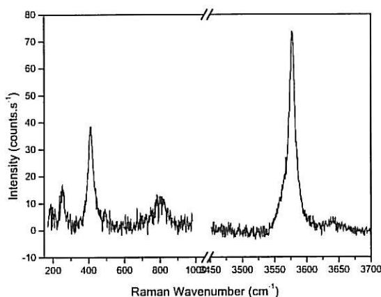
Figure II.C-1 : Spectre Raman in-situ de \text{Fe}(\text{OH})_2 - 40s - 5mW
