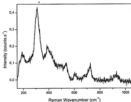
Figure II.A-7 : Spectre Raman d'akaganéite \beta\text{-FeOOH}_{1-x}\text{Cl}_x 1200s – 0,1mW
