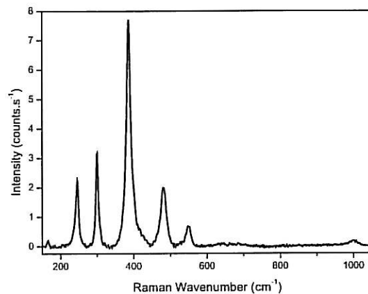
Figure II.A-4 : Spectre Raman de goethite \alpha-FeOOH 200s - 0,1mW
