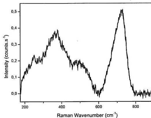
Figure II.A-6 : Spectre Raman de ferrihydrite 5\text{Fe}_2\text{O}_3 \cdot 9\text{H}_2\text{O} 10×300s – 0,1mW
