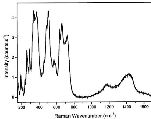
Figure II.A-2 : Spectre Raman de maghémite \gamma-Fe_2O_3 600s - 0,1mW
