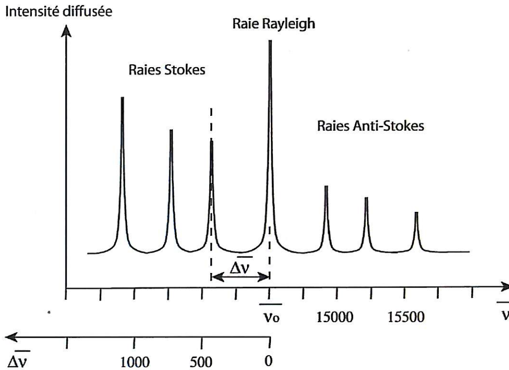
Figure I.E-2: Spectre Raman.
