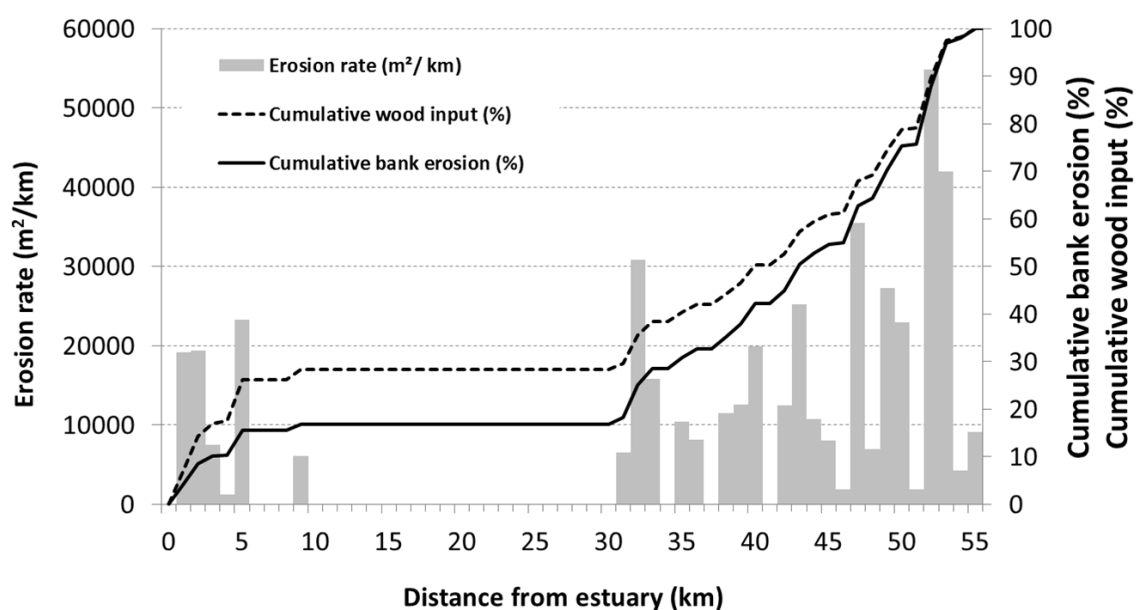
Figure 23. Longitudinal distribution of erosion rates (m 2 /km) and cumulative curves (%) for the eroded surfaces and the wood volume input into the river system.
