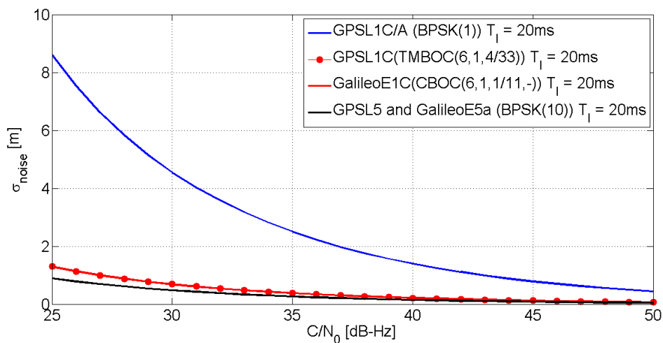
Figure 3-4: Standard deviation of the code thermal noise ranging error - T_I = 20 ms
