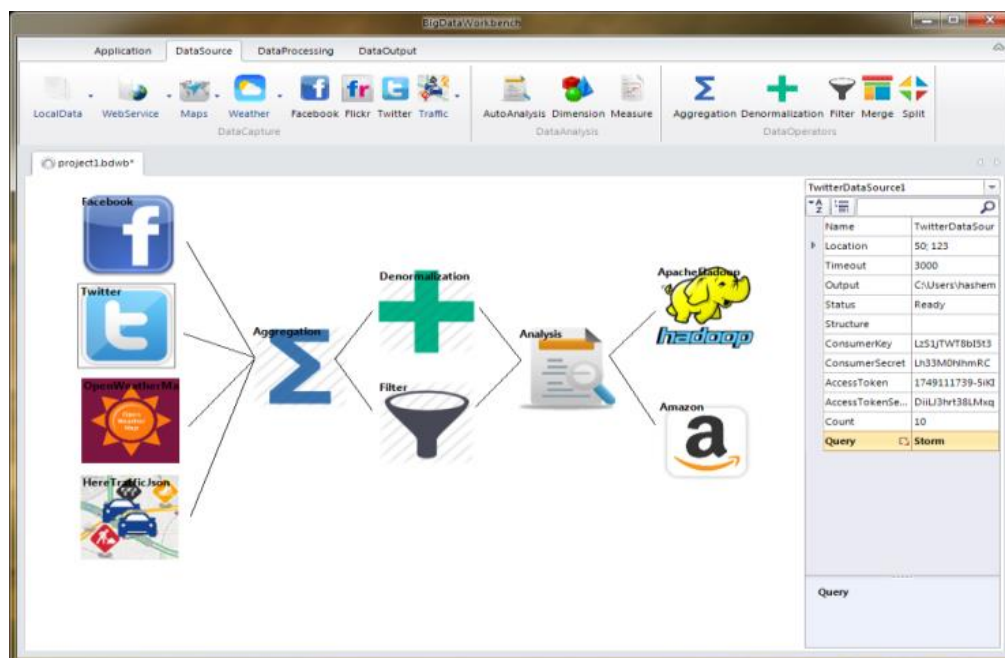
Figure 56 : BigData Workbench
