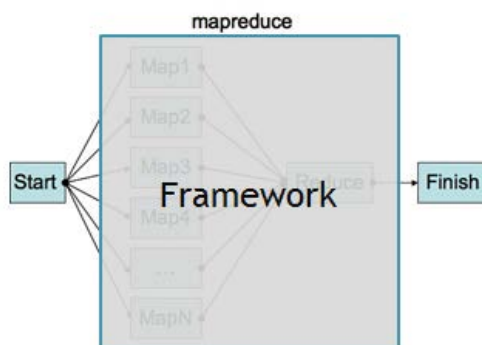
Figure 11 : Framework MapReduce
