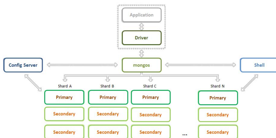
Figure 72 : Cluster MongoDB
