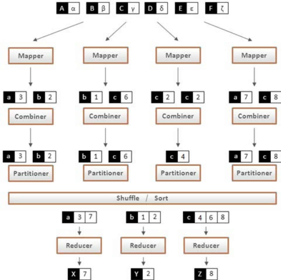
Figure 45 : Framework MapReduce
