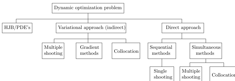
Figure 3.6: Classification of dynamic optimization solution methods [18].
