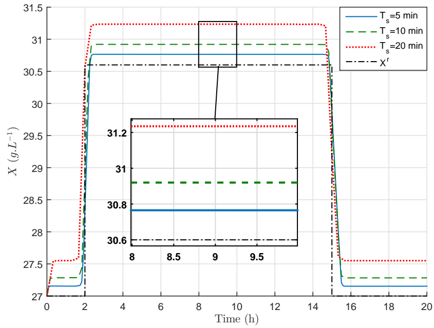
Figure 5.5: Biomass concentration evolution with time for LRMPC strategy for several values of the sampling time T_s .
