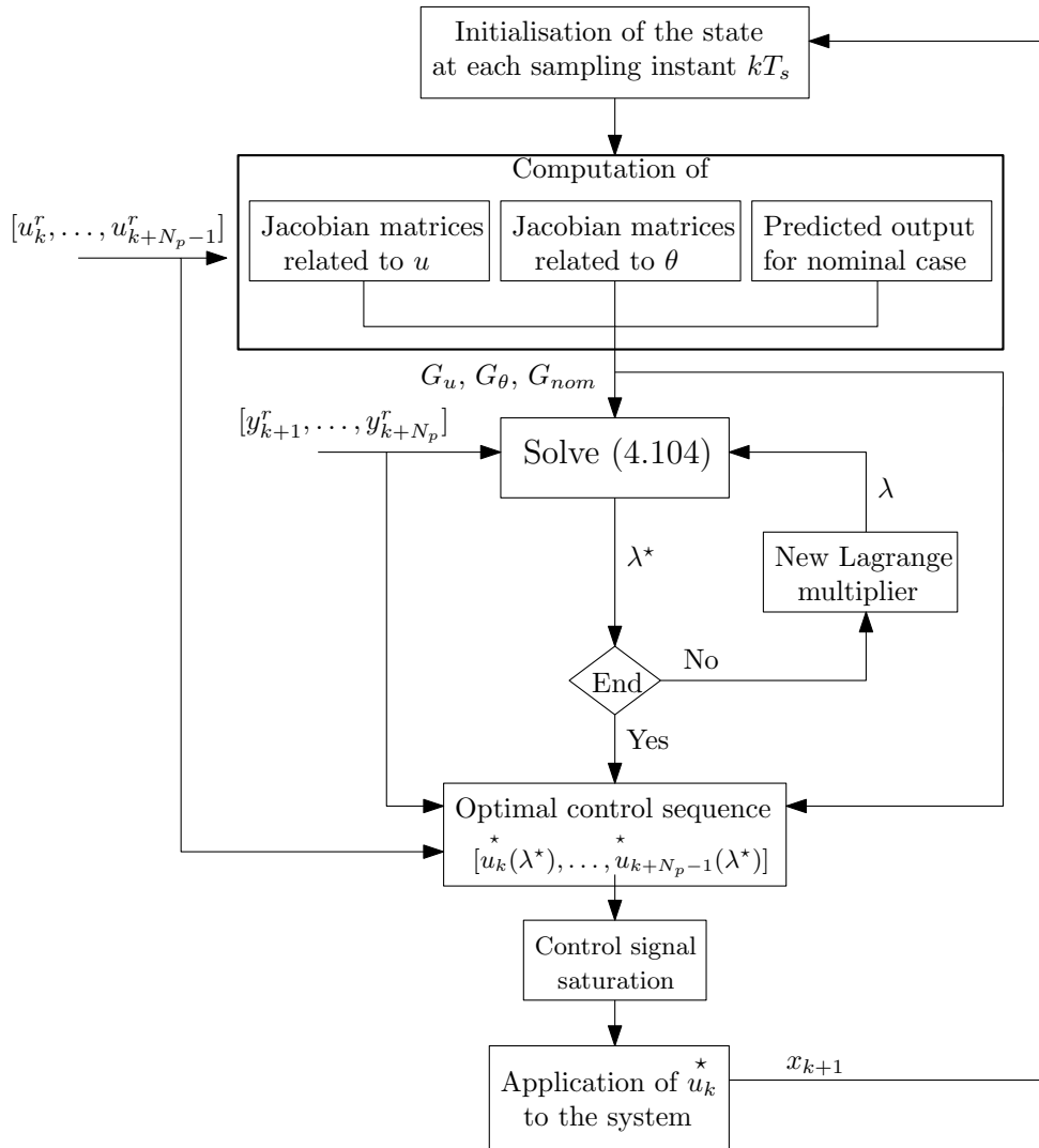
Figure 5.3: Diagram of the LRMPC algorithm.
