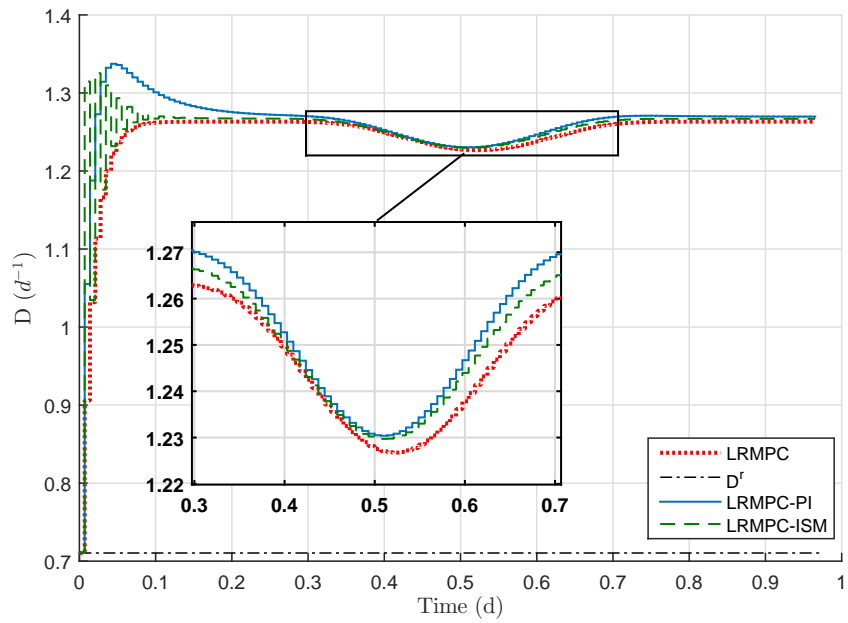
Figure 7.24: Control input evolution with time for LRMPC, LRMPC-PI and LRMPC-ISM strategies (disturbance rejection).
