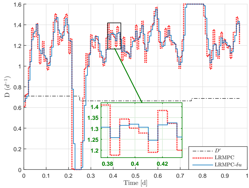
Figure 7.9: Dilution rate evolution with time for LRMPC- (\delta u) strategies.
