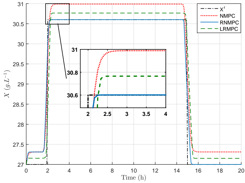
Figure 5.16: Biomass concentration evolution with time for NMPC, RN MPC and LRMPC strategies.
