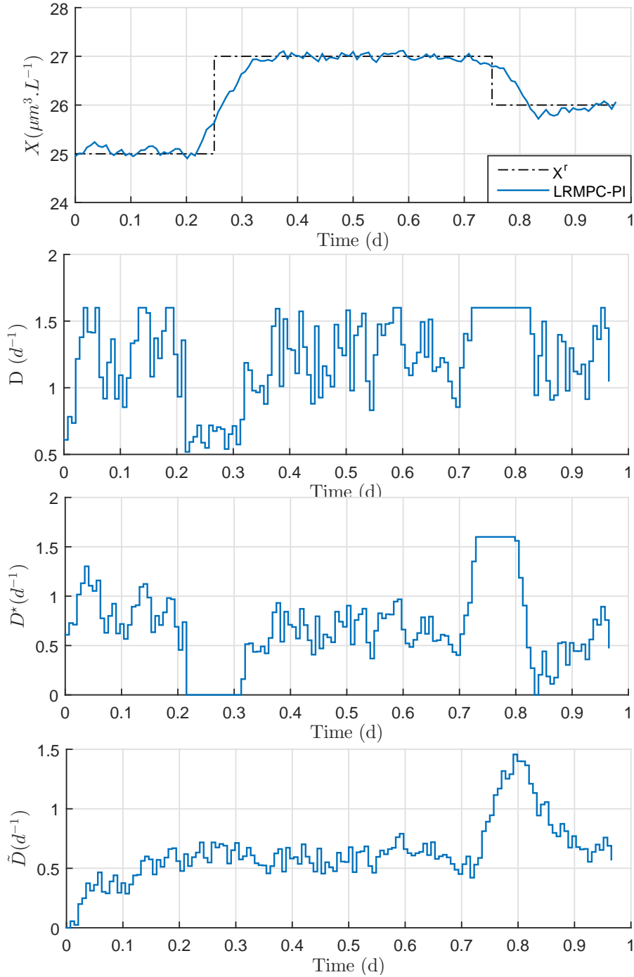
Figure 7.16: Output and control input evolution with time for LRMPC-PI strategy.
