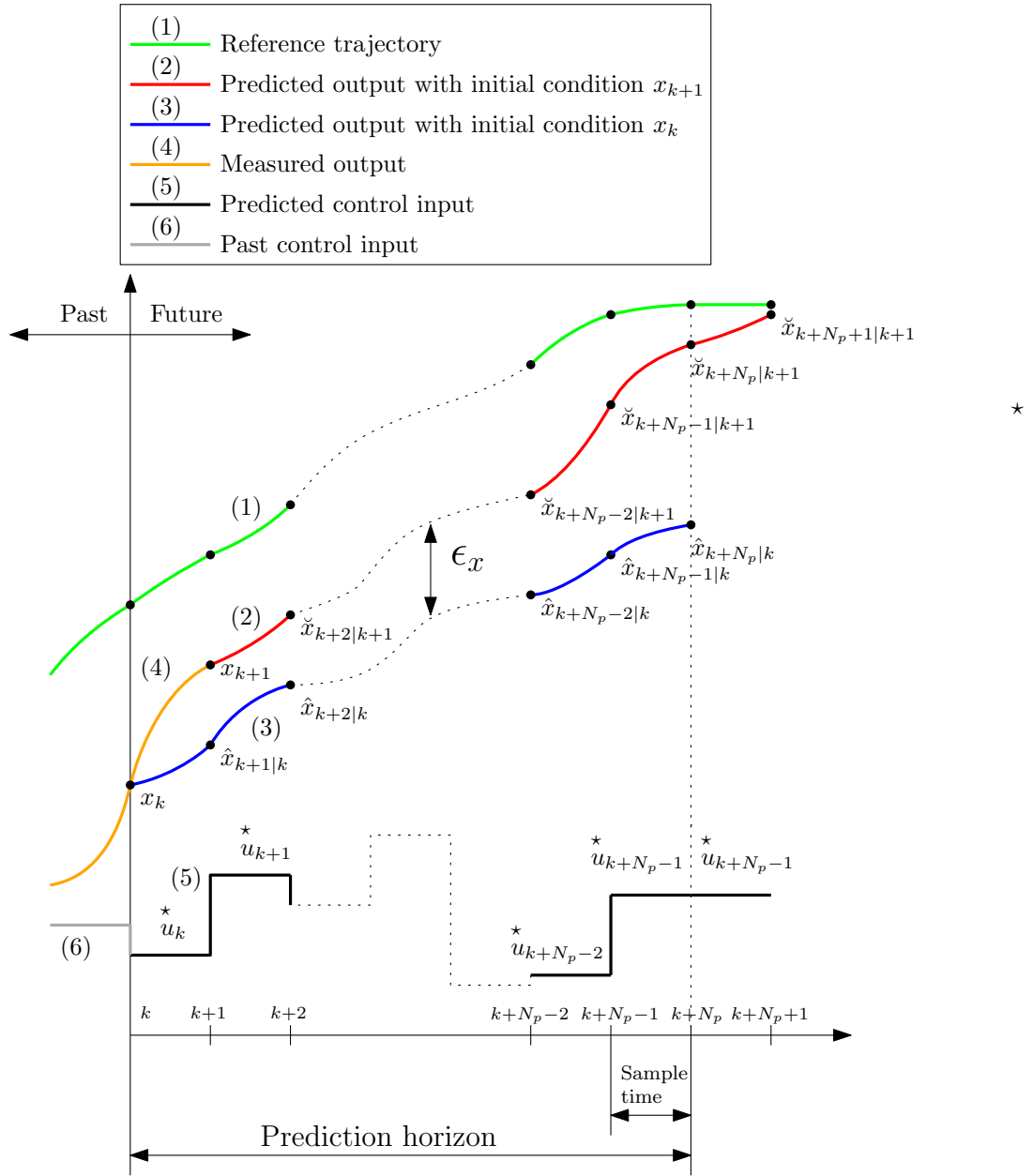
Figure 5.2: Predictions considered for the stability proof.
