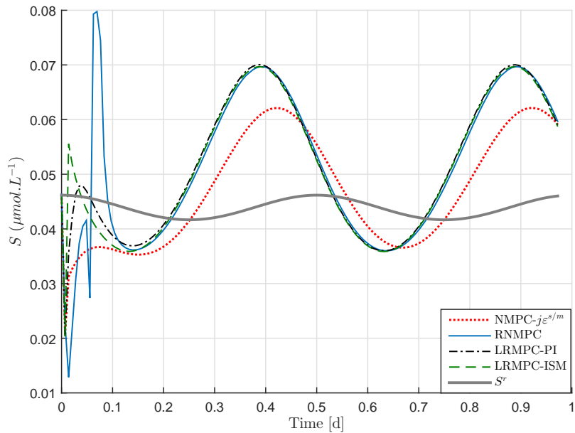
Figure 7.22: Substrate concentration evolution with time for NMPC- j\varepsilon^{s/m} , RNMPC, LRMPC-PI and LRMPC-ISM strategies in case of time varying reference trajectory.
