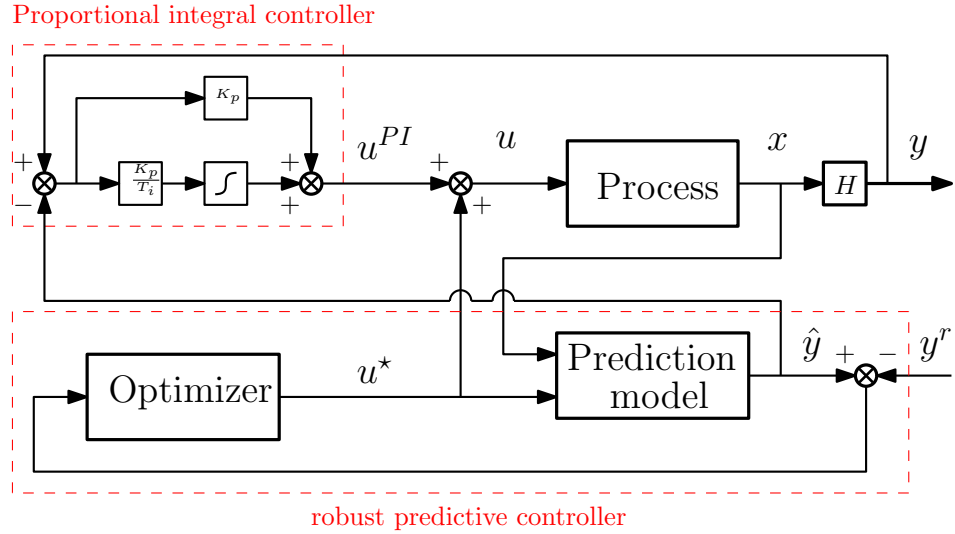
Figure 6.8: Scheme of the hierarchical control strategy based on robust MPC and PI controller.
