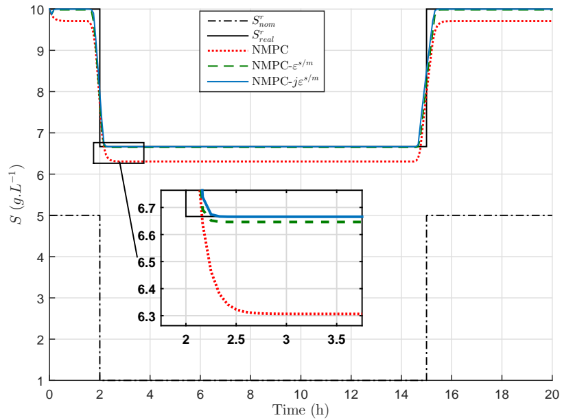
Figure 4.16: Substrate concentration evolution with time for \text{NMPC-}(j)\varepsilon^{s/m} laws in the case of parameter uncertainties.
