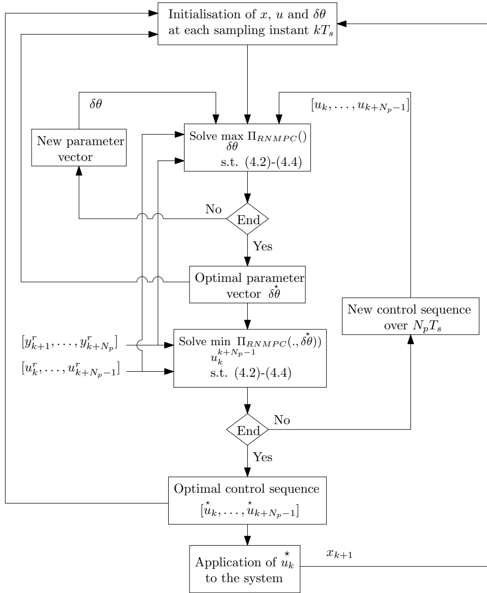
Figure 5.1: Diagram of RN MPC based on min-max optimization problem.
