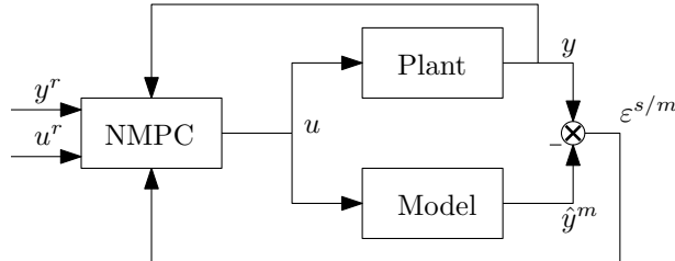
Figure 4.4: NMPC including \varepsilon^{s/m} signal.
