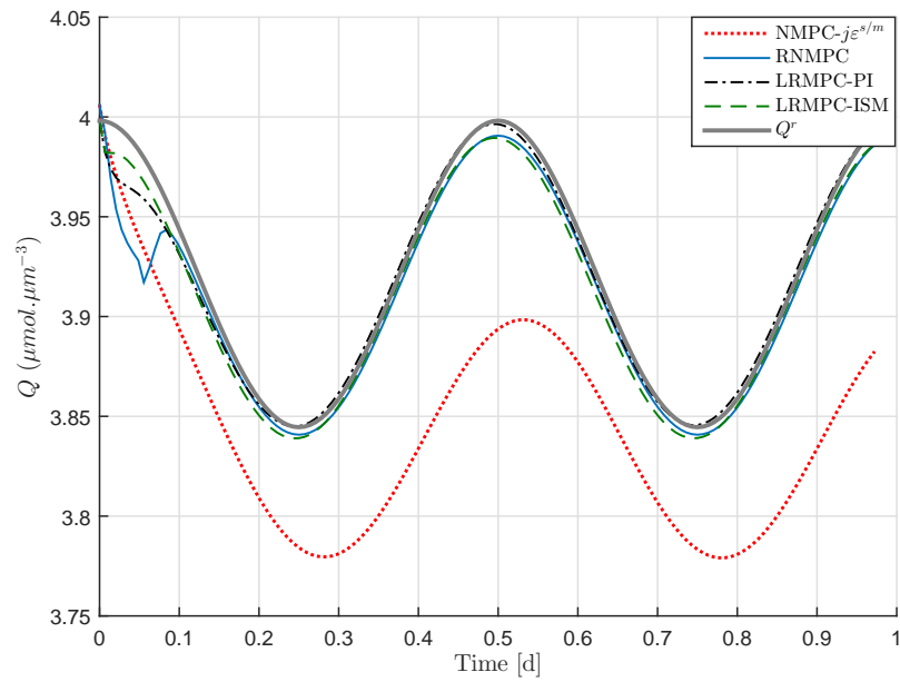
Figure 7.21: Internal quota evolution with time for NMPC- j\varepsilon^{s/m} , RNMPC, LRMPC-PI and LRMPC-ISM strategies in case of time varying reference trajectory.
