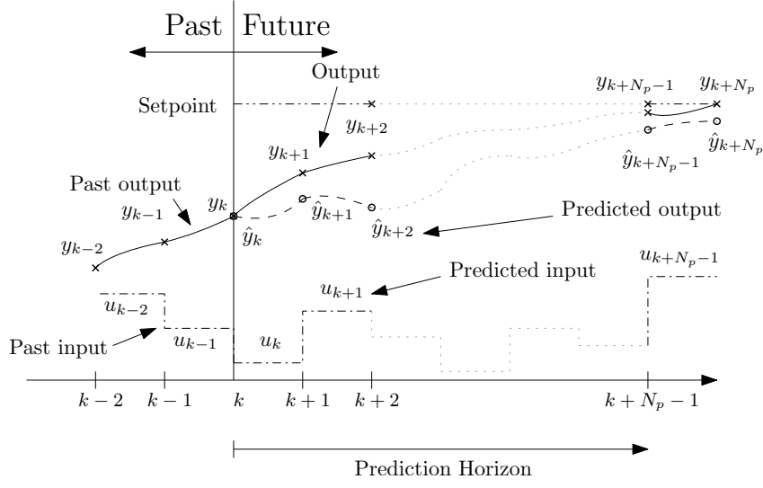
Figure 4.2: Principle of the NMPC (SISO case).
