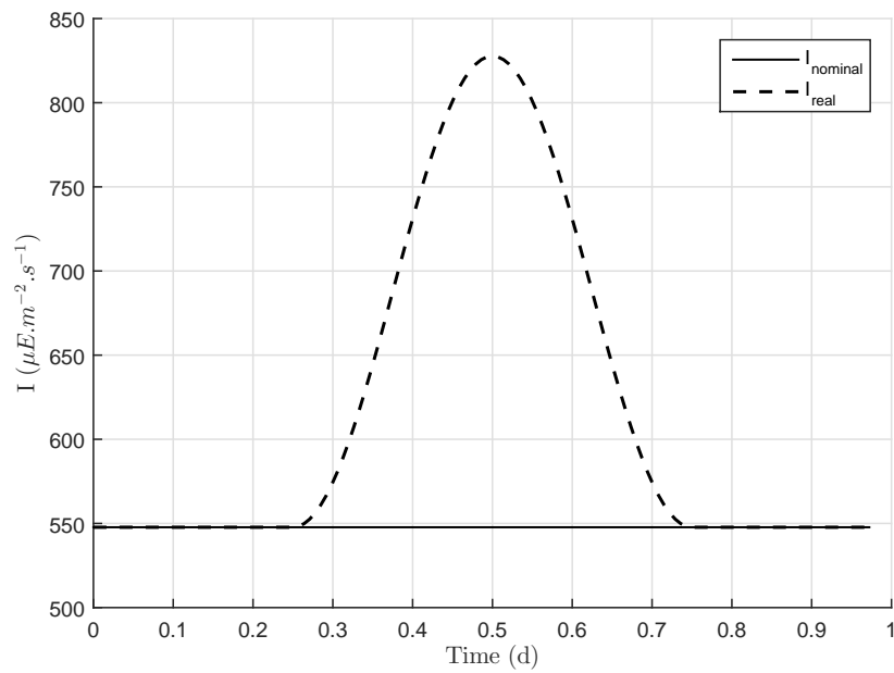
Figure 7.25: Light intensity evolution with time for LRMPC, LRMPC-PI and LRMPC-ISM strategies (disturbance rejection).
