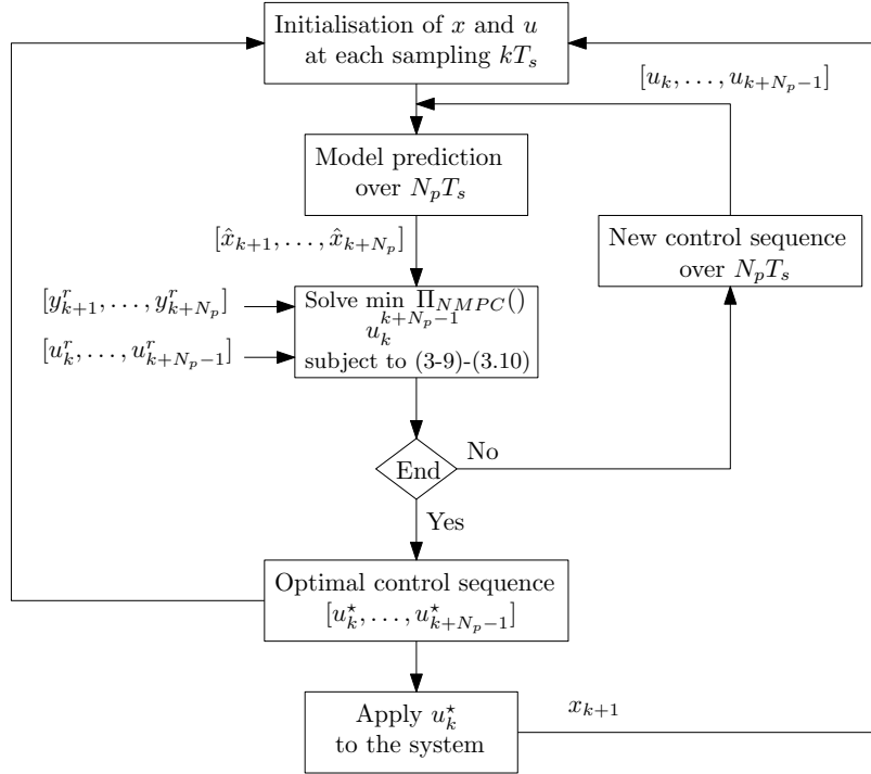
Figure 4.3: Diagram of the NMPC algorithm.
