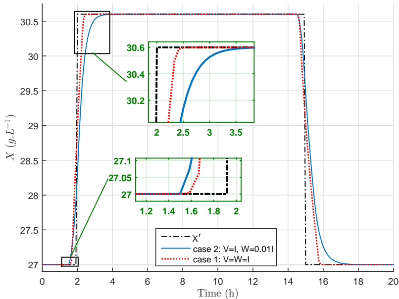
Figure 4.12: Influence of the weighting matrices on the biomass concentration evolution with time for NMPC law.
