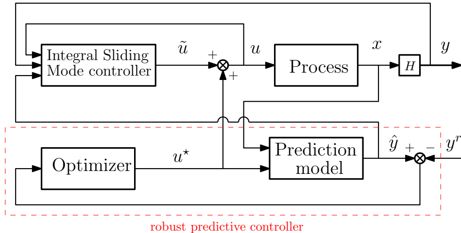
Figure 6.9: Scheme of the hierarchical control strategy based on robust MPC and ISM controller.
