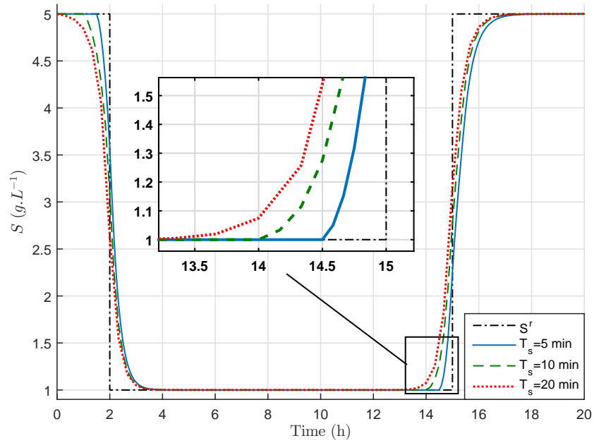
Figure 4.7: Influence of the sampling time T_s on the behavior of the substrate concentration for NMPC law.
