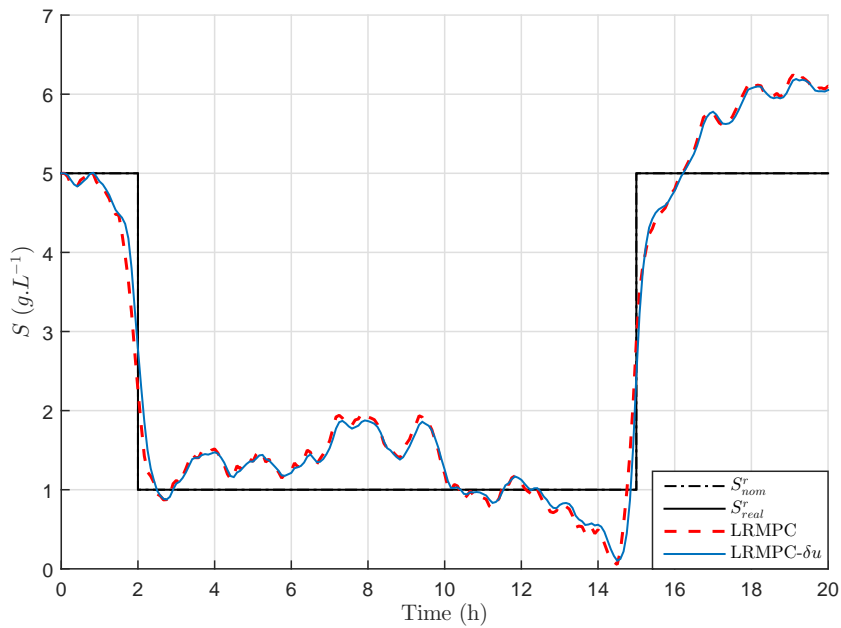
Figure 6.2: Substrate concentration evolution with time for LRMPC and LRMPC- \delta u strategies (nominal case).
