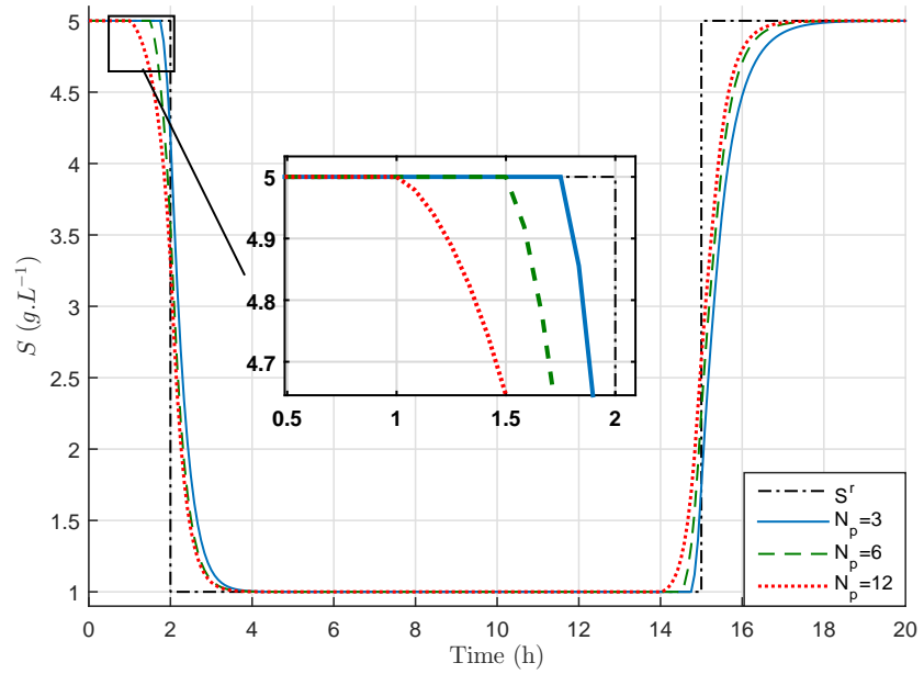
Figure 4.10: Influence of the prediction horizon N_p on the behavior of the substrate concentration for NMPC law.
