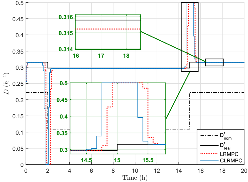
Figure 5.15: Control input evolution with time for (C)LRMPC strategies.
