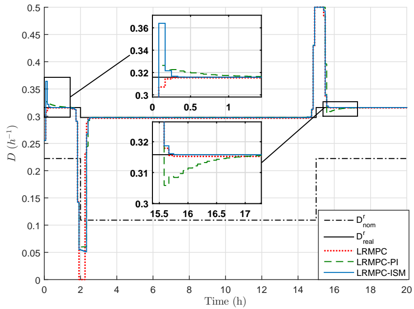
Figure 6.12: Control input evolution with time for LRMPC, LRMPC-PI and LRMPC-ISM strategies.
