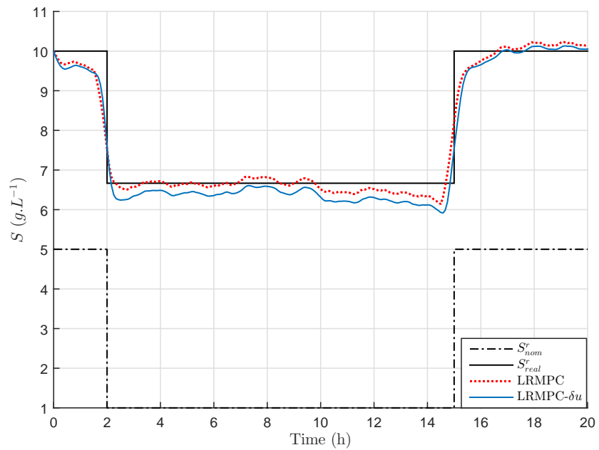
Figure 6.5: Substrate concentration evolution with time for LRMPC and LRMPC- \delta u strategies (mismatched parameters).
