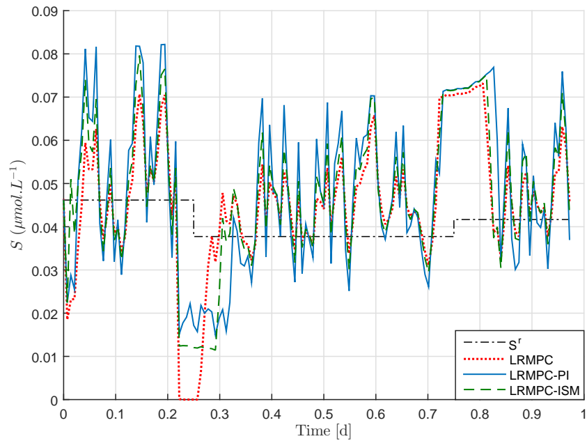
Figure 7.15: Temporal evolution of substrate concentration for LRMPC, LRMPC-PI and LRMPC-ISM strategies.
