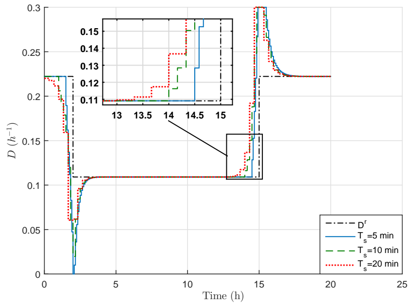
Figure 4.8: Influence of the sampling time T_s on the behavior of the control input for NMPC law.
