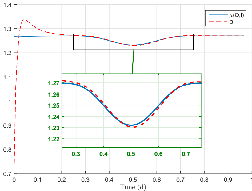
Figure 7.26: Growth rate and dilution rate evolution for LRMPC-PI strategy (disturbance rejection).
