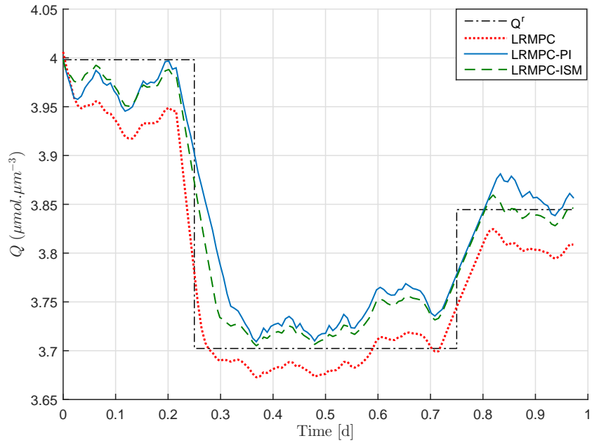
Figure 7.14: Temporal evolution of internal quota for LRMPC, LRMPC-PI and LRMPC-ISM strategies.
