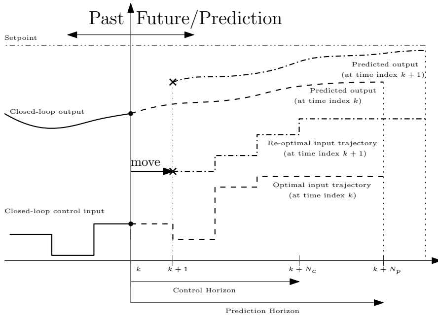
Figure 3.2: Receding horizon principle: the basic idea (SISO case).
