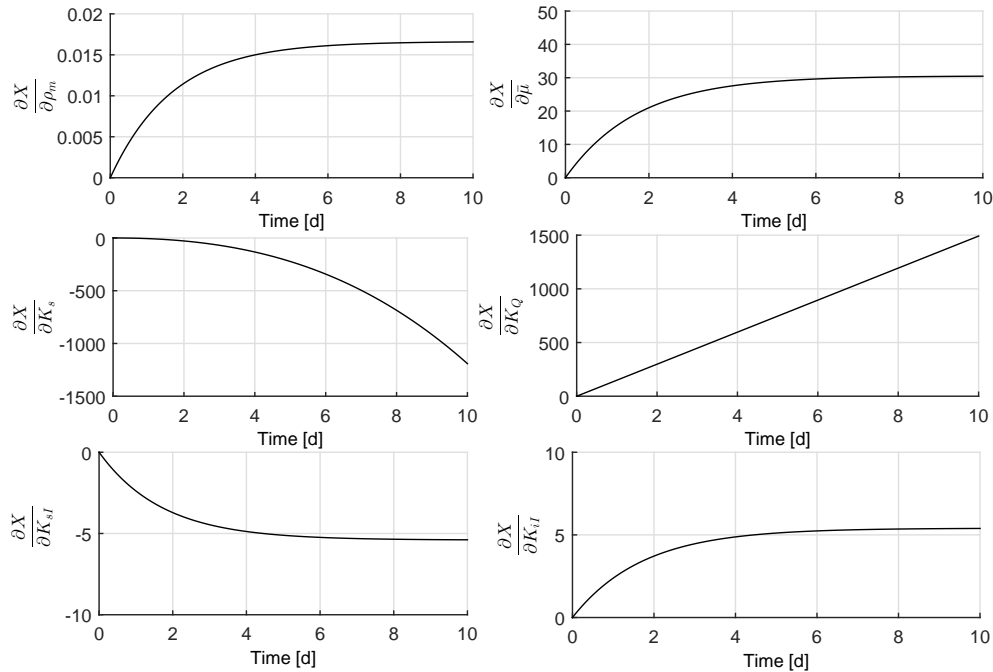
Figure C.1: Evolution of the scaled sensitivity functions (for biomass concentration).
