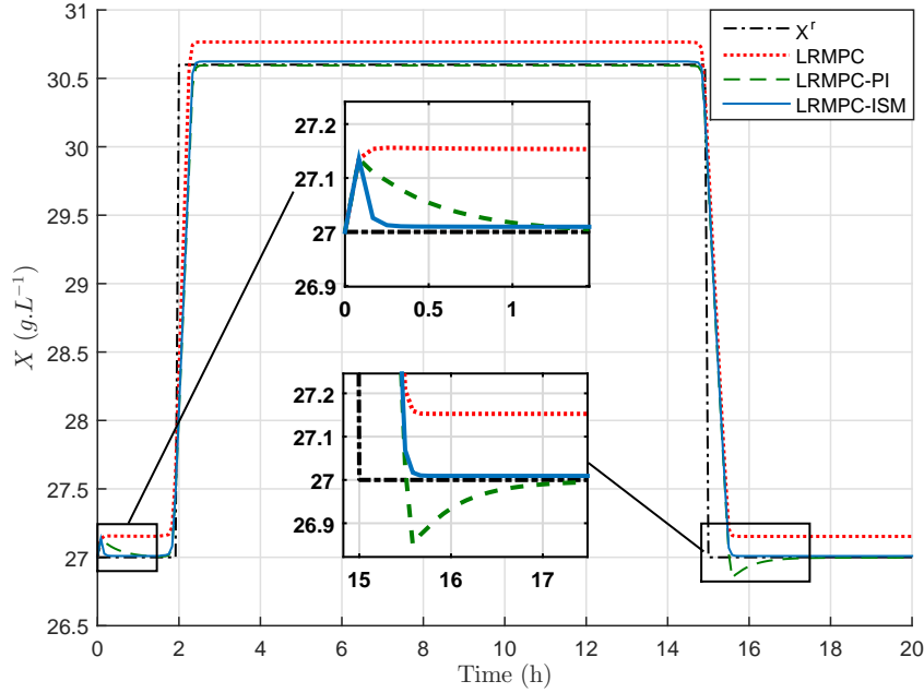
Figure 6.10: Biomass concentration evolution with time for LRMPC, LRMPC-PI and LRMPC-ISM strategies.
