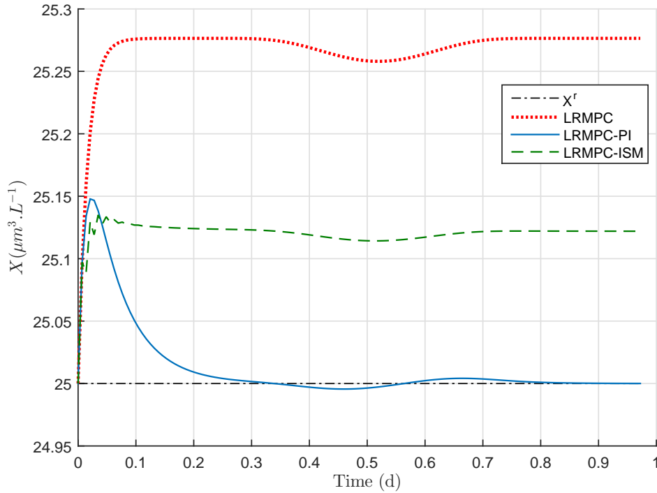
Figure 7.23: Biomass concentration evolution with time for LRMPC, LRMPC-PI and LRMPC-ISM strategies (disturbance rejection).
