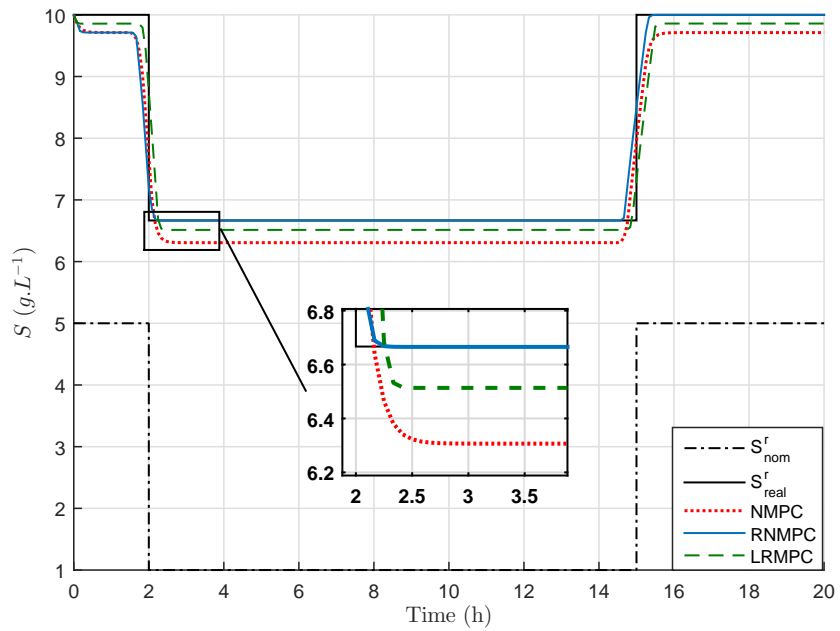
Figure 5.17: Substrate concentration evolution with time for NMPC, RN MPC and LRMPC strategies.
