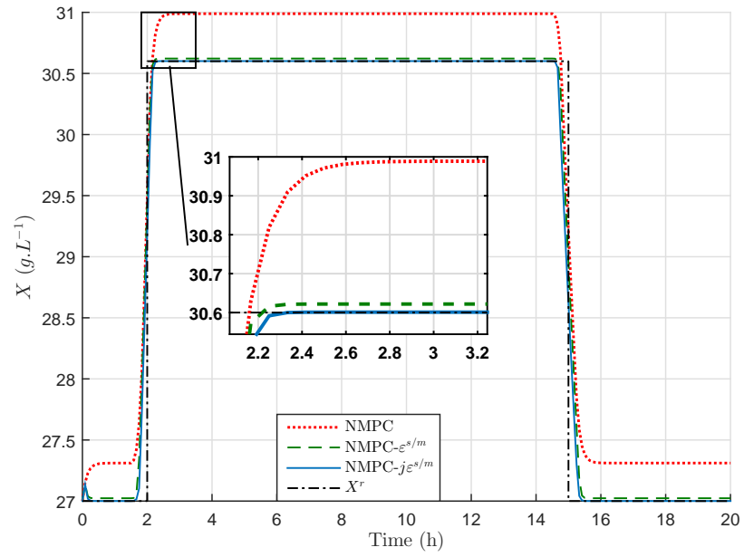
Figure 4.15: Biomass concentration evolution with time for \text{NMPC-}(j)\varepsilon^{s/m} laws in the case of parameter uncertainties.
