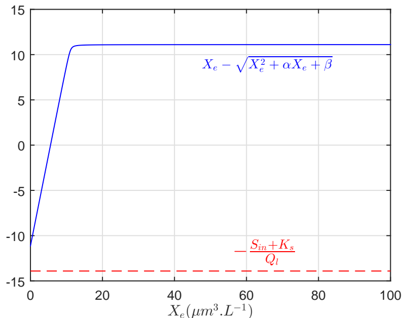
Figure 7.1: Graphical representation of the condition (7.26).
