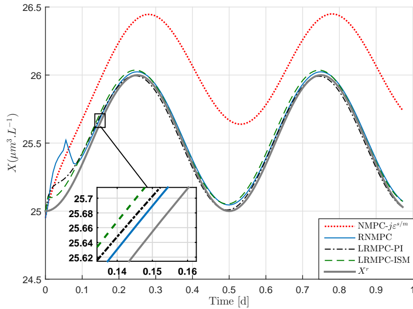
Figure 7.19: Biomass concentration evolution with time for NMPC- j\varepsilon^{s/m} , RNMPC, LRMPC-PI and LRMPC-ISM strategies in case of time varying reference trajectory.
