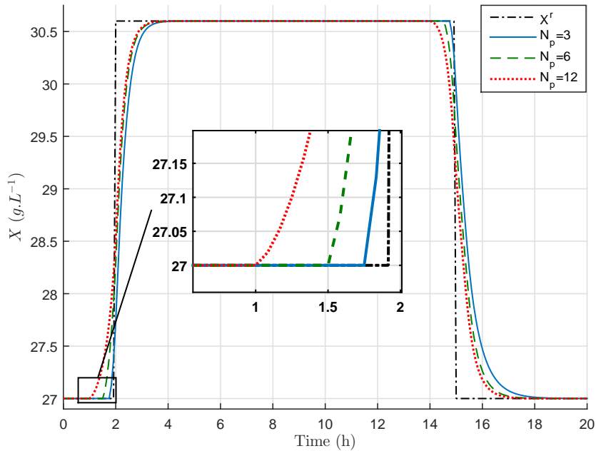
Figure 4.9: Influence of the prediction horizon N_p on the behavior of the biomass concentration for NMPC law.
