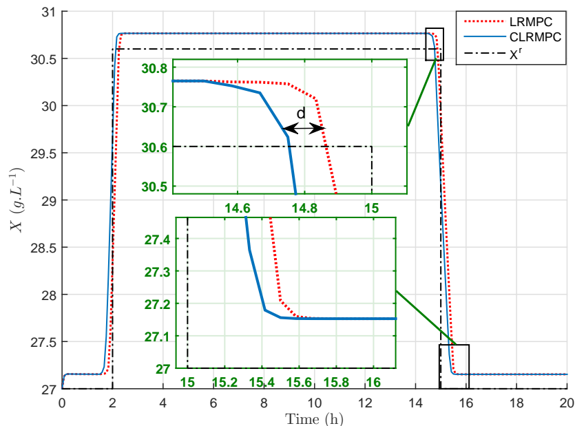
Figure 5.13: Biomass concentration evolution with time for (C)LRMPC strategies.
