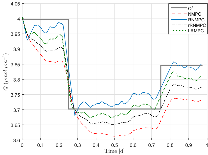
Figure 7.6: Internal quota evolution with time for NMPC, RNMPC, rRNMPC and LRMPC strategies.
