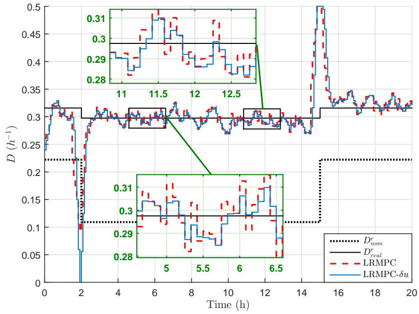
Figure 6.6: Control input evolution with time for LRMPC and LRMPC- \delta u strategies (mismatched parameters).
