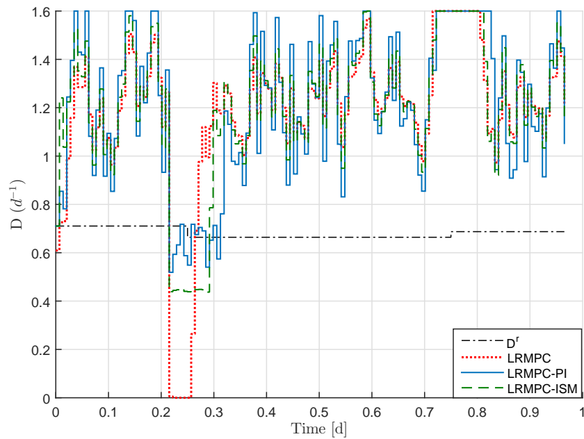
Figure 7.13: Temporal evolution of dilution rate for LRMPC, LRMPC-PI and LRMPC-ISM strategies.
