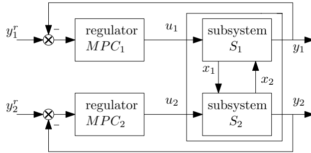
Figure 3.4: Decentralized MPC architecture [34].
