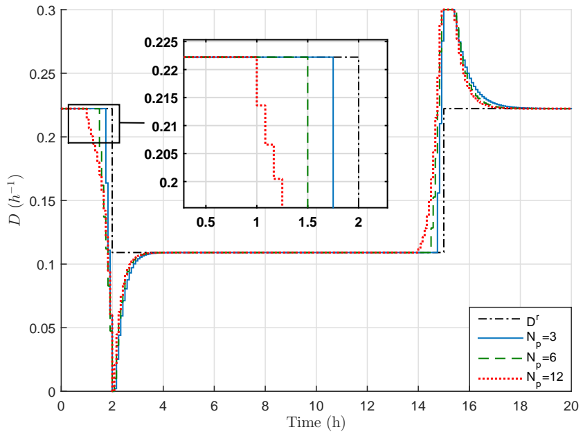
Figure 4.11: Influence of the prediction horizon N_p on the behavior of the control input for NMPC law.
