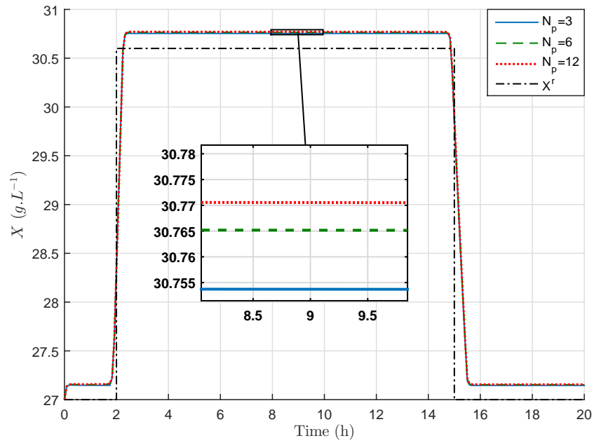
Figure 5.9: Biomass concentration evolution with time for LRMPC strategy for several values of the prediction horizon N_p .
