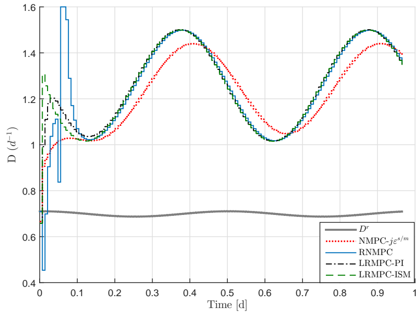
Figure 7.20: Dilution rate evolution with time for NMPC- j\varepsilon^{s/m} , RN MPC, LR MPC-PI and LR MPC-ISM strategies in case of time varying reference trajectory.
