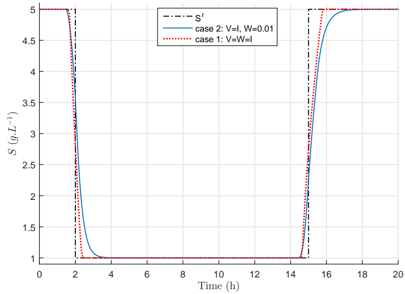
Figure 4.13: Influence of the weighting matrices on the substrate concentration evolution with time for NMPC law.
