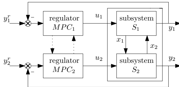
Figure 3.5: Distributed MPC architecture [34].
