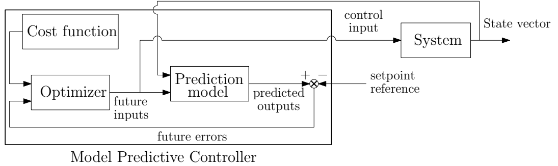
Figure 3.1: Structure of the Model Predictive Control strategy.
