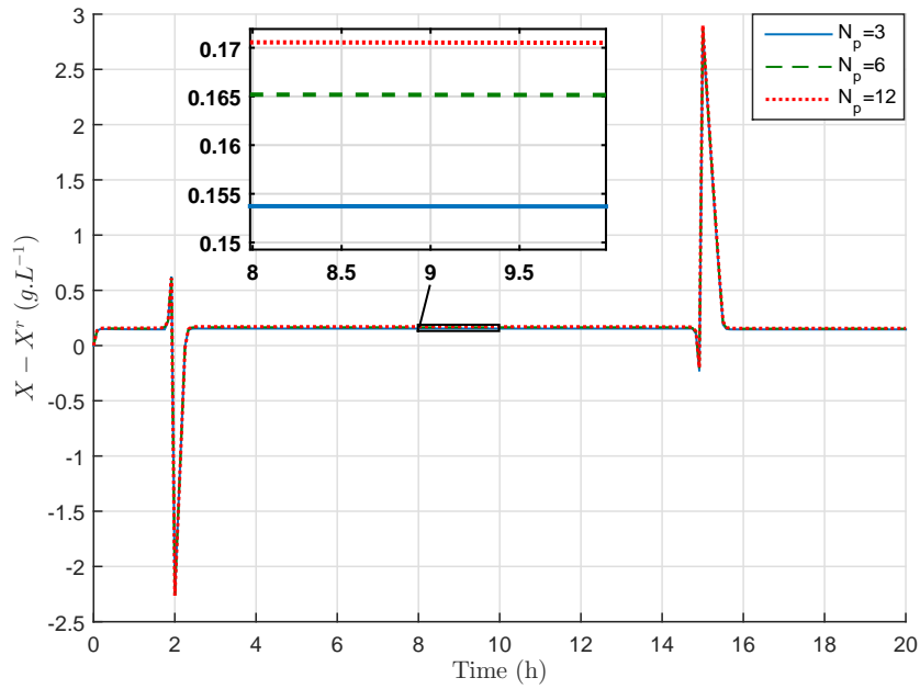
Figure 5.11: Tracking error evolution with time for LRMPC strategy for several values of the prediction horizon N_p .
