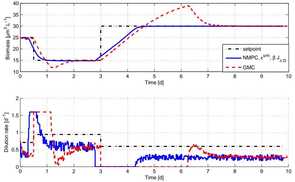
Figure C.2: Evolution of biomass concentration and dilution rate with measurement affected by noise, GMC and NMPC- \varepsilon^{s/m} laws.
