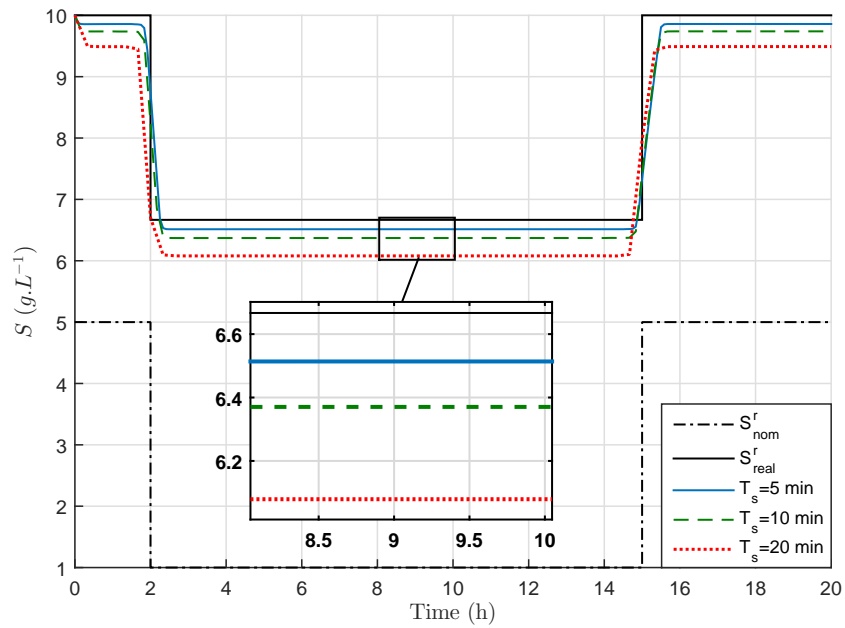
Figure 5.6: Substrate concentration evolution with time for LRMPC strategy for several values of the sampling time T_s .
