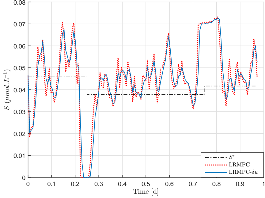
Figure 7.11: Substrate concentration evolution with time for LRMPC- (\delta u) strategies.
