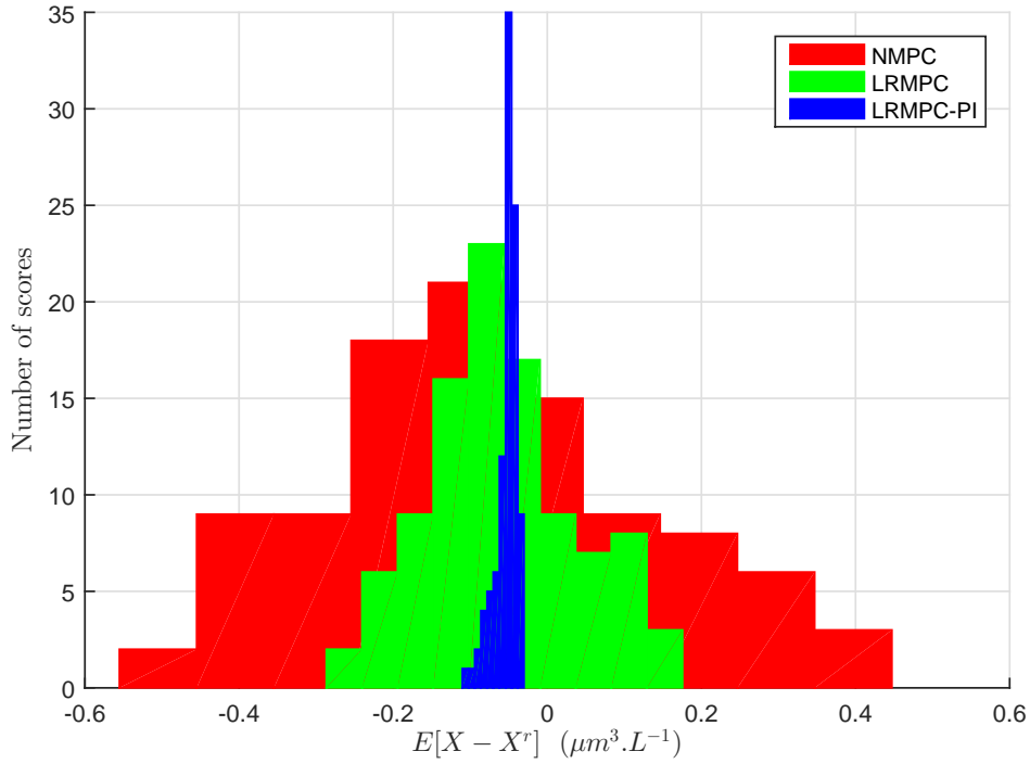
Figure 7.18: Histogram of the average tracking error for simultaneous random non correlated variation in all the parameters (Monte-Carlo).
