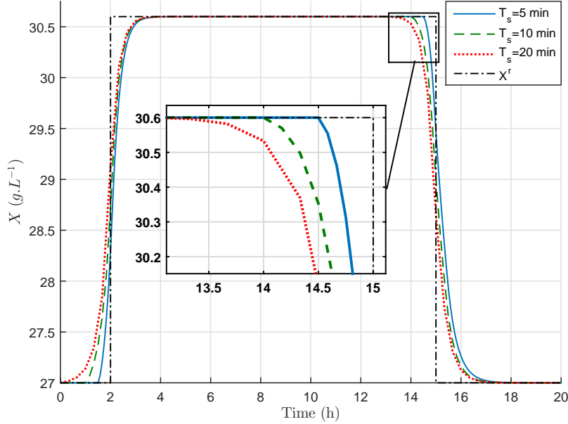
Figure 4.6: Influence of the sampling time T_s on the behavior of the biomass concentration for NMPC law.
