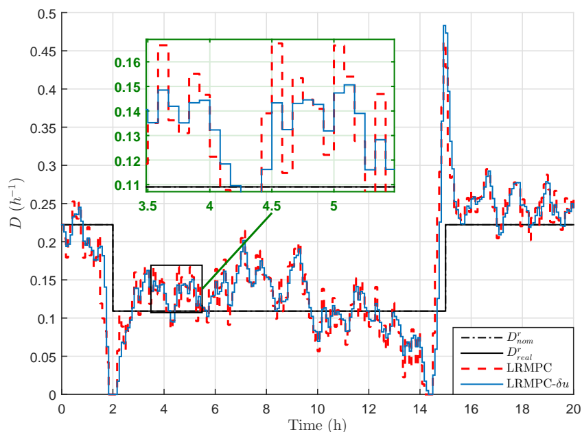
Figure 6.3: Control input evolution with time for LRMPC and LRMPC- \delta u strategies (nominal case).
