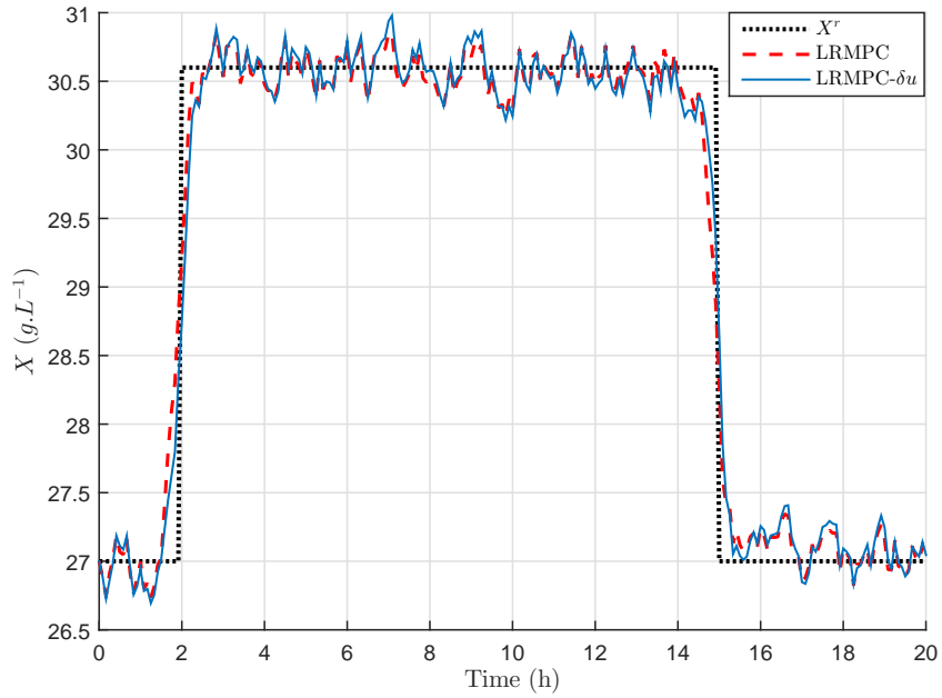
Figure 6.1: Biomass concentration evolution with time for LRMPC and LRMPC- \delta u strategies (nominal case).
