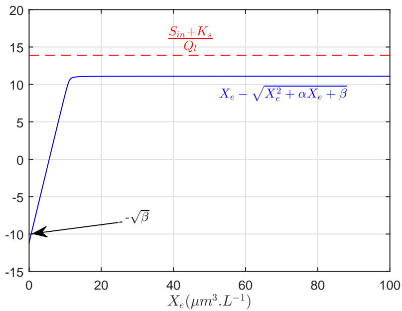
Figure 7.3: Graphical representation of the condition (7.29).
