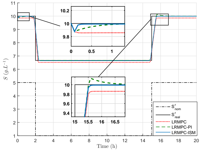
Figure 6.11: Substrate concentration evolution with time for LRMPC, LRMPC-PI and LRMPC-ISM strategies.
