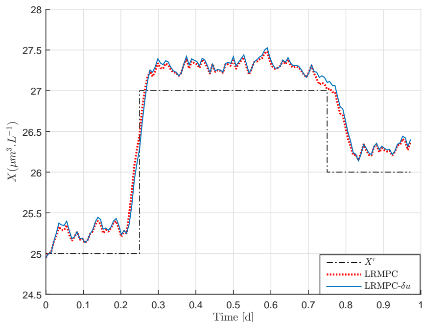
Figure 7.8: Biomass concentration evolution with time for LRMPC- (\delta u) strategies.
