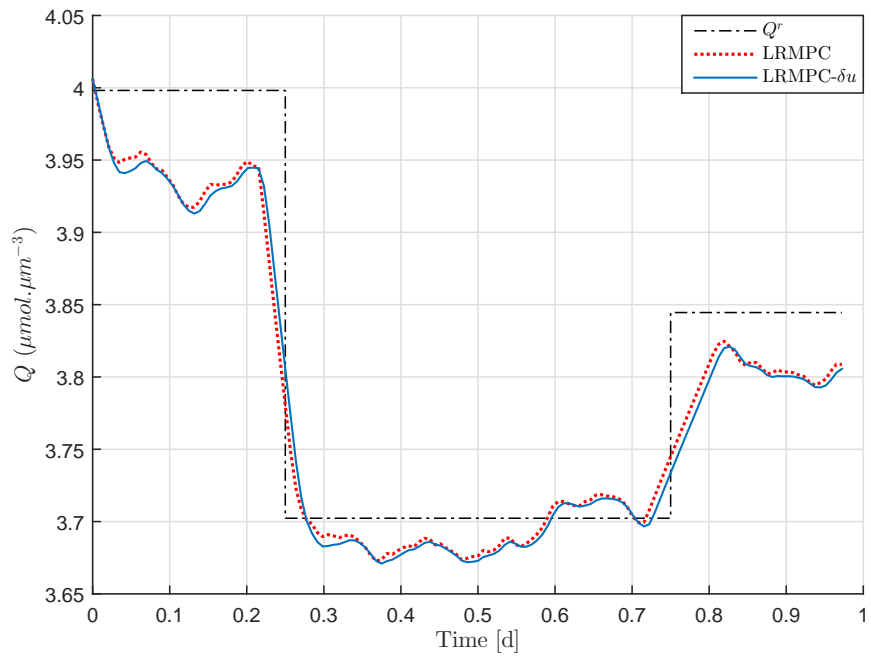
Figure 7.10: Internal quota evolution with time for LRMPC- (\delta u) strategies.
