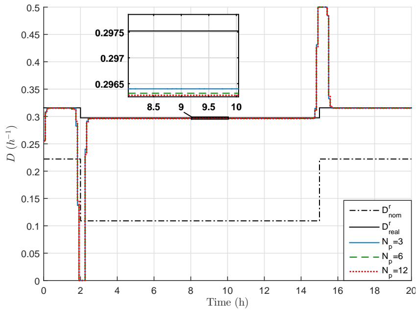
Figure 5.12: Control input evolution with time for LRMPC strategy for several values of the prediction horizon N_p .
