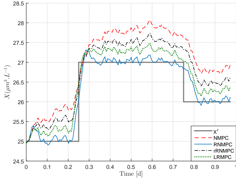
Figure 7.4: Biomass concentration evolution with time for NMPC, RNMPC, rRNMPC and LRMPC strategies.
