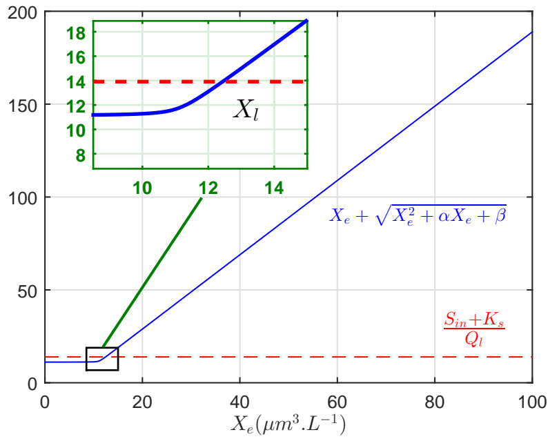
Figure 7.2: Graphical representation of the condition (7.28).
