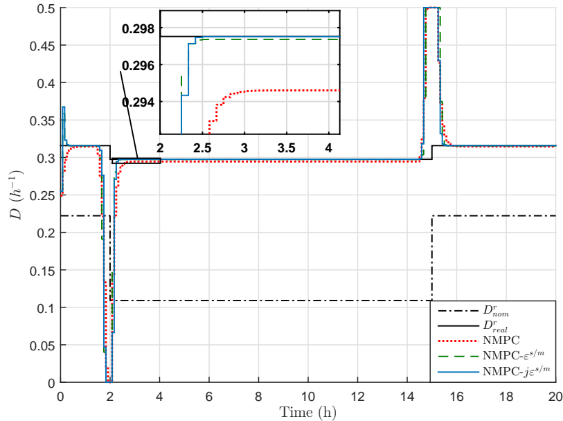
Figure 4.17: Control input evolution with time for \text{NMPC-}(j)\varepsilon^{s/m} laws in the case of parameter uncertainties.
