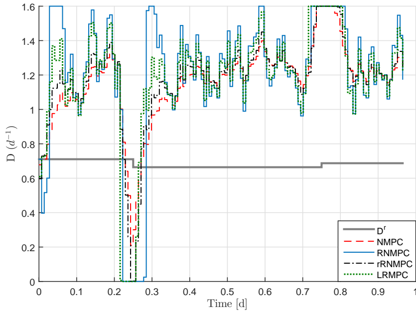
Figure 7.5: Dilution rate evolution with time for NMPC, RNMPC, rRNMPC and LRMPC strategies.
