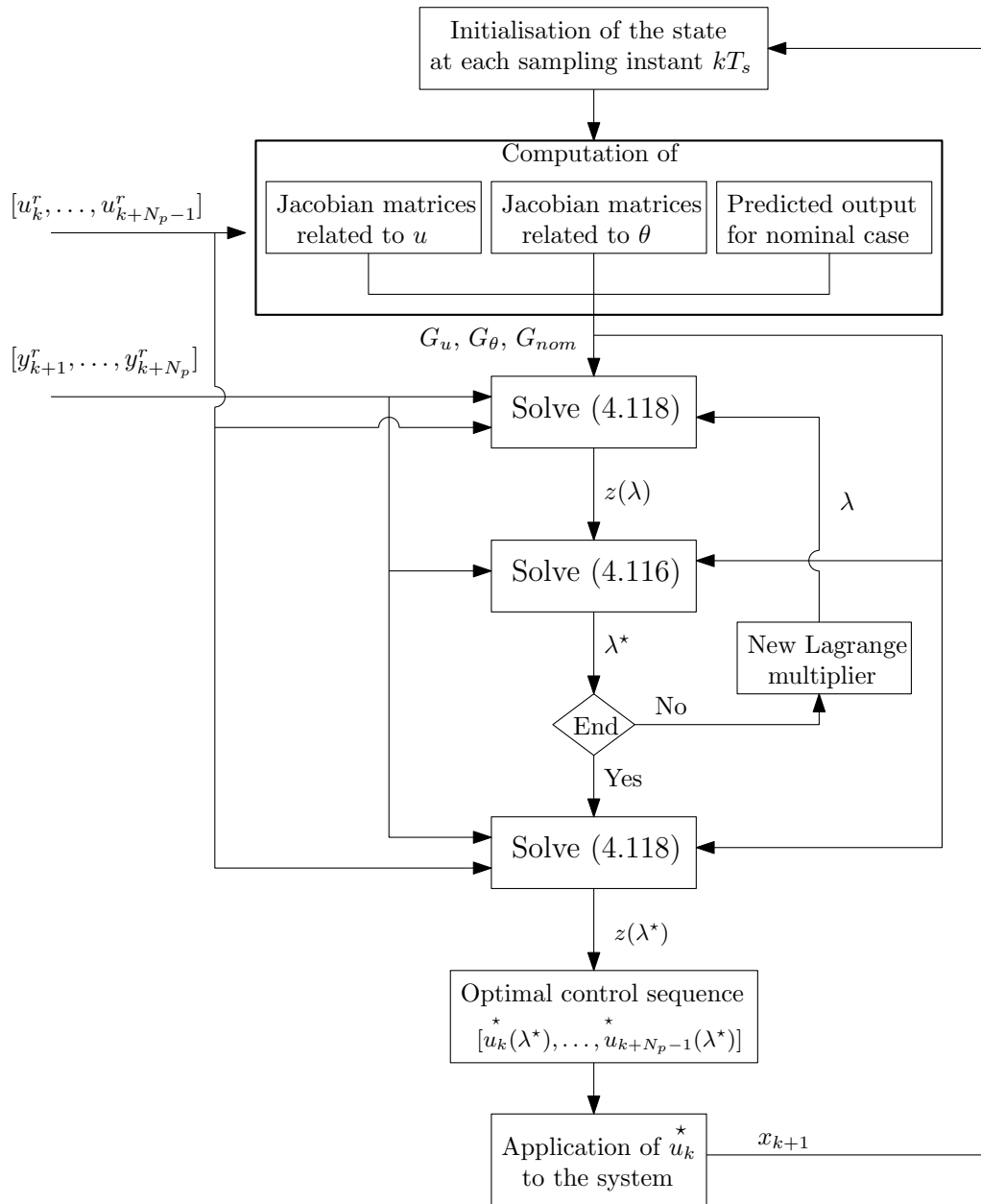
Figure 5.4: Diagram of the CLRMPC algorithm.
