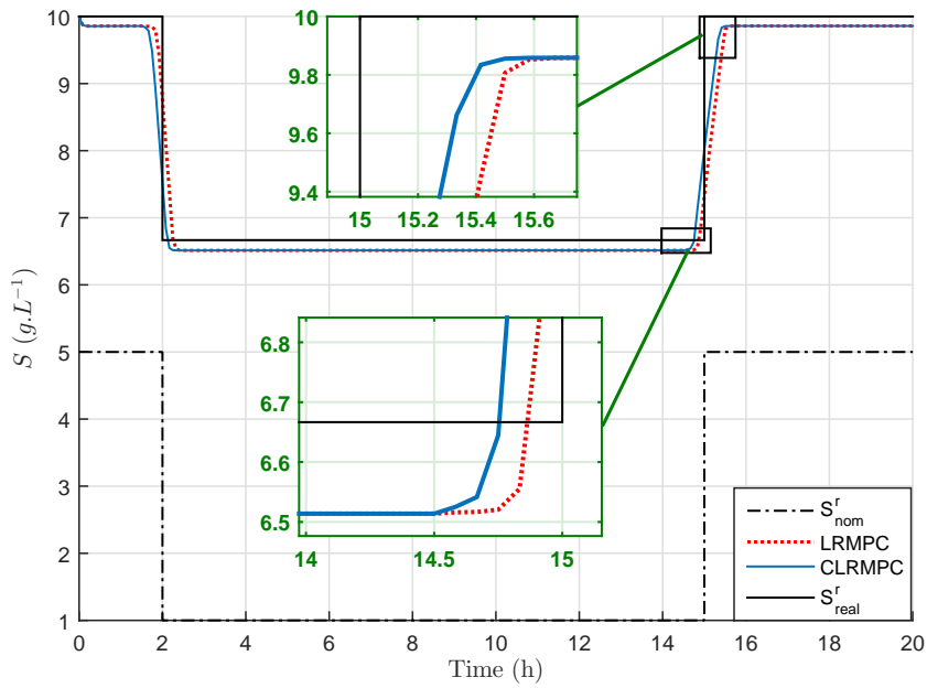
Figure 5.14: Substrate concentration evolution with time for (C)LRMPC strategies.
