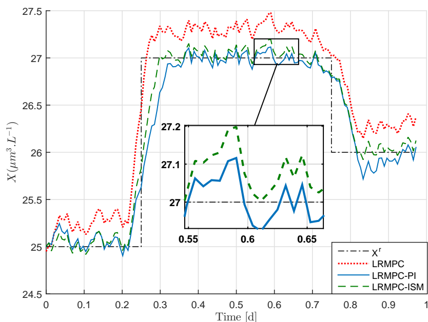
Figure 7.12: Temporal evolution of biomass concentration for LRMPC, LRMPC-PI and LRMPC-ISM strategies.
