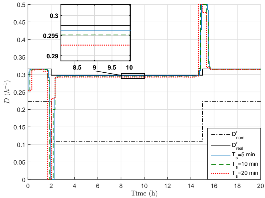
Figure 5.8: Control input evolution with time for LRMPC strategy for several values of the sampling time T_s .
