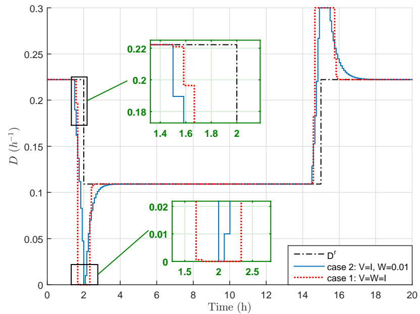
Figure 4.14: Influence of the weighting matrices on the control input evolution with time for NMPC law.
