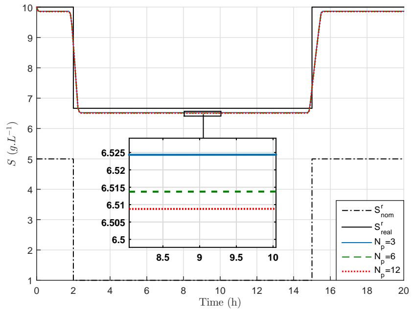
Figure 5.10: Substrate concentration evolution with time for LRMPC strategy for several values of the prediction horizon N_p .
