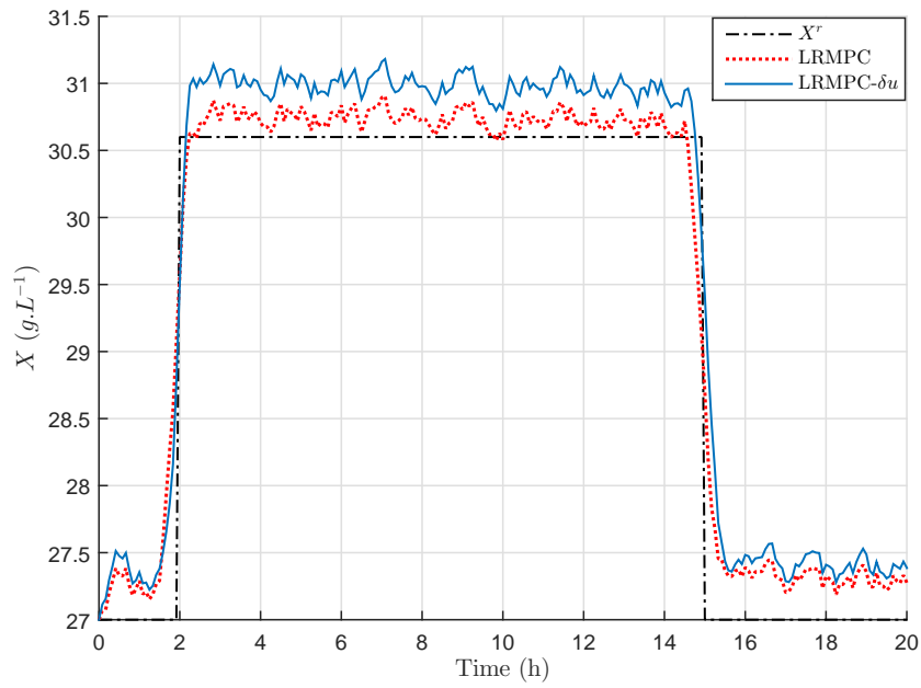
Figure 6.4: Biomass concentration evolution with time for LRMPC and LRMPC- \delta u strategies (mismatched parameters).
