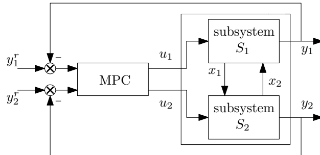
Figure 3.3: Centralized MPC architecture [34].
