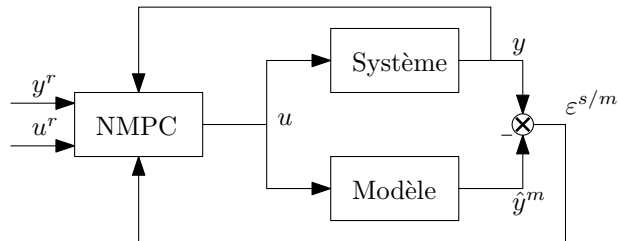
FIGURE 1.5 – CPNL incluant le signal \varepsilon^{s/m} .
