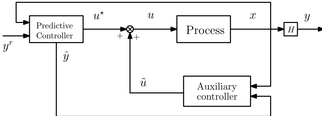
Figure 6.7: Scheme of the hierarchical control strategy [131].
