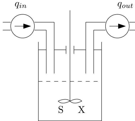
Figure 4.5: Schematic representation of a bioreactor.
