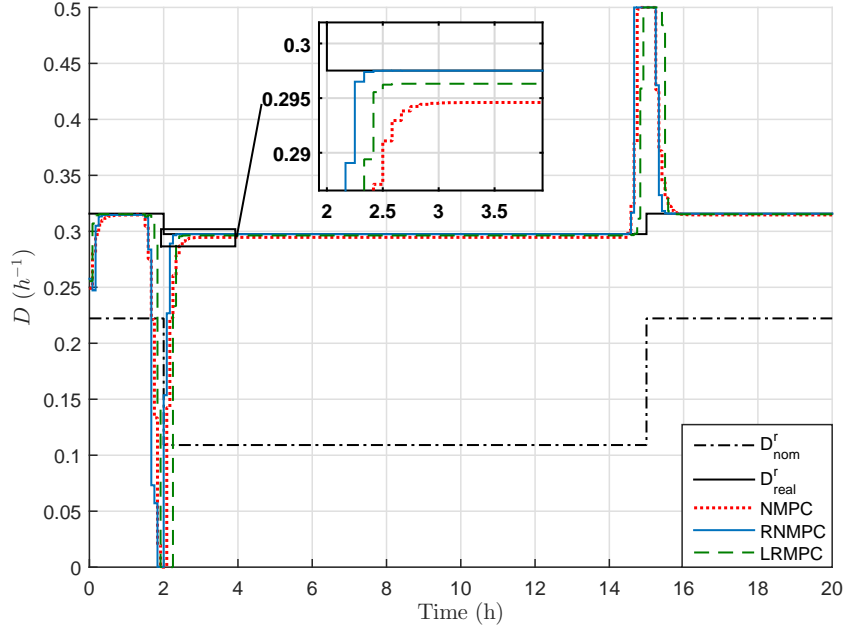
Figure 5.18: Control input evolution with time for NMPC, RNMPC and LRMPC strategies.
