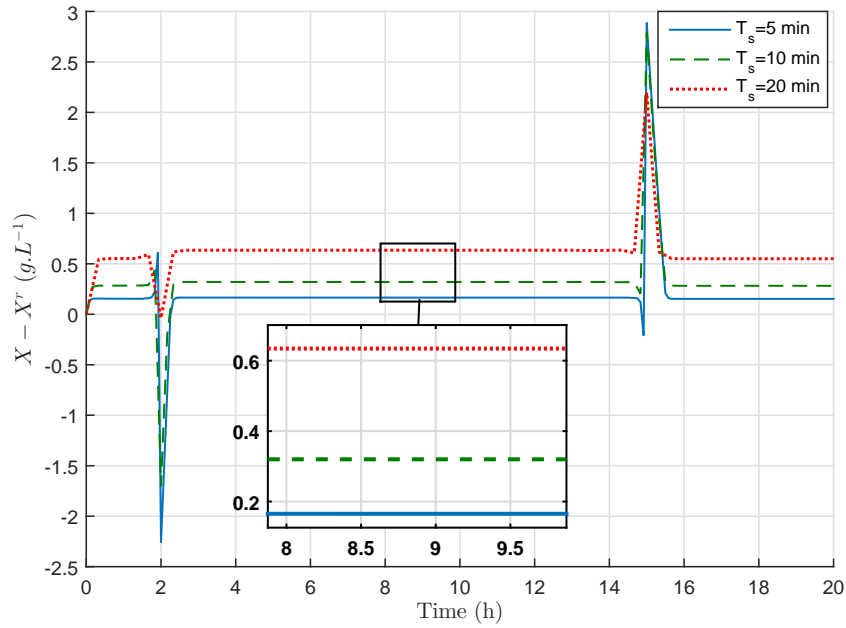
Figure 5.7: Tracking error evolution with time for LRMPC strategy for several values of the sampling time T_s .
