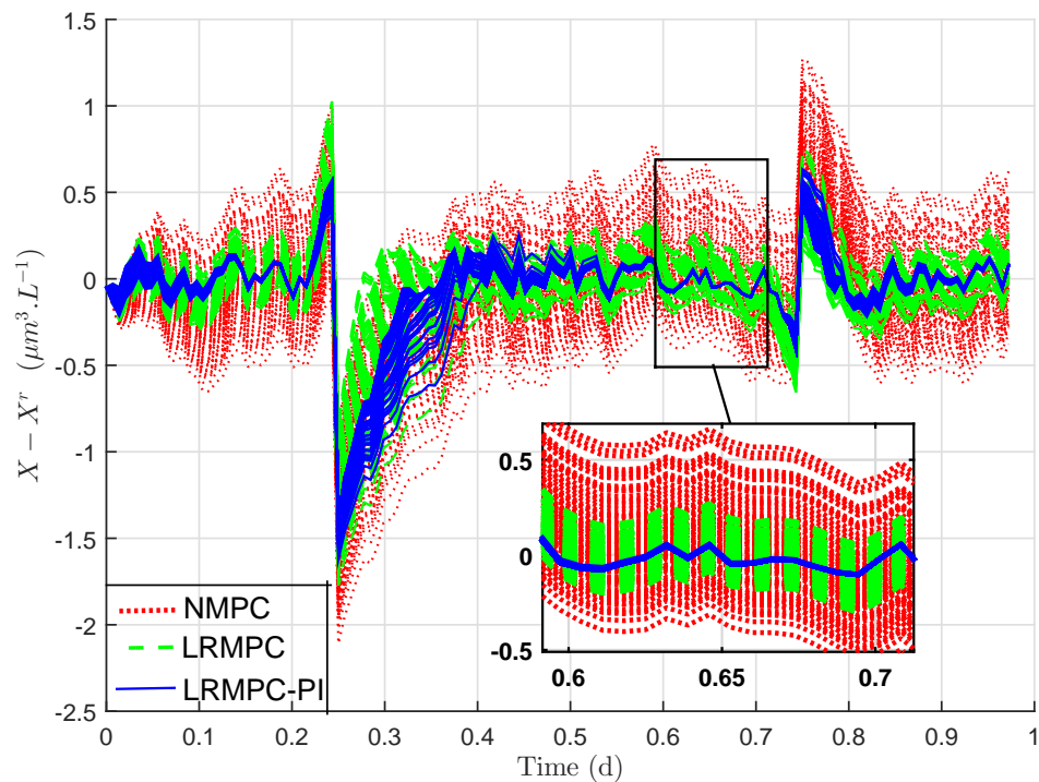
Figure 7.17: Time evolution of tracking error for simultaneous random non correlated variation in all the parameters (Monte-Carlo).
