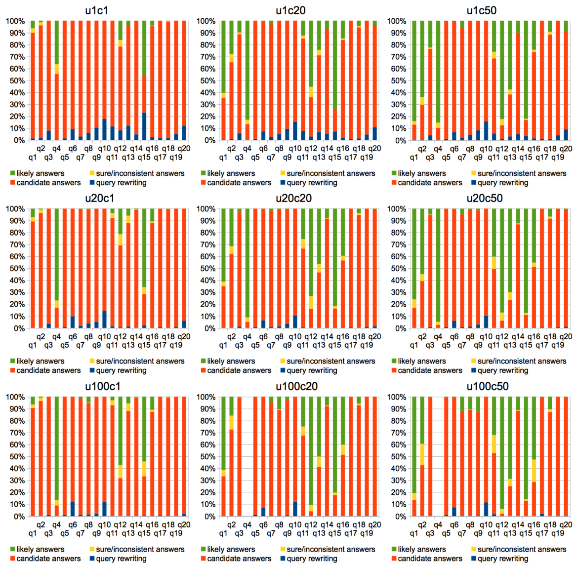
Fig. 3.6 Proportion of time spent by CQAPri in the different phases of query answering on 9 ABoxes: the two lower bars are the time for rewriting the query and executing the rewritten query to get candidate answers, and the two upper bars represent the time needed to classify such answers, by identifying the IAR- and non-brave-answers in a first step, then the AR-answers.
