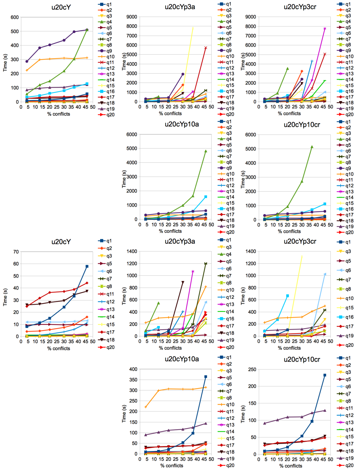
Fig. 6.7 Time in seconds for query answering under \subseteq_P -AR w.r.t. the ratios of conflicts on u20cYpZW (about 2 million assertions), for four prioritizations. For readability, the figures on the bottom focus on the queries whose answering times are lower and whose behaviors are thus not visible on the first one.
