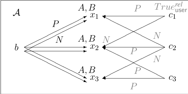
Reduction for coNP-hardness of recognition of globally \preceq_{W,U} -optimal optimal repair plans. Graphical representation of \mathcal{A} \cup True_{user}^{rel} constructed from an example set of clauses \Phi = \{C_1 = x_1 \vee \neg x_2, C_2 = \neg x_1 \vee x_2 \vee \neg x_3\} .
