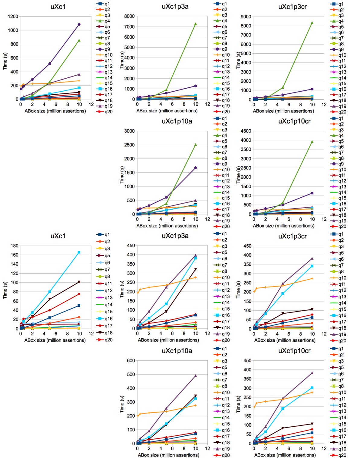
Fig. 6.8 Time in seconds for query answering under \subseteq_P -AR w.r.t. the size of the ABox on uXc1pZW (about 4% of assertions involved in some conflict), for four prioritizations. For readability, the figures on the bottom focus on the queries whose answering times are lower and whose behaviors are thus not visible on the first one.
