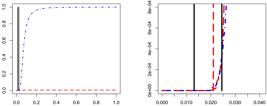
Figure 6.9: Real case study for p = 10^{-5} and d = 4 . Results have been averaged on 24 independent experiments. Left: Representation of the estimation of the cumulative distribution function of g(\mathbf{X}) . Vertical lines represent the bounds obtained by the sequential estimator. Right: Representation of the estimation of the cumulative distribution function around the estimation of q_p . The red dashed line represents the estimation of the quantile obtained from the sequential method.
