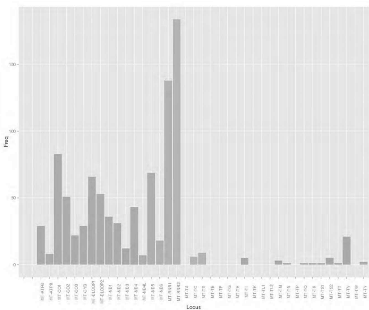
Figure 55: Heteroplasmic sites grouped according their loci on the mitochondrial genome over all samples.
