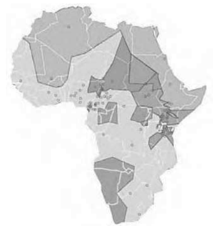
Figure 32: Geographic distributions of six major clusters based on genome-wide SNP diversity within African populations. Each colour represents one of six clusters produced by using a Bayesian clustering analysis assuming no admixture. The yellow cluster corresponds well with the distribution of Niger-Kordofanian languages (Tishkoff et al., 2009).
