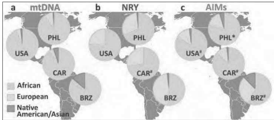
Figure 34: Pan-continental group ancestry of African descendants. MtDNA (a) and NRY (b) reflecting maternal and paternal admixture respectively, while AIMs (c) reflecting the autosomal genome. These genetic systems show the relative ratio of three continental populations that significantly contribute to the admixed populations of the United States (the entire U.S. and by a sample from Philadelphia, PHL), the Caribbean Islands (CAR), and Brazil (BRZ) (Stefflova et al., 2011).
