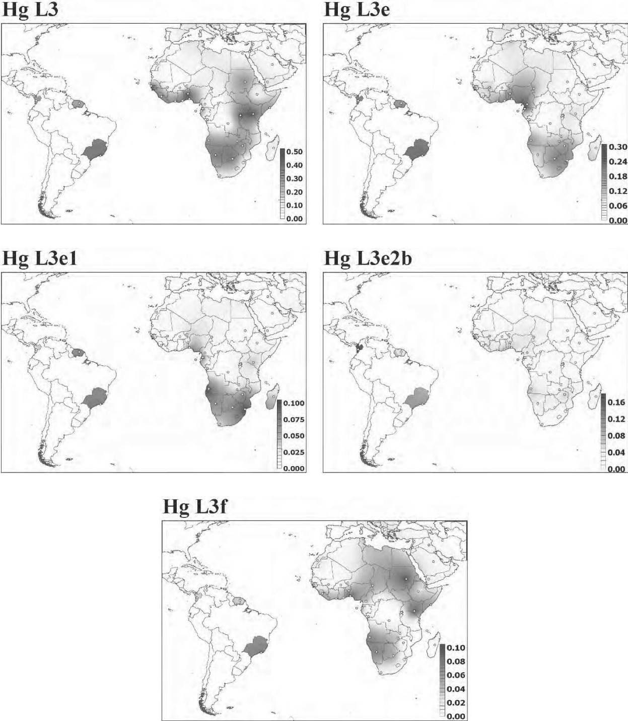
Figure 62: Spatial patterns of the African haplogroup L3 and its subhaplogroups: L3e, L3e1, L3e2b, and L3f, within African, Near Eastern, and African-American populations.
