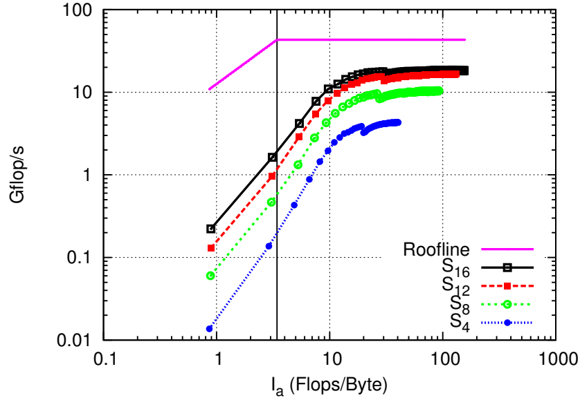
Figure 2.6: Roofline model for an Intel Xeon E52697 V2 processor and measured performances of the sweep operation as a function of the arithmetic intensity I_a . The variation of I_a is obtained by varying size of MacroCells as in Figure 2.4b.
