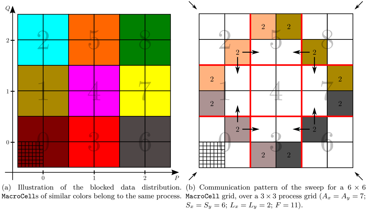
Figure 3.1: 2D blocked data distribution and communication pattern of the simultaneous sweep of all quadrants.
