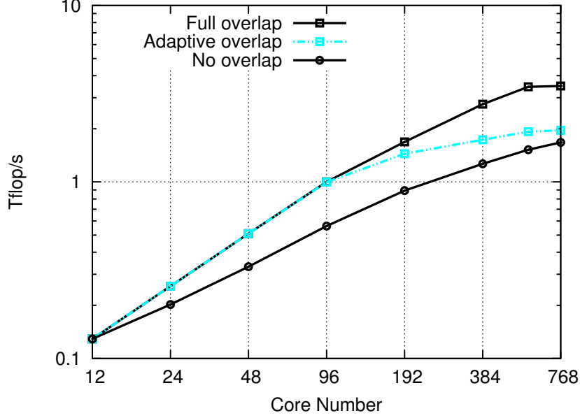
Figure 3.7: Performance of the Hybrid model using the small test case on IVANOE. This figure illustrates how the Hybrid model integrates the overlap of communications by computations.
