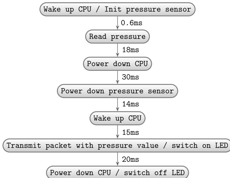
Figure 8.3 – Application layer: a single transmission cycle
