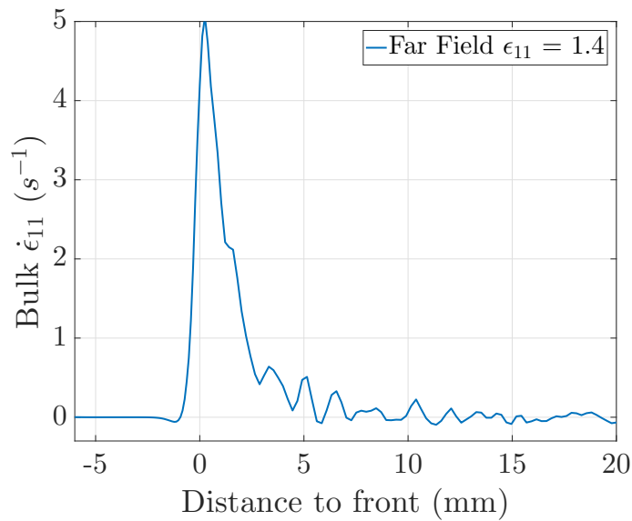
Figure 7.18: The local steady state strain rate in direction 1 along the median axis of symmetry as a function of the distance to the crack tip. The mean strain rate is about 1.5 s^{-1} but the maximal strain rate is about 5 s^{-1} .
