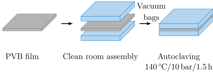
Figure 2.1: Schematic representation of laminated glass assembly at the laboratory scale
