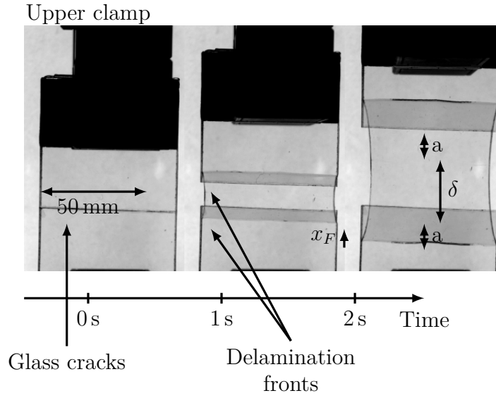
Figure 4.3: A typical TCT experiment at 20^\circ\text{C} and 10\text{ mm s}^{-1} . Sample width is 50\text{ mm} . \delta is the upper clamp/upper glass displacement. a will denote the position of the delamination front relative to the glass edge. x_f will be the distance of a given point to the point at the vertical of the delamination front.
