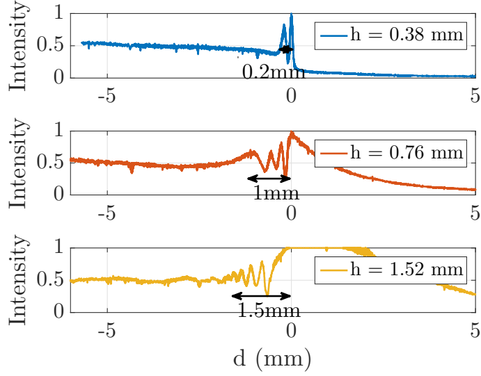
Figure 4.11: Photoelastic measurement conducted close to the delamination front during a TCT experiment at 20^\circ\text{C} and 10\text{ mm s}^{-1} .
