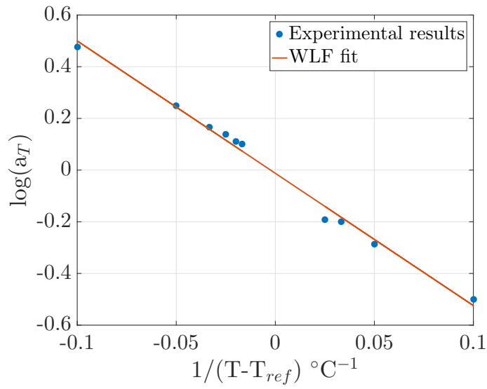
Figure 3.7: DMA shift coefficient at a reference temperature of 40 °C (blue) and WLF law fit with ( C_1 = 19 and C_2 = 143 °C) (red).
