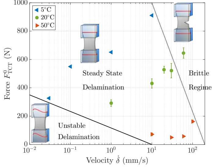
Figure 4.8: The mean steady state delamination force F_{TCT}^0 increases with velocity \dot{\delta} and decreases with temperature. The dark lines arbitrary delimit the three delamination regimes. Measurements were only possible in the intermediate regime where no buckling of the front (low velocities and high temperatures) or brittle nature of the interlayer (high velocities and low temperatures) are observed.
