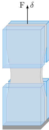
Figure 1.9: Schematic representation of the Through Crack Tensile Test sample. The delaminated part of the interlayer is stretched in between the delamination fronts.
