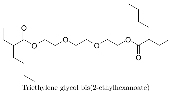
Figure 3.2: Plasticizer molecule.
