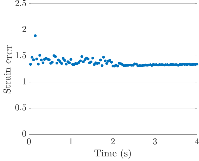
Figure 4.6: In this 20^{\circ}\text{C} and 10\text{ mm s}^{-1} TCT Test, the nominal strain \epsilon_{\text{TCT}} reaches a steady state plateau which mean value is \epsilon_{\text{TCT}}^0 = 1.4 and that is related to the symmetric delamination of the fronts at a constant velocity.
