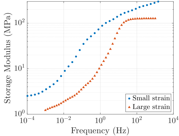
Figure 3.15: Prony series using the characteristic times and moduli found in the relaxation experiment at large strain and in the small strain DMA/Rheometer tests. The reference temperature is 20 °C in both cases. It illustrates the difference induced by the large strain on the time/temperature superimposition.
