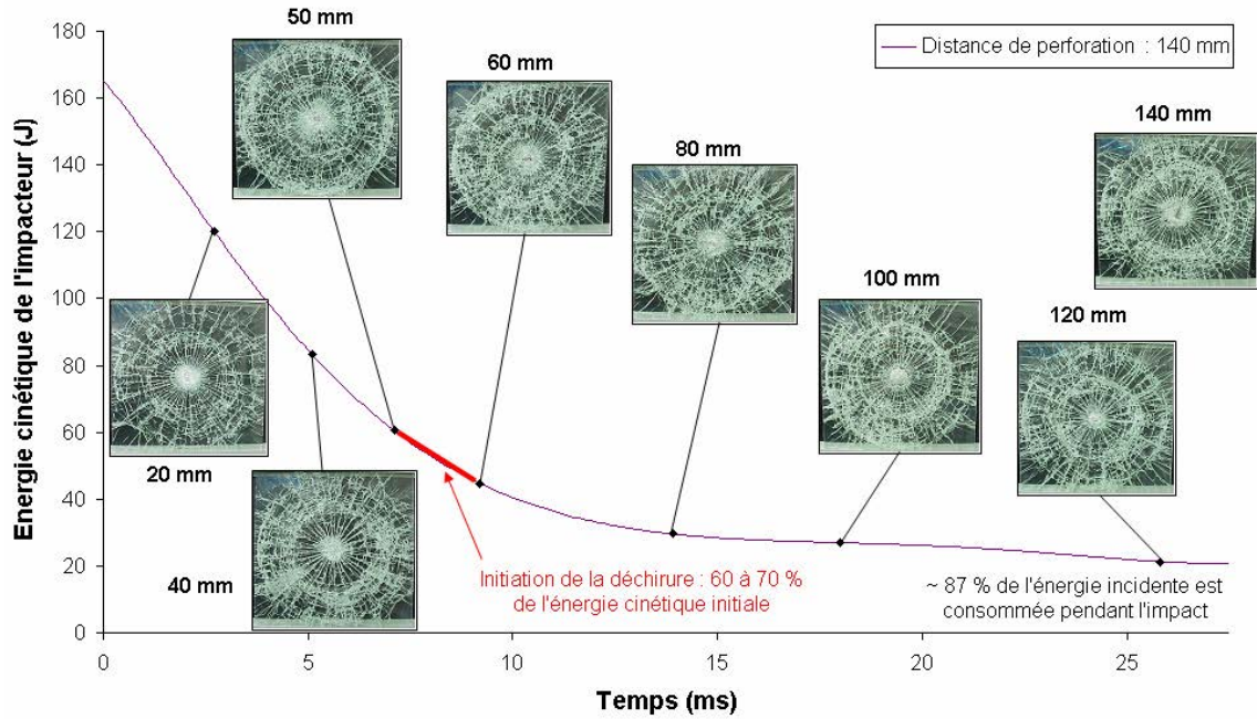
Figure 1.7: The kinetic energy of the impacting object is plotted as a function of time and perforation length. This test is conducted at 20^{\circ}\text{C} and the impacting object has a velocity of 9.2\text{ m s}^{-1} (Results from Nourry's PhD thesis [8]).
