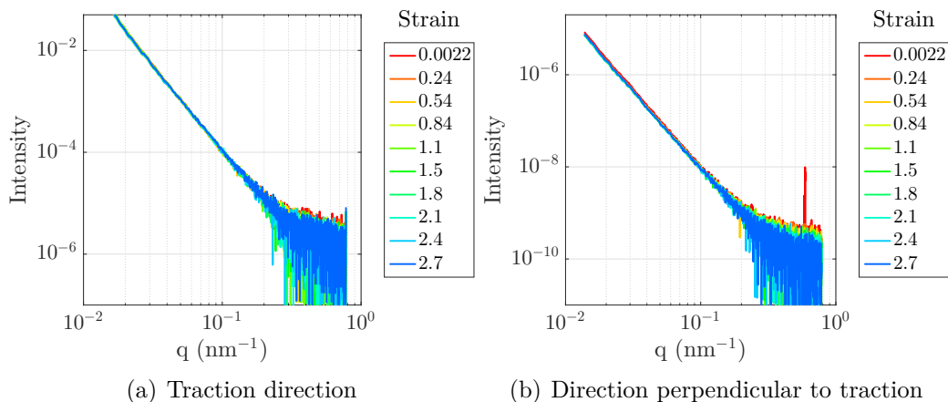
Figure 3.27: SAXS experiment at 70 °C during a uniaxial tension experiment.
