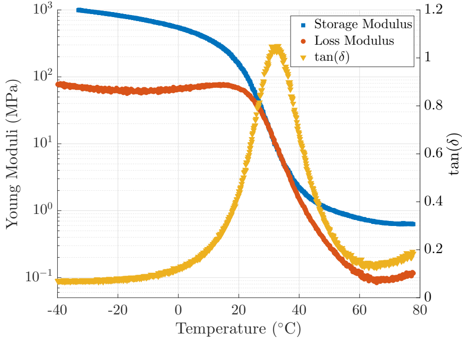
Figure 3.5: DMA experiment on PVB at 1 Hz and 0.01% deformation for temperature ranging from -40^{\circ}\text{C} to 80^{\circ}\text{C} .
