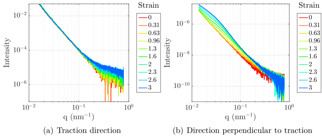
Figure 3.26: SAXS experiment at 23^{\circ}\text{C} during a uniaxial tension experiment.
