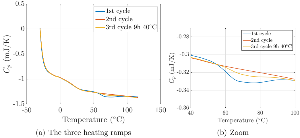
Figure 3.25: Three DSC cycles at 20^{\circ}\text{C min}^{-1} . First cycle shows an exothermic - fusion like signal around 70^{\circ}\text{C} . The second cycle after a fast cooling at 20^{\circ}\text{C min}^{-1} do not display this signal. Finally the third cycle done after 9 h at 40^{\circ}\text{C} presents a partial recovery of the signal.
