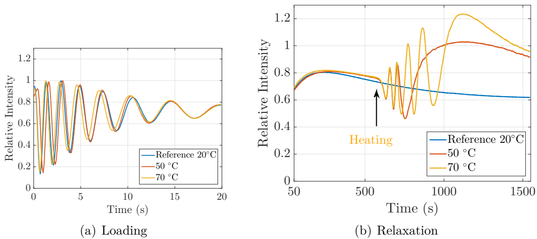
Figure 3.24: Relaxation experiment while heating. A reference at 20 °C is displayed. Two temperatures were tested 50 °C and 70 °C. Loading rate was 0.1 \text{ s}^{-1} (a). Relaxation lasts 1000s. Heating start at 500s after the end of the loading.
