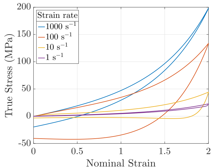
Figure 7.9: Calculated traction curve for our model polymer with \mu = 10\text{ MPa} , \lambda_m = 2 and one relaxation time \tau_1 = 0.01\text{ s} and \alpha_1 = 0.9 . The calculation was made for four different strain rates from 1\text{ s}^{-1} to 1000\text{ s}^{-1} . These results can be compared with experimental curves in Figure 3.12.
