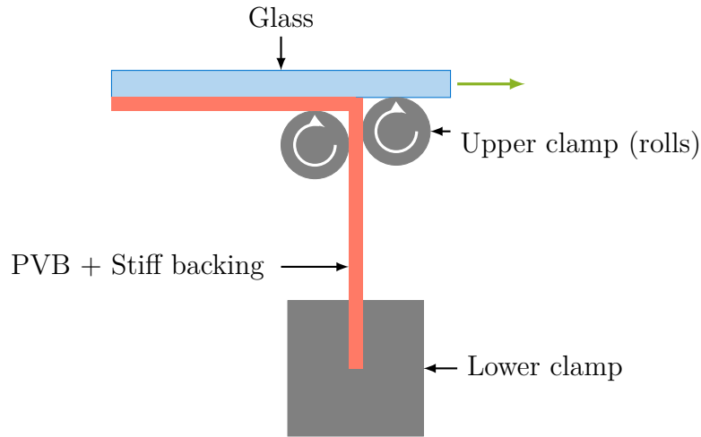
Figure 2.7: Schematic view of the peel setup. Two rolls enable the peel angle to be kept constant through the test equal to 90^\circ [13].
