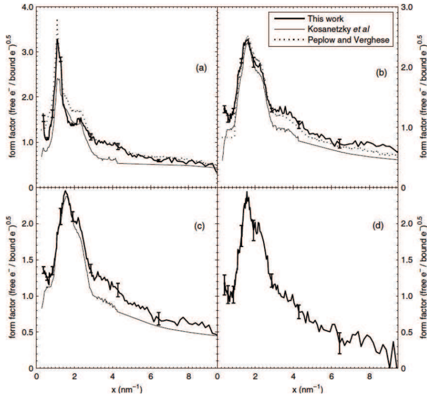
Figure I.31: Measured form factors of (a) fat, (b) muscle, (c) liver and (d) kidney. Comparison of the results obtained by [King et al. , 2011] to the ones found by [Peplow and Verghese, 1998] and [Kosanetzky et al. , 1987]. (Image taken from [King et al. , 2011].)
