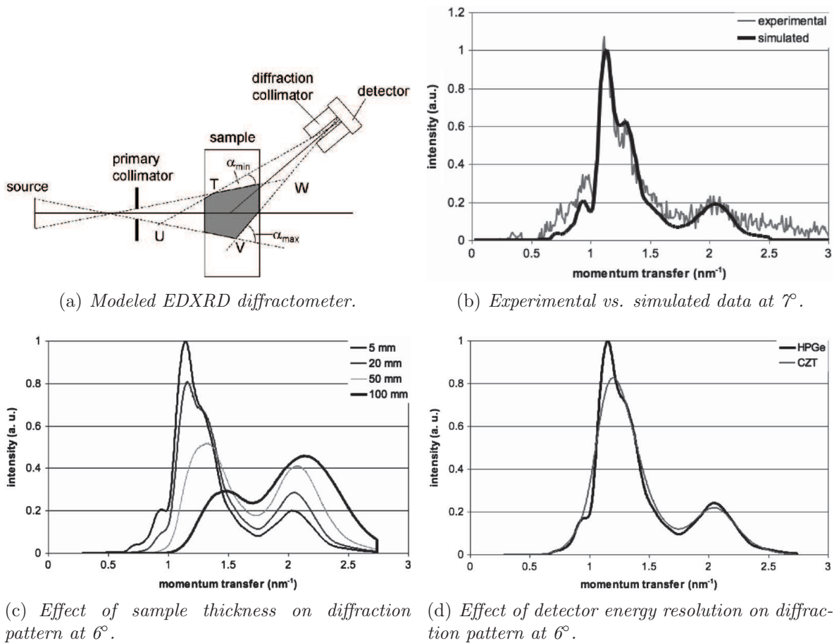
Figure I.68: Modeled EDXRD diffractometer and simulated Zircate spectra with different parameters [Pani et al. , 2009].
