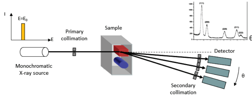
Figure I.19: Schematic view of an angular dispersive X-ray diffraction (ADXRD) system: Constant energy E (monochromatic source) and different diffraction angles \theta .
