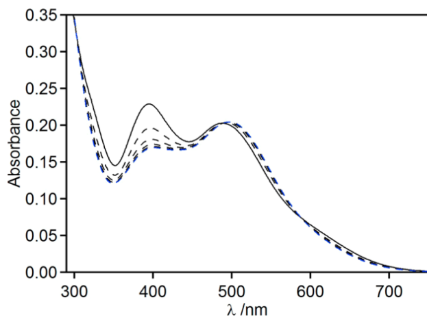
Figure 9. Absorption spectrum of ruthenium complex ( E )- 14 in MeCN ( C = 30 \mu\text{M} ) at 25 °C (black solid line) and its stepwise evolution upon 5 s irradiation pulses at 406 nm with P = 9 \text{ mW cm}^{-2} (black dashed lines). The blue dashed line corresponds to the PSS.
