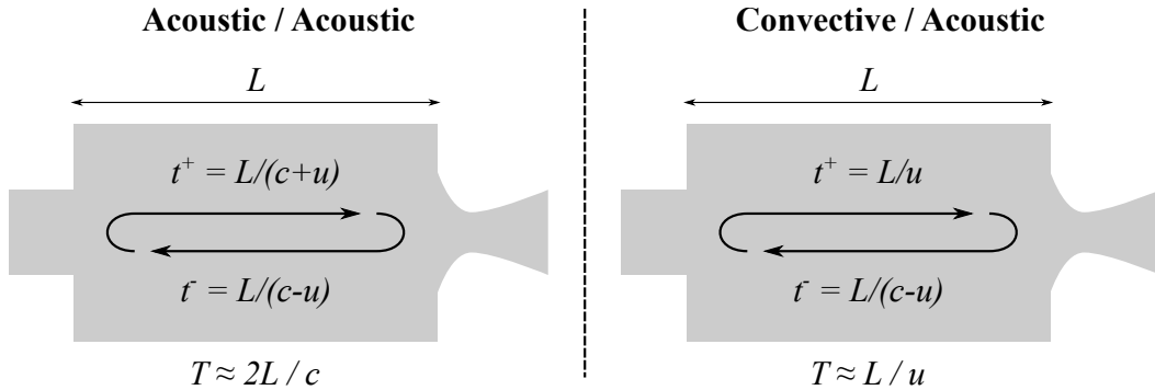
Figure 11.15: Simplified representation of an acoustic/acoustic loop (left), associated with a round-trip time of T \approx 2L/c , and a convective/acoustic loop (right), where T \approx L/u . Note that these values arise from a low Mach number approximation, i.e. u \ll c .
