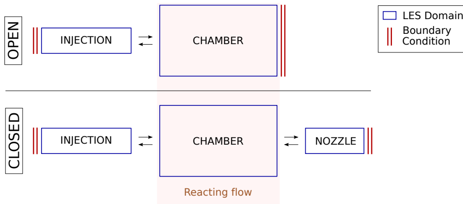
Figure 4.2: OPEN versus CLOSED domains for LES. Top: OPEN with no nozzle. The chamber sees LES input at its inlet but its outlet is a plane upstream of the nozzle. Bottom: CLOSED domain with (part of) the nozzle included. The inlet is unchanged, but the nozzle belongs to the LES domain, and the boundary condition is located further downstream.
