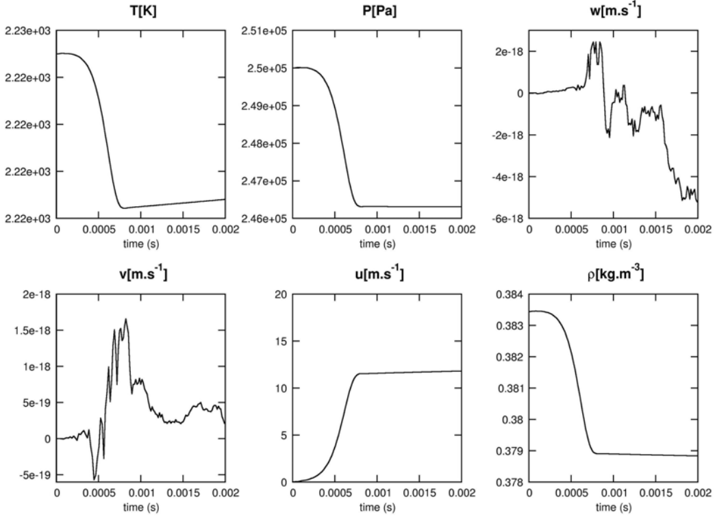
Figure 8.4: xl tool on a node at the center of the inlet patch.
