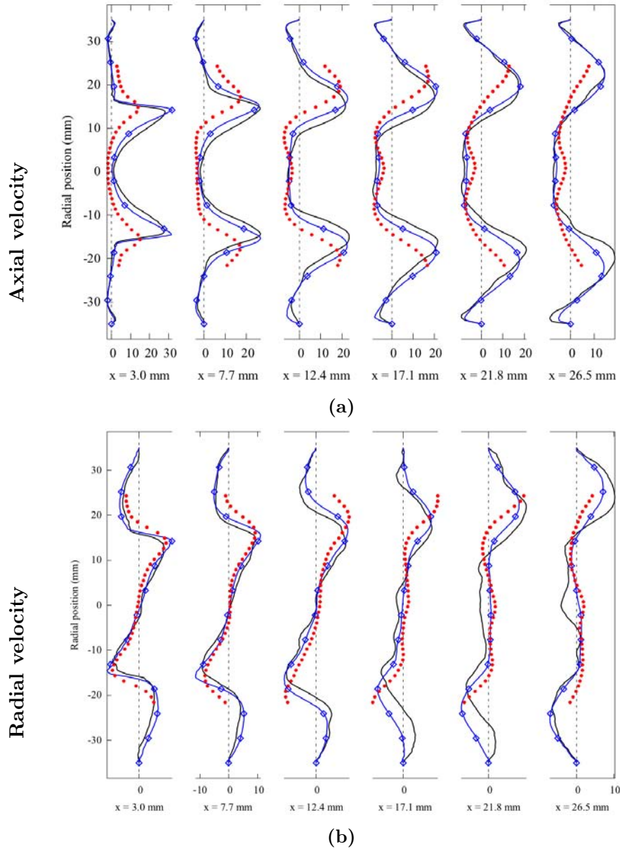
Figure 10.5: Mean velocity profiles (in \text{ms}^{-1} ) along 6 the lines of Fig. 10.4. (a) axial velocity, and (b) radial velocity. Red dots: PIV, blue lines with diamonds: LES with the wrong geometry, Black lines: LES with the correct geometry.
