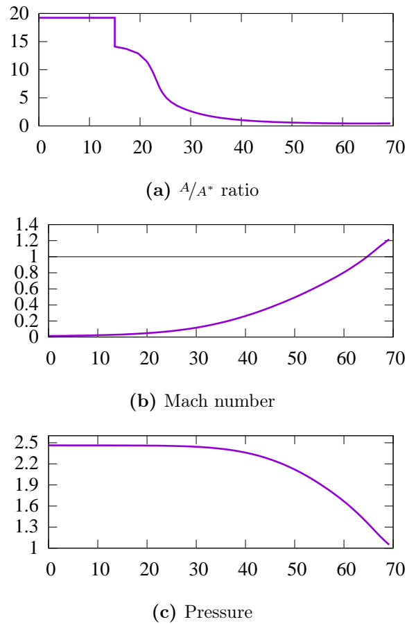
Figure 8.8: A/A^* ratio (a), Mach number (b) and pressure (c) profiles along the nozzle axis for the 18 \text{ g s}^{-1} reference case.
