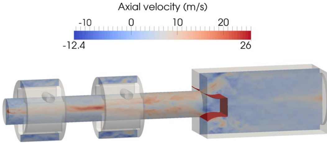
Figure 10.7: Initial field for reacting open simulations. Red surface is 1000 K isoline. Colored plane represents axial velocity.
