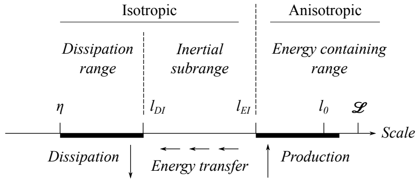
Figure 7.1: Schematic representation of the turbulent energy cascade, versus motion scales. From ( Pope, 2000 , chap. 6), who notes l_{DI} the demarcation line between Dissipation (D) and Inertial (I) ranges, and l_{EI} the one between Energy (E) and Inertial (I) ranges.
