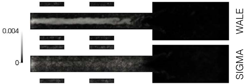
Figure 9.5: Turbulent viscosity (in \text{kg s}^{-1} \text{m}^{-1} ). Comparison between the WALE (top) and SIGMA (bottom) SGS models.
