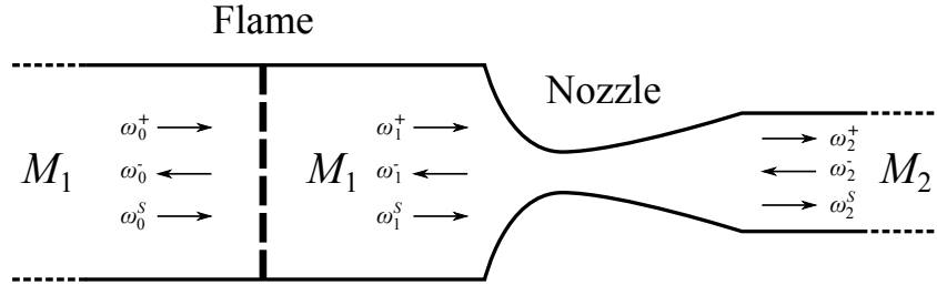
Figure 5.7: Notations for the toy model of Leyko (2010) .
