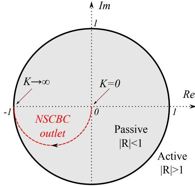
Figure 4.3: Reflection coefficient R_{out} of an NSCBC outlet in the complex plane, according to calculations of Selle et al. (2004a) . R_{out} follows the red dotted arc circle as the relax coefficient K of the outlet changes. For K = 0 , the condition is non reflective. If K > 0 , the reflection coefficient is located in the complex plane, somewhere along the arc. The exact position depends on both the value of K and on the frequency f . In the limit of K \rightarrow \infty , the boundary condition becomes fully reflective for all frequencies and R = 1 .
