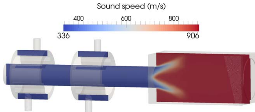
Figure 11.12: Distribution of the sound speed used for the AVSP computation.
