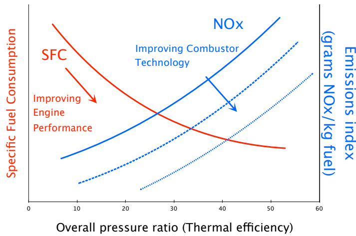
Figure 1.2: Specific fuel consumption and \text{NO}_x emissions versus overall pressure ratio for present aircraft engine technologies. Reproduced from Suder (2012) .
