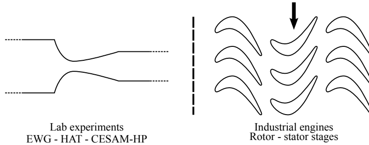
Figure 5.4: Simplified lab experiment dilatation systems (generally a simple nozzle) differ from realistic rotor stator stages of industrial turbines.
