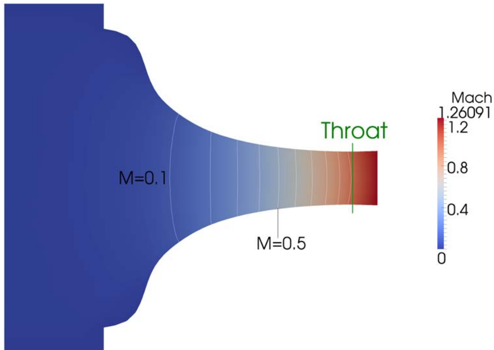
Figure 8.6: Mach number field in a cross subsectional cut along the axis of the nozzle, for \dot{m} = 18 g/s. White lines are Mach number isolines from 0.1 to 1.0 with a step of 0.1.
