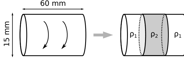
Figure 6.7: Initialization strategy for the FPAVA test case. A cold field at T = 300 K of density \rho_1 is put in rotation with a constant azimuthal source term (SP flow). Then, the middle third of the domain is modified: pressure is kept constant, but temperature is set to T = 2200 K, inducing a decrease of density according to the equation of state to \rho_2 . The right-hand side field is the initial field for the FPAVA test case.
