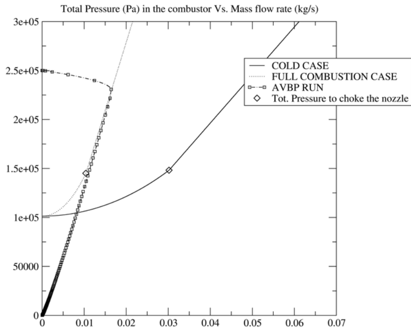
Figure 8.11: XNozzle tool applied to run 0 (no inlet).
