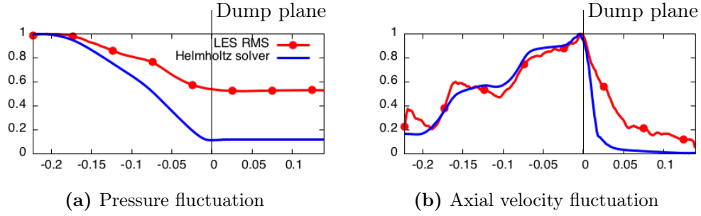
Figure 11.13: Comparison along the setup centerline between the RMS activity in the CHOKED-ST LES (red line with dots) and the acoustic mode found with the Helmholtz solver (blue solid line).
