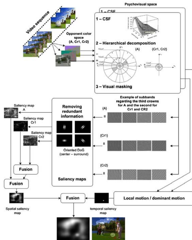
Figure 2.3: Architecture of the spatio-temporal model of visual attention by Le Meur et al. [144]
