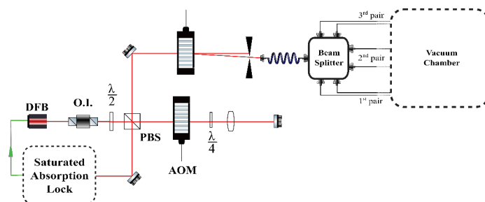
Figure 3.3 – Schematic optical setup of the re-pumping beams. Two AOMs are used in this setup. The upper AOM switches on and off (single pass configuration), and the bottom one is being used to scan the frequency of the laser without misaligning the beam (double pass configuration). Green line indicates the feedback lock signal.
