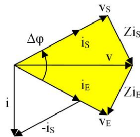
Figure 3-12: Diagramme de Fresnel idéal
