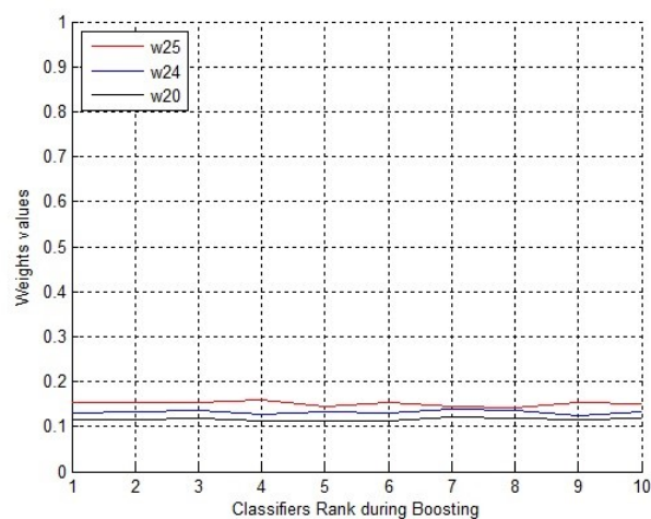
Fig. 5.10 Variation of values affected to the best three weights ( w_{25} , w_{24} , w_{20} ) with the inclusion order of their corresponding weak classifiers: case of HGPP algorithm upon the IRIS – M 3 database
