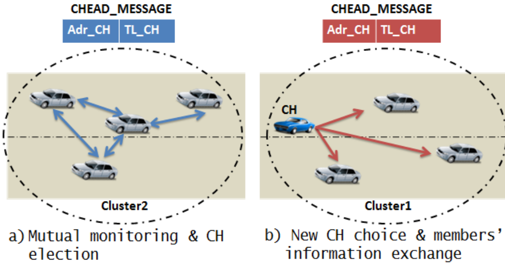
Figure 4.7 – Cluster-head election and maintenance in IPDS
