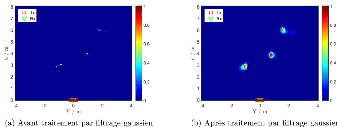
Fig. III.21 – Cartographie nettoyée, C_1 = (-1, 3)m , C_2 = (1, 4)m et C_3 = (1.8, 6)m , PRF=40MHz
