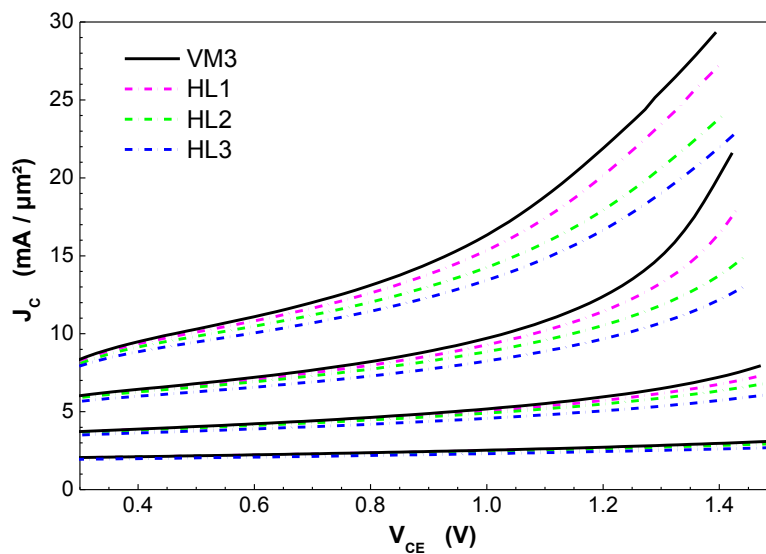
Figure 4.4 : Comparison of the collector current density J_C for the test structures HL; test structure VM3 is used as a reference. The V_{BE} is swept from 0.825V to 0.9V.
