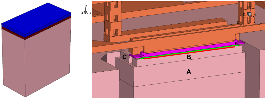
Figure 3.26: (left) the structure simulated in Sentaurus TCAD environment: silicon is represented in pink, \text{SiO}_2 in brown, copper in orange and the air layer is colored in blue. (right) zoom in the active part of the transistor: polysilicon is colored in magenta, SiGe in green and the heat source is highlighted in red, whereas \text{SiO}_2 is hidden for better visibility; the buried layer is indicated with the letter A, the selectively implanted collector (SIC) with B and the collector sinker with C.
