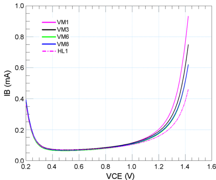
Figure 4.7: comparison of the I_B of the different transistors for V_{BE}=0.875V ; for clarity in this plot just 5 different test structures are compared. Refer to Table 4.2 for a complete comparison.
