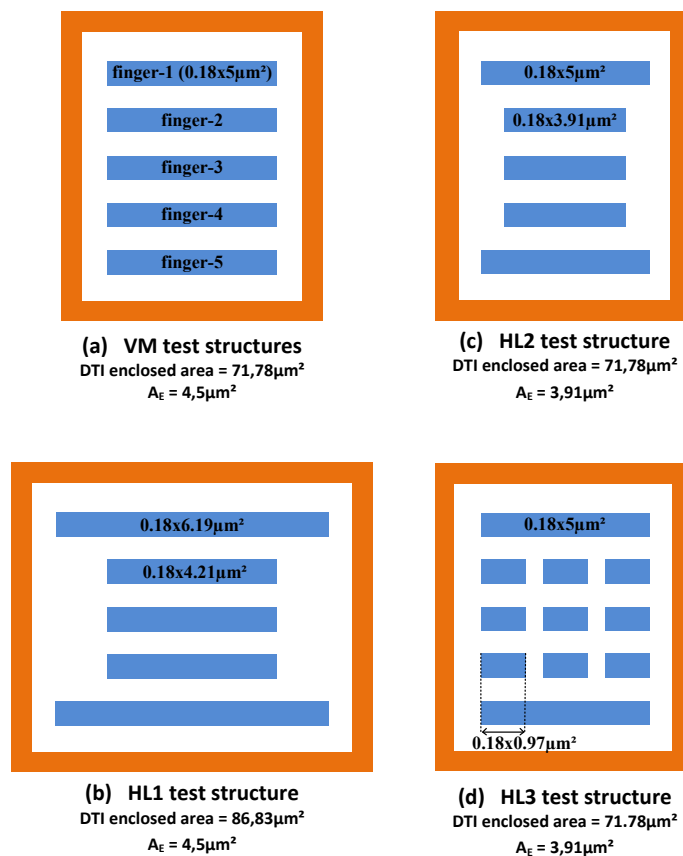
Figure 4.2: Finger layout of the test structures (the dimensions reported refer to the drawn emitter window). The DTI is depicted in orange, whereas the 5 drawn emitter windows are colored in blue.
