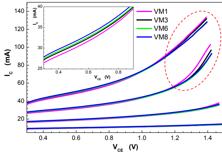
Figure 4.3 : Comparison of the output characteristics of the transistors VM. The V_{BE} is swept from 0.825V to 0.9V. The dotted circle highlights the region where power dissipation is more significant. The subplot shows a zoom-in in the medium V_{CE} range for V_{BE}=0.875V to show the impact of the mechanical stress.
