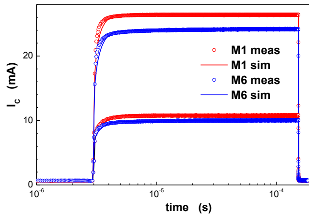
Figure 3.21: Measured and simulated I_C versus time for V_{CE}=1.5V ; on-voltages of the pulse signal V_{BE} are 0.9V and 0.95V ; x axis is in log scale to better evidence the evolution of I_C versus time.
