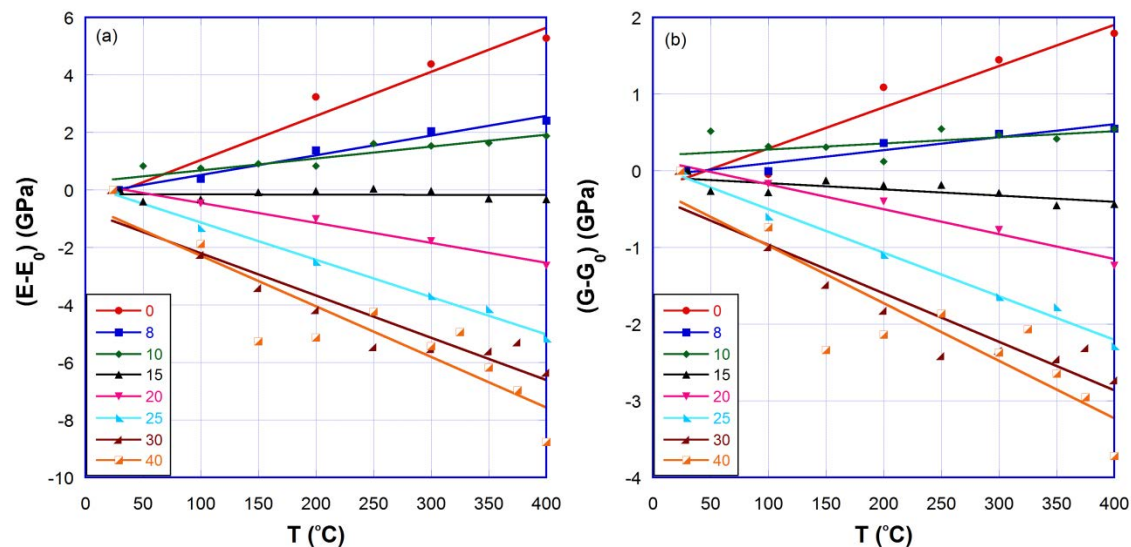
Fig. 2-5. Normalized temperature dependence of Young's modulus ( E ) (a) and shear modulus ( G ) (b) for sodium silicate glasses. E_0 and G_0 are the room temperature values. Sodium silicate glasses switch from anomalous to normal behavior with increasing sodium content, with intermediate behavior occurring around 15% \text{Na}_2\text{O} [19].
