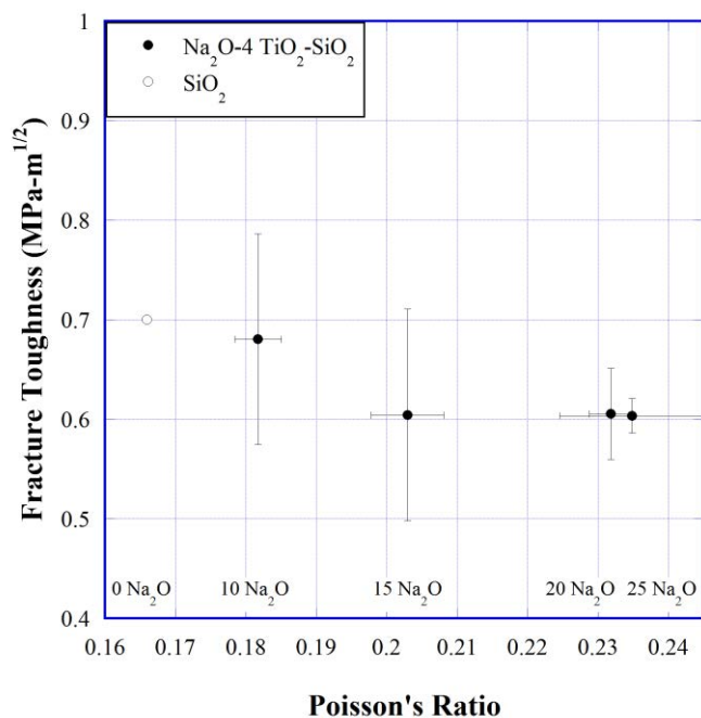
Fig. 6-5. Fracture toughness versus Poisson's ratio. Fracture toughness was measured using the SEPB method on \text{Na}_2\text{O-TiO}_2\text{-SiO}_2 glasses with 4 mol% \text{TiO}_2 . Error bars represent the standard deviation across two to four measurements. \text{SiO}_2 fracture toughness was taken from literature [10,11].
